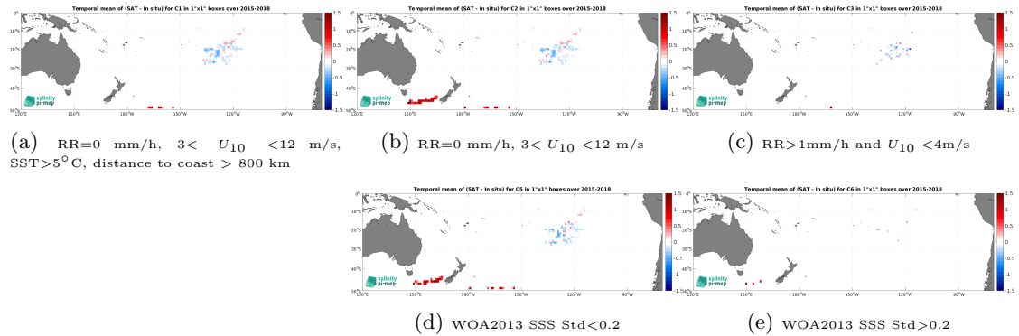
Figure 13: Temporal mean gridded over spatial boxes of size 1^\circ \times 1^\circ of \Delta SSS (SMAP SSS L3 v5.0 - 8-Day running (JPL) - Surface drifters) for 5 different subdatasets corresponding to:RR=0 mm/h, 3 < U_{10} < 12 m/s, SST > 5^\circ\text{C} , distance to coast > 800 km (a), RR=0 mm/h, 3 < U_{10} < 12 m/s (b), RR > 1 mm/h and U_{10} < 4 m/s (c), WOA2013 SSS Std < 0.2 (d), WOA2013 SSS Std > 0.2 (e).
