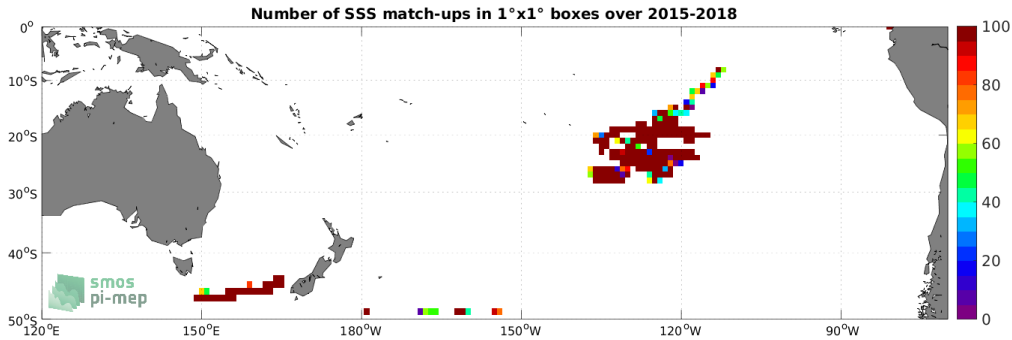
Figure 3: Number of SSS match-ups between Surface drifters SSS and the SMAP SSS L3 v5.0 - 8-Day running (JPL) SSS product for the South Pacific Ocean Pi-MEP region over 1^\circ \times 1^\circ boxes and for the full satellite product period.
