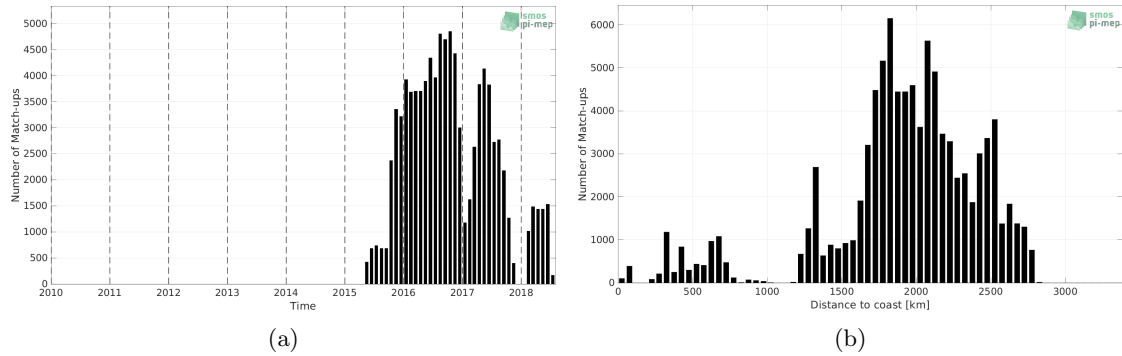
Figure 1: Number of match-ups between Surface drifters and SMAP SSS L3 v5.0 - 8-Day running (JPL) SSS as a function of time (a) and as function of the distance to coast (b) over the South Pacific Ocean Pi-MEP region and for the full satellite product period.
