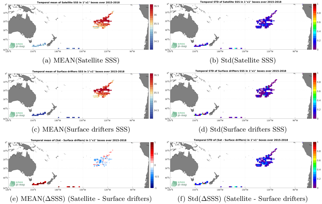
Figure 5: Temporal mean (left) and Std (right) of SSS from SMAP SSS L3 v5.0 - 8-Day running (JPL) (top), Surface drifters (middle), and of \Delta SSS (Satellite - Surface drifters). Only match-up pairs are used to generate these maps.
