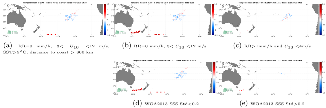
Figure 11: Temporal mean gridded over spatial boxes of size 1^\circ \times 1^\circ of \Delta SSS (SMAP SSS L3 v5.0 - 8-Day running (JPL) - Surface drifters) for 5 different subdatasets corresponding to:RR=0 mm/h, 3 < U_{10} < 12 m/s, SST >5^\circ C, distance to coast > 800 km (a), RR=0 mm/h, 3 < U_{10} < 12 m/s (b), RR >1 mm/h and U_{10} < 4 m/s (c), WOA2013 SSS Std <0.2 (d), WOA2013 SSS Std >0.2 (e).
