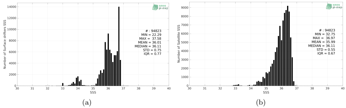
Figure 2: Histograms of SSS from Surface drifters (a) and SMAP SSS L3 v5.0 - 8-Day running (JPL) (b) considering all match-up pairs per bins of 0.1 over the South Pacific Ocean Pi-MEP region and for the full satellite product period.
