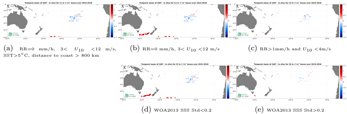
Figure 11: Temporal mean gridded over spatial boxes of size 1^\circ \times 1^\circ of \Delta\text{SSS} (SMAP SSS L3 v5.0 - 8-Day running (JPL) - Surface drifters) for 5 different subdatasets corresponding to:RR=0 mm/h, 3 < U_{10} < 12 m/s, SST >5^\circ\text{C} , distance to coast > 800 km (a), RR=0 mm/h, 3 < U_{10} < 12 m/s (b), RR >1 mm/h and U_{10} < 4 m/s (c), WOA2013 SSS Std <0.2 (d), WOA2013 SSS Std >0.2 (e).
