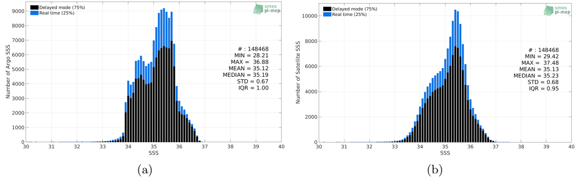
Figure 2: Histograms of SSS from Argo (a) and SMAP SSS L3 v5.0 - 8-Day running (JPL) (b) considering all match-up pairs per bins of 0.1 over the South Pacific Ocean Pi-MEP region and for the full satellite product period.
