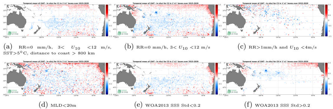
Figure 12: Temporal mean gridded over spatial boxes of size 1°x1° of \Delta SSS (SMAP SSS L3 v5.0 - 8-Day running (JPL) - Argo) for 6 different subdatasets corresponding to:RR=0 mm/h, 3 < U_{10} < 12 m/s, SST>5°C, distance to coast > 800 km (a), RR=0 mm/h, 3 < U_{10} < 12 m/s (b), RR>1mm/h and U_{10} < 4 m/s (c),MLD<20m (d),WOA2013 SSS Std<0.2 (e),WOA2013 SSS Std>0.2 (f).
