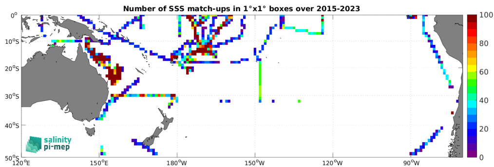
Figure 5: Number of SSS match-ups between TSG (SAMOS) SSS and the SMAP SSS L3 v5.0 - Monthly (JPL) SSS product for the South Pacific Ocean Pi-MEP region over 1^\circ \times 1^\circ boxes and for the full satellite product period.
