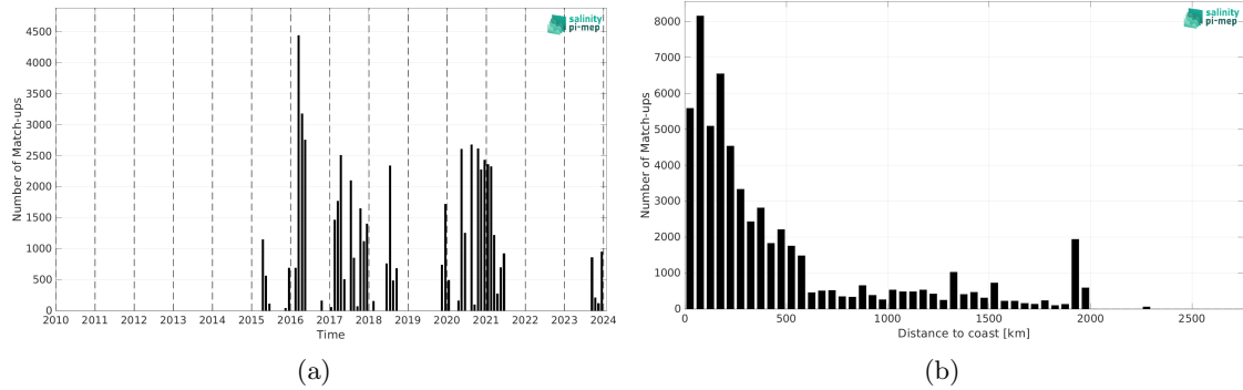
Figure 2: Number of match-ups between TSG (SAMOS) and SMAP SSS L3 v5.0 - Monthly (JPL) SSS as a function of time (a) and as function of the distance to coast (b) over the South Pacific Ocean Pi-MEP region and for the full satellite product period.
