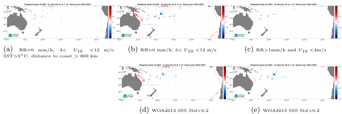
Figure 14: Temporal mean gridded over spatial boxes of size 1^\circ \times 1^\circ of \Delta\text{SSS} (SMAP SSS L3 v5.0 - Monthly (JPL) - TSG (SAMOS)) for 5 different subdatasets corresponding to:RR=0 mm/h, 3 < U_{10} < 12 m/s, SST>5°C, distance to coast > 800 km (a), RR=0 mm/h, 3 < U_{10} < 12 m/s (b), RR>1mm/h and U_{10} < 4 m/s (c), WOA2013 SSS Std<0.2 (d), WOA2013 SSS Std>0.2 (e).
