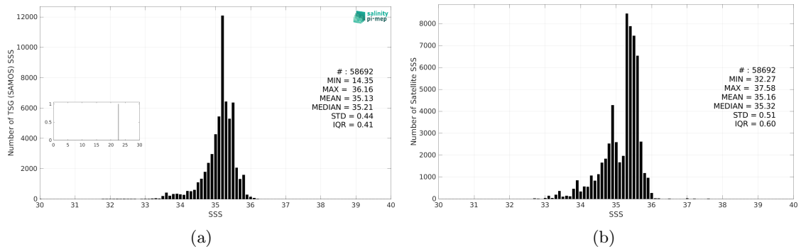
Figure 3: Histograms of SSS from TSG (SAMOS) (a) and SMAP SSS L3 v5.0 - Monthly (JPL) (b) considering all match-up pairs per bins of 0.1 over the South Pacific Ocean Pi-MEP region and for the full satellite product period.
