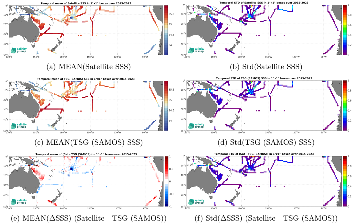
Figure 7: Temporal mean (left) and Std (right) of SSS from SMAP SSS L3 v5.0 - Monthly (JPL) (top), TSG (SAMOS) (middle), and of \Delta SSS (Satellite - TSG (SAMOS)). Only match-up pairs are used to generate these maps.
