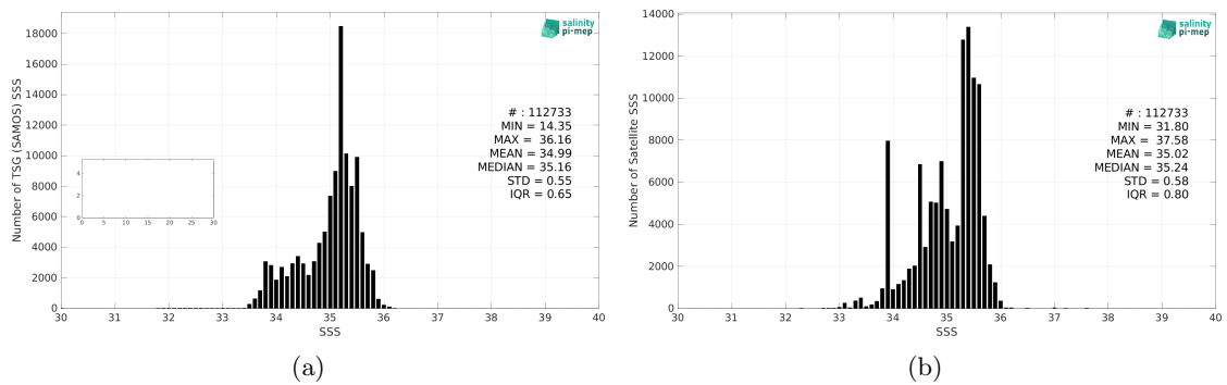
Figure 2: Histograms of SSS from TSG (SAMOS) (a) and SMAP SSS L3 v5.0 - Monthly (JPL) (b) considering all match-up pairs per bins of 0.1 over the South Pacific Ocean Pi-MEP region and for the full satellite product period.
