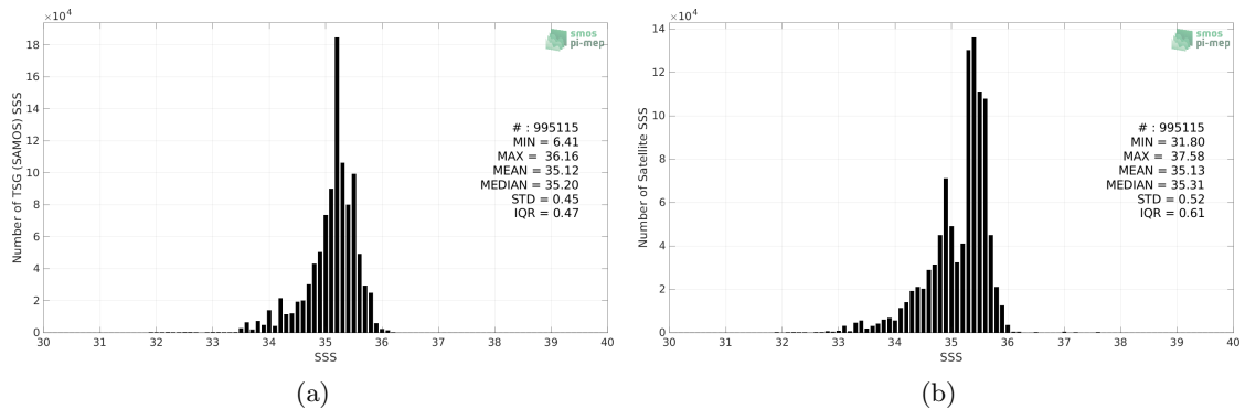
Figure 2: Histograms of SSS from TSG (SAMOS) (a) and SMAP SSS L3 v5.0 - Monthly (JPL) (b) considering all match-up pairs per bins of 0.1 over the South Pacific Ocean Pi-MEP region and for the full satellite product period.
