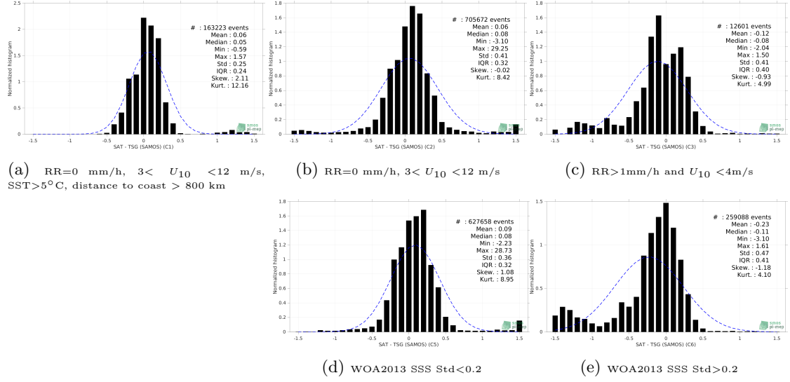
Figure 13: Normalized histogram of \Delta SSS (SMAP SSS L3 v5.0 - Monthly (JPL) - TSG (SAMOS)) for 5 different subdatasets corresponding to: RR=0 mm/h, 3 < U_{10} < 12 m/s, SST>5°C, distance to coast > 800 km (a), RR=0 mm/h, 3 < U_{10} < 12 m/s (b), RR>1mm/h and U_{10} < 4 m/s (c), WOA2013 SSS Std<0.2 (d), WOA2013 SSS Std>0.2 (e).
