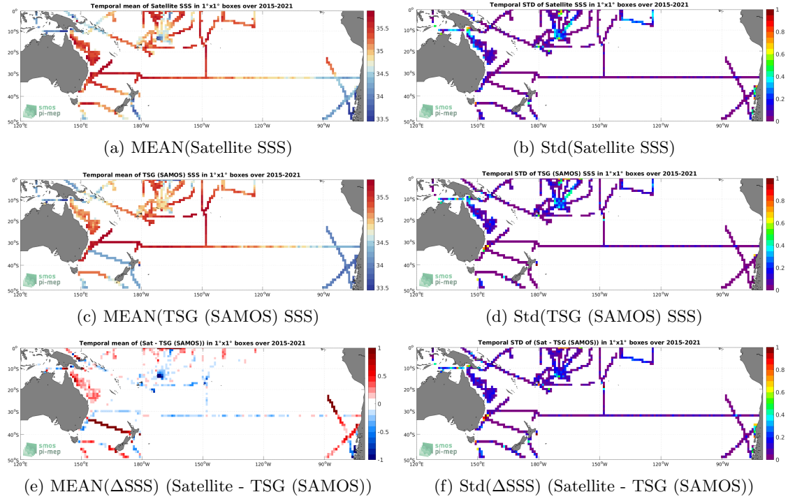
Figure 6: Temporal mean (left) and Std (right) of SSS from SMAP SSS L3 v5.0 - Monthly (JPL) (top), TSG (SAMOS) (middle), and of \Delta SSS (Satellite - TSG (SAMOS)). Only match-up pairs are used to generate these maps.
