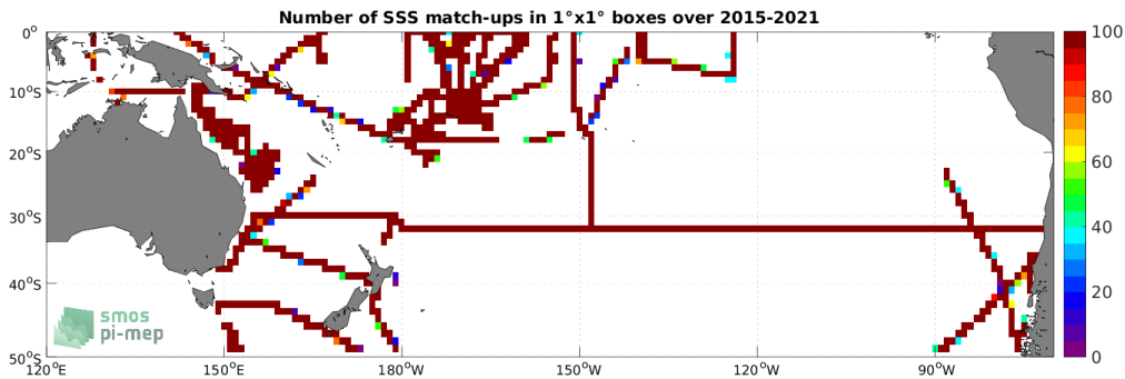
Figure 4: Number of SSS match-ups between TSG (SAMOS) SSS and the SMAP SSS L3 v5.0 - Monthly (JPL) SSS product for the South Pacific Ocean Pi-MEP region over 1^\circ \times 1^\circ boxes and for the full satellite product period.
