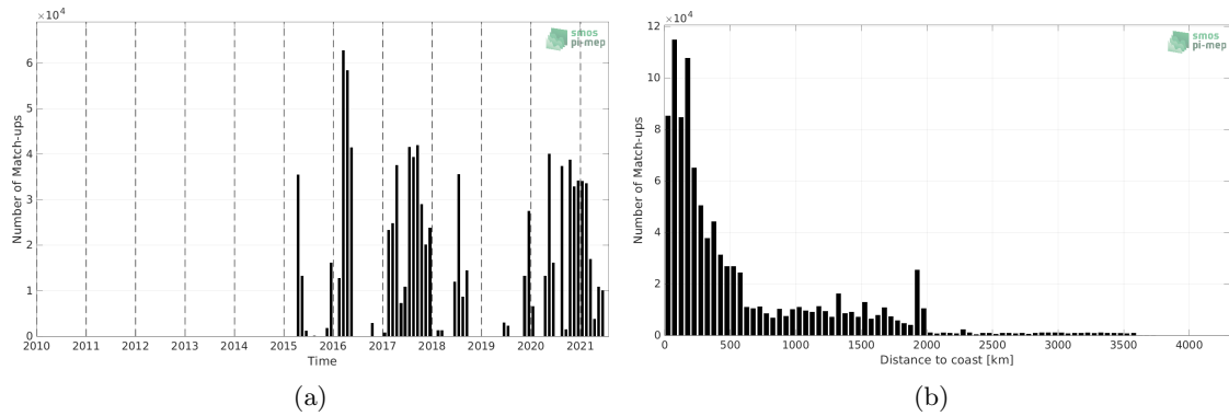
Figure 1: Number of match-ups between TSG (SAMOS) and SMAP SSS L3 v5.0 - Monthly (JPL) SSS as a function of time (a) and as function of the distance to coast (b) over the South Pacific Ocean Pi-MEP region and for the full satellite product period.
