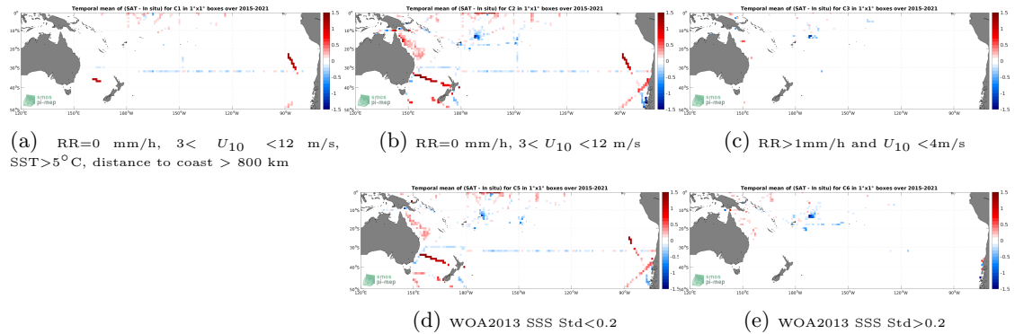
Figure 12: Temporal mean gridded over spatial boxes of size 1^\circ \times 1^\circ of \Delta SSS (SMAP SSS L3 v5.0 - Monthly (JPL) - TSG (SAMOS)) for 5 different subdatasets corresponding to:RR=0 mm/h, 3 < U_{10} < 12 m/s, SST >5^\circ\text{C} , distance to coast > 800 km (a), RR=0 mm/h, 3 < U_{10} < 12 m/s (b), RR >1 mm/h and U_{10} < 4 m/s (c), WOA2013 SSS Std <0.2 (d), WOA2013 SSS Std >0.2 (e).
