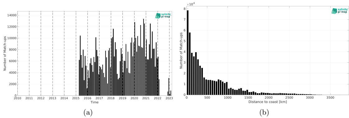
Figure 2: Number of match-ups between TSG (LEGOS-DM) and SMAP SSS L3 v5.0 - Monthly (JPL) SSS as a function of time (a) and as function of the distance to coast (b) over the South Pacific Ocean Pi-MEP region and for the full satellite product period.
