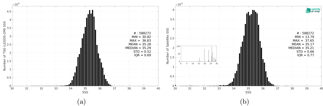
Figure 3: Histograms of SSS from TSG (LEGOS-DM) (a) and SMAP SSS L3 v5.0 - Monthly (JPL) (b) considering all match-up pairs per bins of 0.1 over the South Pacific Ocean Pi-MEP region and for the full satellite product period.
