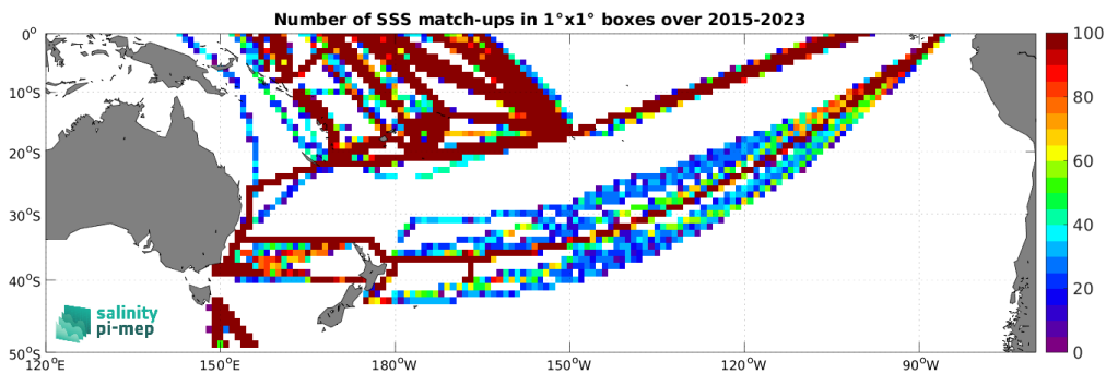
Figure 5: Number of SSS match-ups between TSG (LEGOS-DM) SSS and the SMAP SSS L3 v5.0 - Monthly (JPL) SSS product for the South Pacific Ocean Pi-MEP region over 1^\circ \times 1^\circ boxes and for the full satellite product period.
