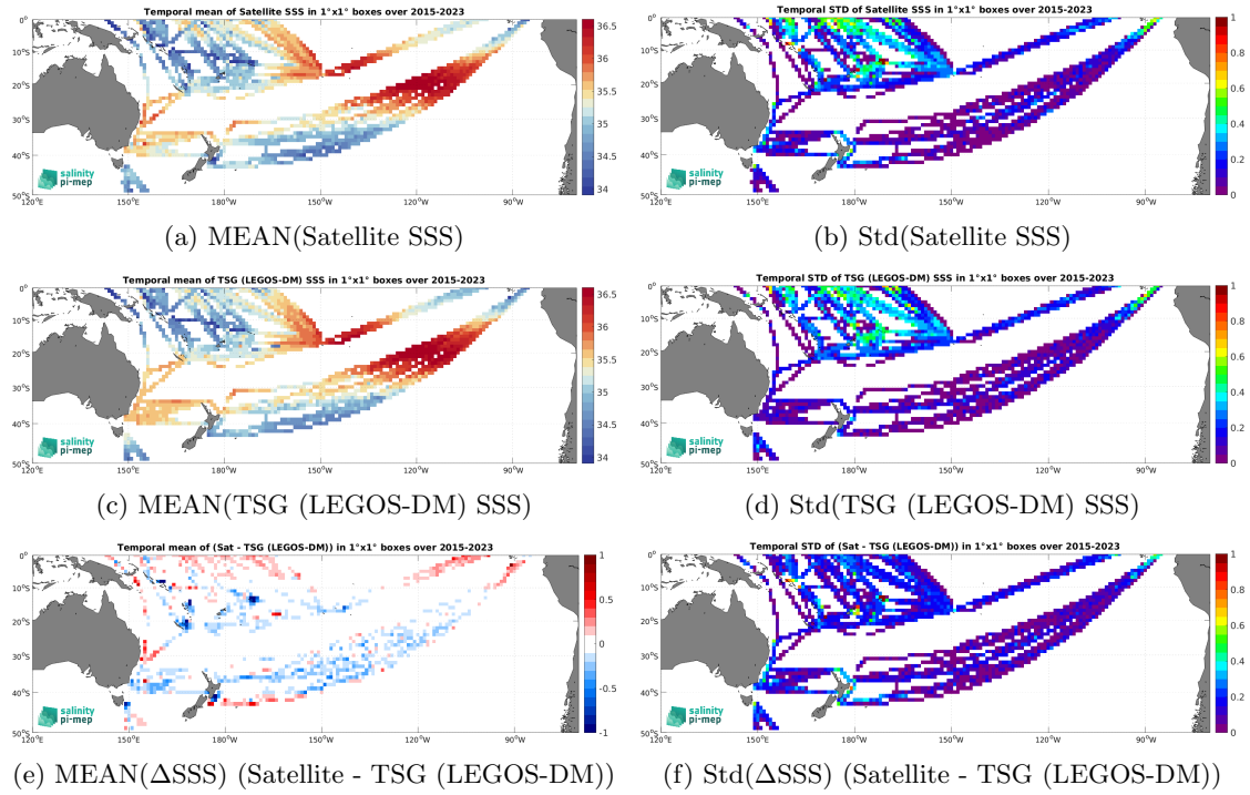
Figure 7: Temporal mean (left) and Std (right) of SSS from SMAP SSS L3 v5.0 - Monthly (JPL) (top), TSG (LEGOS-DM) (middle), and of \Delta SSS (Satellite - TSG (LEGOS-DM)). Only match-up pairs are used to generate these maps.
