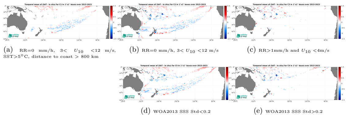
Figure 14: Temporal mean gridded over spatial boxes of size 1^\circ \times 1^\circ of \Delta SSS (SMAP SSS L3 v5.0 - Monthly (JPL) - TSG (LEGOS-DM)) for 5 different subdatasets corresponding to:RR=0 mm/h, 3 < U_{10} < 12 m/s, SST>5°C, distance to coast > 800 km (a), RR=0 mm/h, 3 < U_{10} < 12 m/s (b), RR>1mm/h and U_{10} < 4 m/s (c), WOA2013 SSS Std<0.2 (d), WOA2013 SSS Std>0.2 (e).
