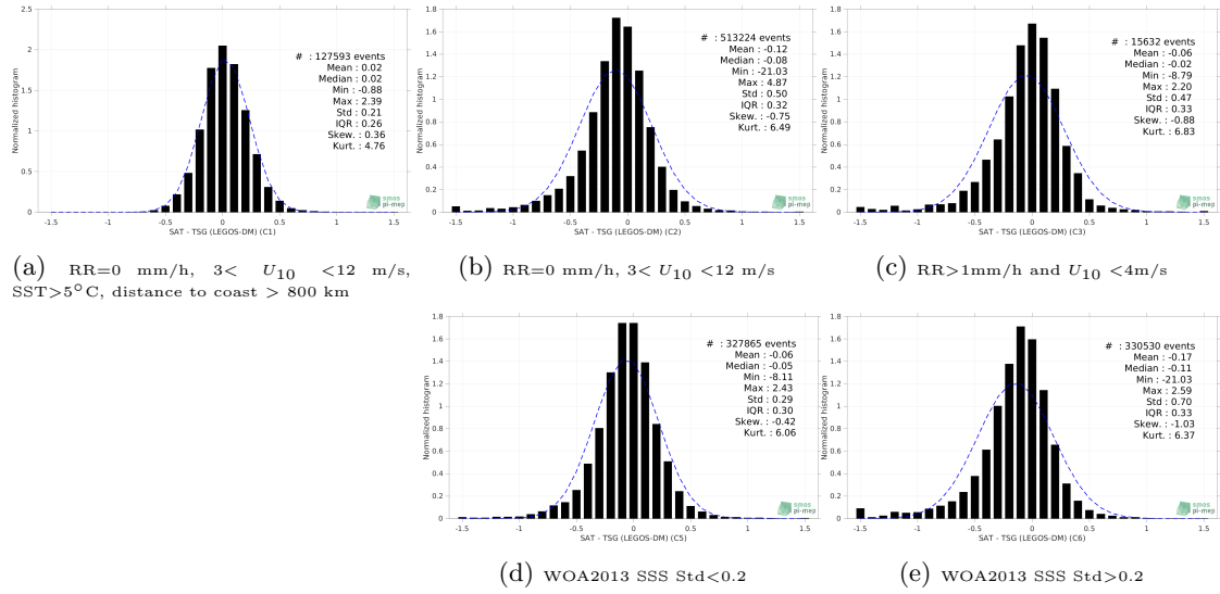
Figure 13: Normalized histogram of \Delta\text{SSS} (SMAP SSS L3 v5.0 - Monthly (JPL) - TSG (LEGOS-DM)) for 5 different subdatasets corresponding to: RR=0 mm/h, 3 < U_{10} < 12 m/s, SST>5°C, distance to coast > 800 km (a), RR=0 mm/h, 3 < U_{10} < 12 m/s (b), RR>1mm/h and U_{10} < 4 m/s (c), WOA2013 SSS Std<0.2 (d), WOA2013 SSS Std>0.2 (e).
