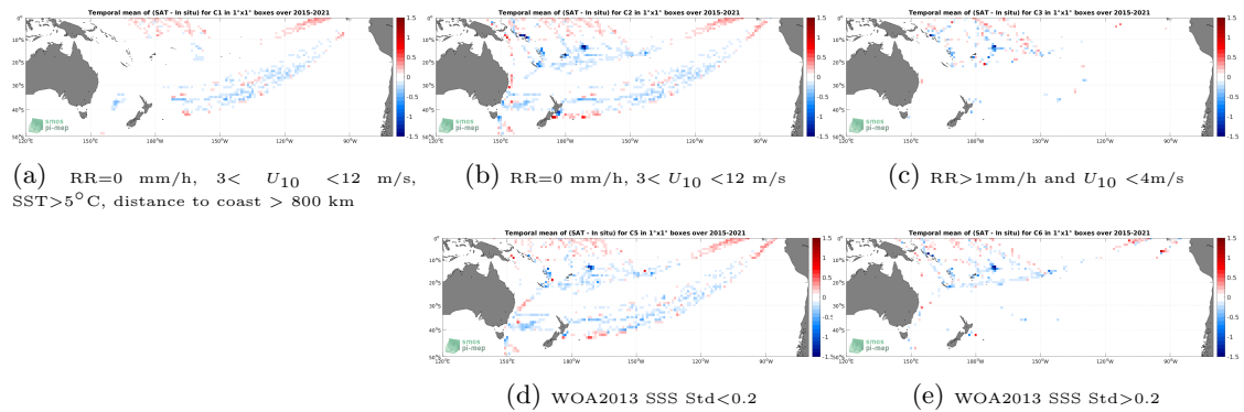
Figure 12: Temporal mean gridded over spatial boxes of size 1^\circ \times 1^\circ of \Delta SSS (SMAP SSS L3 v5.0 - Monthly (JPL) - TSG (LEGOS-DM)) for 5 different subdatasets corresponding to:RR=0 mm/h, 3 < U_{10} < 12 m/s, SST >5^\circ\text{C} , distance to coast > 800 km (a), RR=0 mm/h, 3 < U_{10} < 12 m/s (b), RR >1 mm/h and U_{10} < 4 m/s (c), WOA2013 SSS Std <0.2 (d), WOA2013 SSS Std >0.2 (e).
