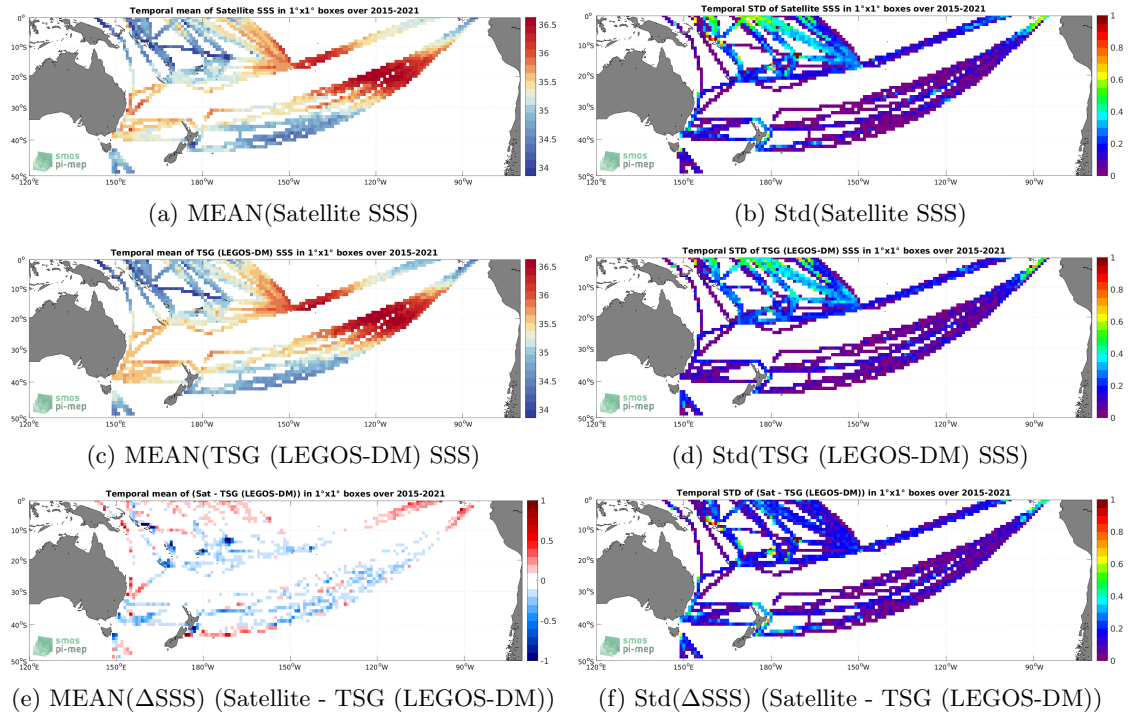
Figure 6: Temporal mean (left) and Std (right) of SSS from SMAP SSS L3 v5.0 - Monthly (JPL) (top), TSG (LEGOS-DM) (middle), and of \Delta SSS (Satellite - TSG (LEGOS-DM)). Only match-up pairs are used to generate these maps.
