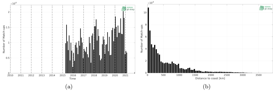
Figure 1: Number of match-ups between TSG (LEGOS-DM) and SMAP SSS L3 v5.0 - Monthly (JPL) SSS as a function of time (a) and as function of the distance to coast (b) over the South Pacific Ocean Pi-MEP region and for the full satellite product period.
