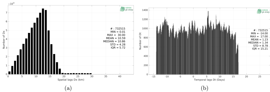
Figure 5: Histograms of the spatial (a) and temporal (b) lags between the location/time of the TSG (LEGOS-DM) measurement and the date of the corresponding SMAP SSS L3 v5.0 - Monthly (JPL) SSS pixel.
