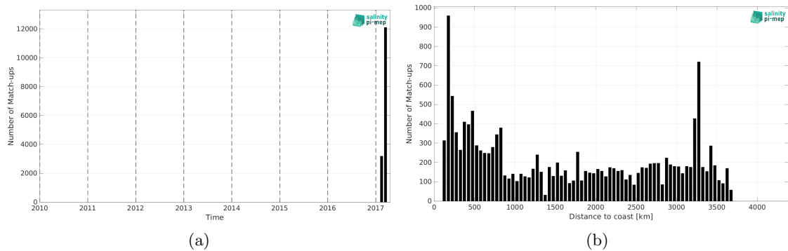
Figure 2: Number of match-ups between TSG (GOSUD-Sailing-ship) and SMAP SSS L3 v5.0 - Monthly (JPL) SSS as a function of time (a) and as function of the distance to coast (b) over the South Pacific Ocean Pi-MEP region and for the full satellite product period.
