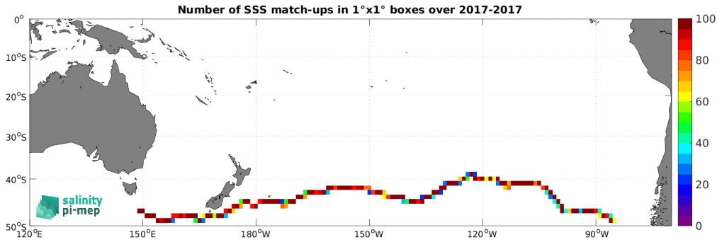
Figure 5: Number of SSS match-ups between TSG (GOSUD-Sailing-ship) SSS and the SMAP SSS L3 v5.0 - Monthly (JPL) SSS product for the South Pacific Ocean Pi-MEP region over 1^\circ \times 1^\circ boxes and for the full satellite product period.
