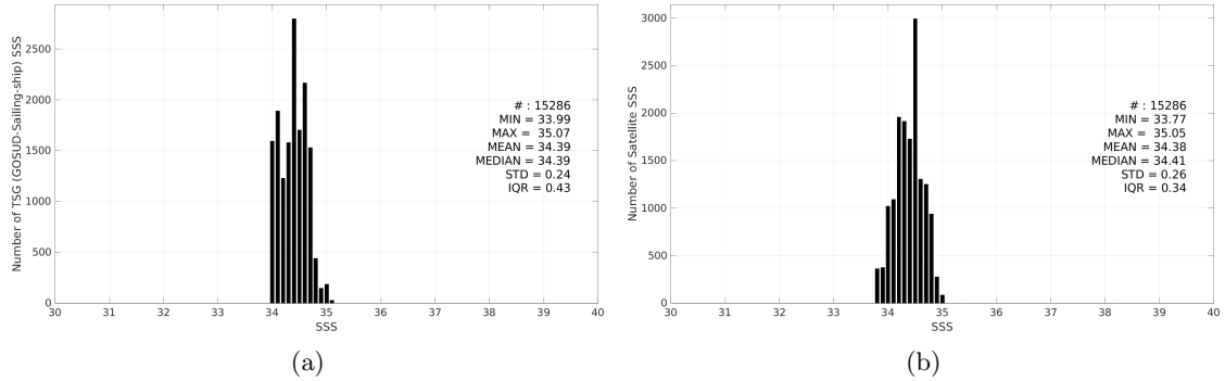
Figure 3: Histograms of SSS from TSG (GOSUD-Sailing-ship) (a) and SMAP SSS L3 v5.0 - Monthly (JPL) (b) considering all match-up pairs per bins of 0.1 over the South Pacific Ocean Pi-MEP region and for the full satellite product period.
