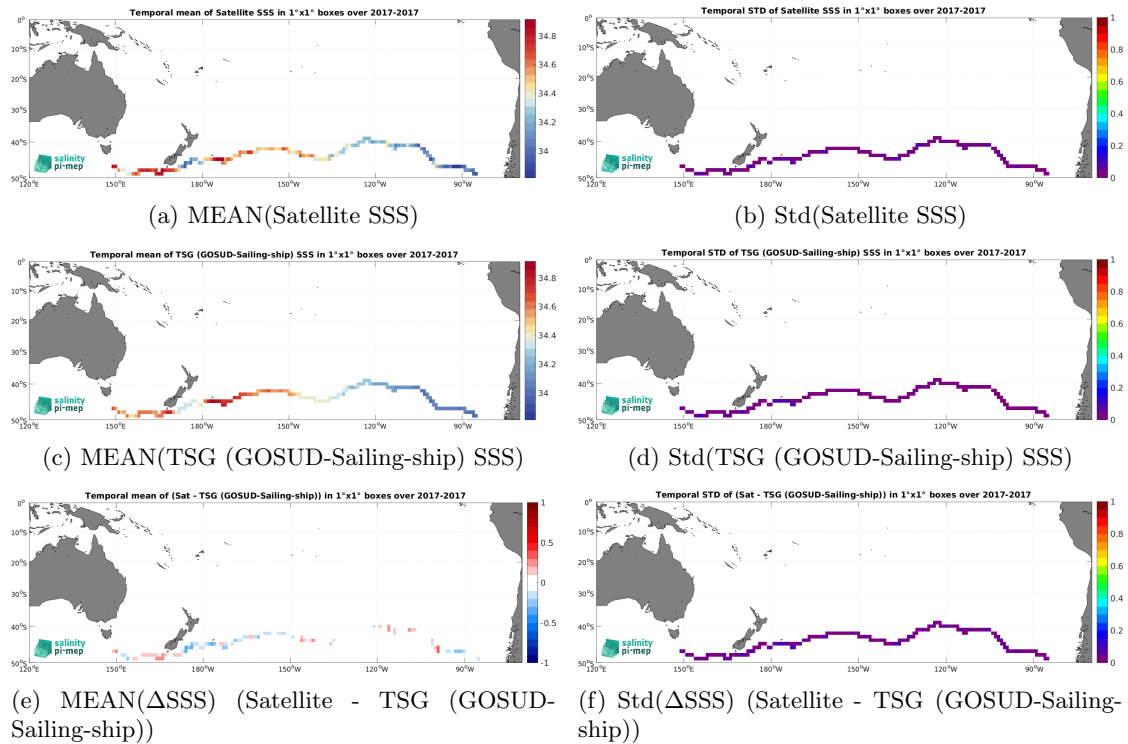
Figure 7: Temporal mean (left) and Std (right) of SSS from SMAP SSS L3 v5.0 - Monthly (JPL) (top), TSG (GOSUD-Sailing-ship) (middle), and of \Delta SSS (Satellite - TSG (GOSUD-Sailing-ship)). Only match-up pairs are used to generate these maps.
