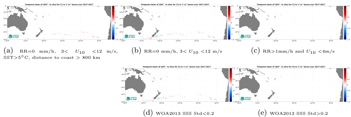
Figure 14: Temporal mean gridded over spatial boxes of size 1^\circ \times 1^\circ of \Delta SSS (SMAP SSS L3 v5.0 - Monthly (JPL) - TSG (GOSUD-Sailing-ship)) for 5 different subdatasets corresponding to:RR=0 mm/h, 3 < U_{10} < 12 m/s, SST >5^\circ\text{C} , distance to coast > 800 km (a), RR=0 mm/h, 3 < U_{10} < 12 m/s (b), RR >1 mm/h and U_{10} < 4 m/s (c), WOA2013 SSS Std <0.2 (d), WOA2013 SSS Std >0.2 (e).
