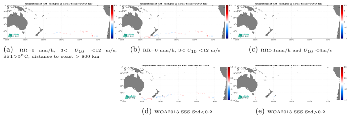
Figure 12: Temporal mean gridded over spatial boxes of size 1^\circ \times 1^\circ of \Delta\text{SSS} (SMAP SSS L3 v5.0 - Monthly (JPL) - TSG (GOSUD-Sailing-ship)) for 5 different subdatasets corresponding to:RR=0 mm/h, 3 < U_{10} < 12 m/s, SST>5°C, distance to coast > 800 km (a), RR=0 mm/h, 3 < U_{10} < 12 m/s (b), RR>1mm/h and U_{10} < 4 m/s (c), WOA2013 SSS Std<0.2 (d), WOA2013 SSS Std>0.2 (e).
