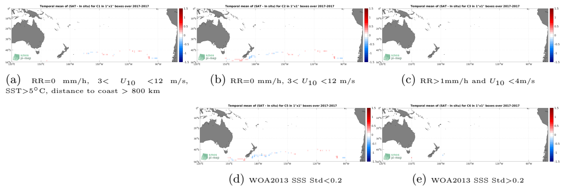
Figure 12: Temporal mean gridded over spatial boxes of size 1^\circ \times 1^\circ of \Delta SSS (SMAP SSS L3 v5.0 - Monthly (JPL) - TSG (GOSUD-Sailing-ship)) for 5 different subdatasets corresponding to:RR=0 mm/h, 3 < U_{10} < 12 m/s, SST >5^\circ\text{C} , distance to coast > 800 km (a), RR=0 mm/h, 3 < U_{10} < 12 m/s (b), RR >1 mm/h and U_{10} < 4 m/s (c), WOA2013 SSS Std <0.2 (d), WOA2013 SSS Std >0.2 (e).
