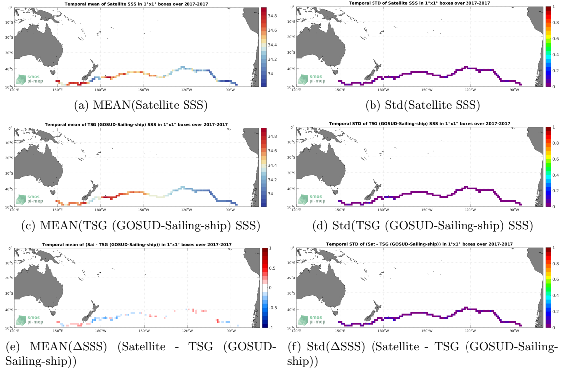
Figure 6: Temporal mean (left) and Std (right) of SSS from SMAP SSS L3 v5.0 - Monthly (JPL) (top), TSG (GOSUD-Sailing-ship) (middle), and of \Delta SSS (Satellite - TSG (GOSUD-Sailing-ship)). Only match-up pairs are used to generate these maps.
