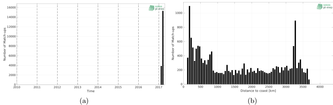
Figure 1: Number of match-ups between TSG (GOSUD-Sailing-ship) and SMAP SSS L3 v5.0 - Monthly (JPL) SSS as a function of time (a) and as function of the distance to coast (b) over the South Pacific Ocean Pi-MEP region and for the full satellite product period.
