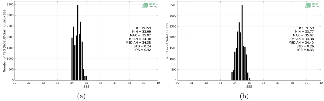
Figure 2: Histograms of SSS from TSG (GOSUD-Sailing-ship) (a) and SMAP SSS L3 v5.0 - Monthly (JPL) (b) considering all match-up pairs per bins of 0.1 over the South Pacific Ocean Pi-MEP region and for the full satellite product period.
