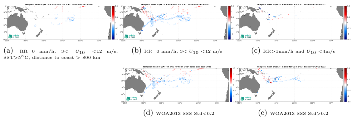
Figure 14: Temporal mean gridded over spatial boxes of size 1^\circ \times 1^\circ of \Delta SSS (SMAP SSS L3 v5.0 - Monthly (JPL) - TSG (GOSUD-Research-vessel)) for 5 different subdatasets corresponding to:RR=0 mm/h, 3 < U_{10} < 12 m/s, SST>5°C, distance to coast > 800 km (a), RR=0 mm/h, 3 < U_{10} < 12 m/s (b), RR>1mm/h and U_{10} < 4 m/s (c), WOA2013 SSS Std<0.2 (d), WOA2013 SSS Std>0.2 (e).
