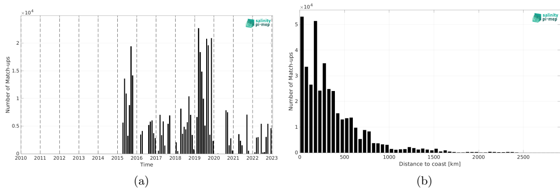
Figure 2: Number of match-ups between TSG (GOSUD-Research-vessel) and SMAP SSS L3 v5.0 - Monthly (JPL) SSS as a function of time (a) and as function of the distance to coast (b) over the South Pacific Ocean Pi-MEP region and for the full satellite product period.
