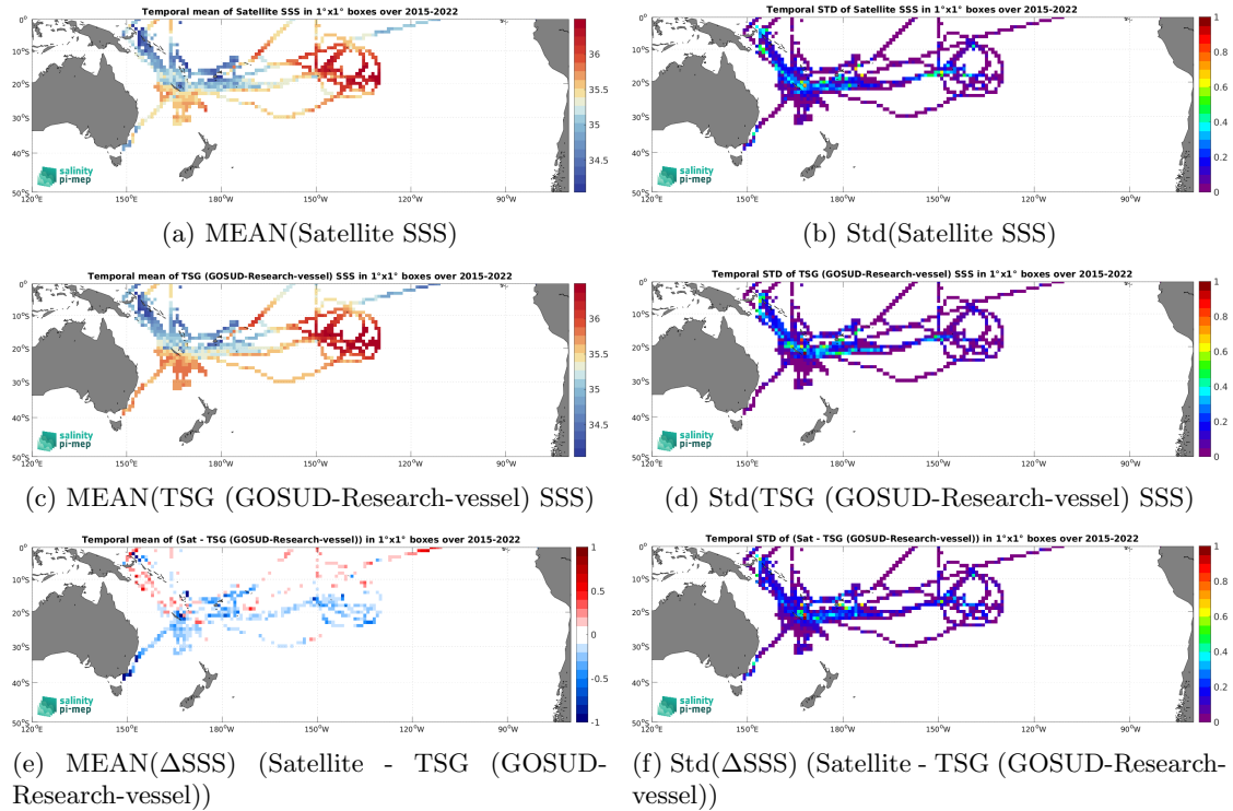
Figure 7: Temporal mean (left) and Std (right) of SSS from SMAP SSS L3 v5.0 - Monthly (JPL) (top), TSG (GOSUD-Research-vessel) (middle), and of \Delta SSS (Satellite - TSG (GOSUD-Research-vessel)). Only match-up pairs are used to generate these maps.
