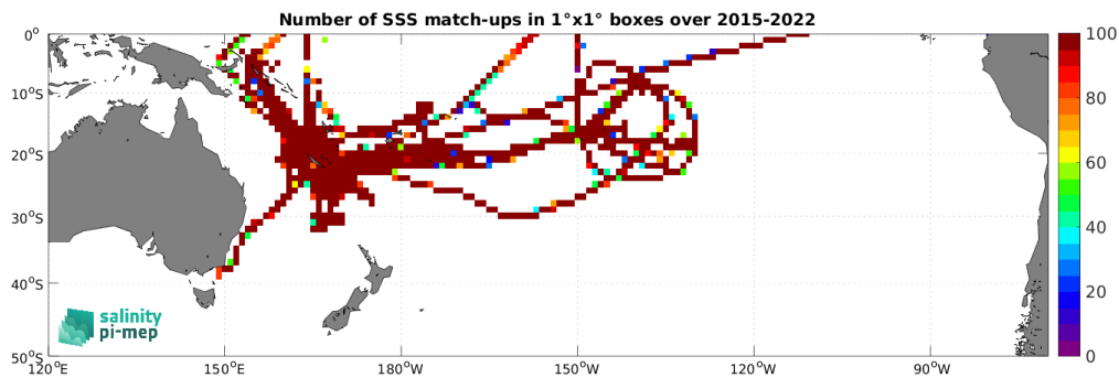
Figure 5: Number of SSS match-ups between TSG (GOSUD-Research-vessel) SSS and the SMAP SSS L3 v5.0 - Monthly (JPL) SSS product for the South Pacific Ocean Pi-MEP region over 1^\circ \times 1^\circ boxes and for the full satellite product period.
