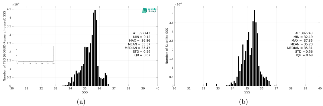
Figure 3: Histograms of SSS from TSG (GOSUD-Research-vessel) (a) and SMAP SSS L3 v5.0 - Monthly (JPL) (b) considering all match-up pairs per bins of 0.1 over the South Pacific Ocean Pi-MEP region and for the full satellite product period.
