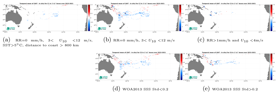
Figure 14: Temporal mean gridded over spatial boxes of size 1^\circ \times 1^\circ of \Delta\text{SSS} (SMAP SSS L3 v5.0 - Monthly (JPL) - TSG (GOSUD-Research-vessel)) for 5 different subdatasets corresponding to:RR=0 mm/h, 3 < U_{10} < 12 m/s, SST>5°C, distance to coast > 800 km (a), RR=0 mm/h, 3 < U_{10} < 12 m/s (b), RR>1mm/h and U_{10} < 4 m/s (c), WOA2013 SSS Std<0.2 (d), WOA2013 SSS Std>0.2 (e).
