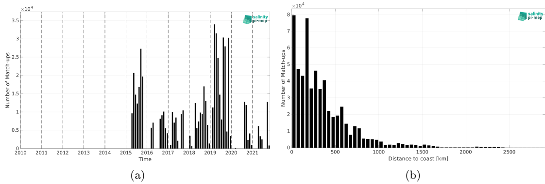
Figure 1: Number of match-ups between TSG (GOSUD-Research-vessel) and SMAP SSS L3 v5.0 - Monthly (JPL) SSS as a function of time (a) and as function of the distance to coast (b) over the South Pacific Ocean Pi-MEP region and for the full satellite product period.
