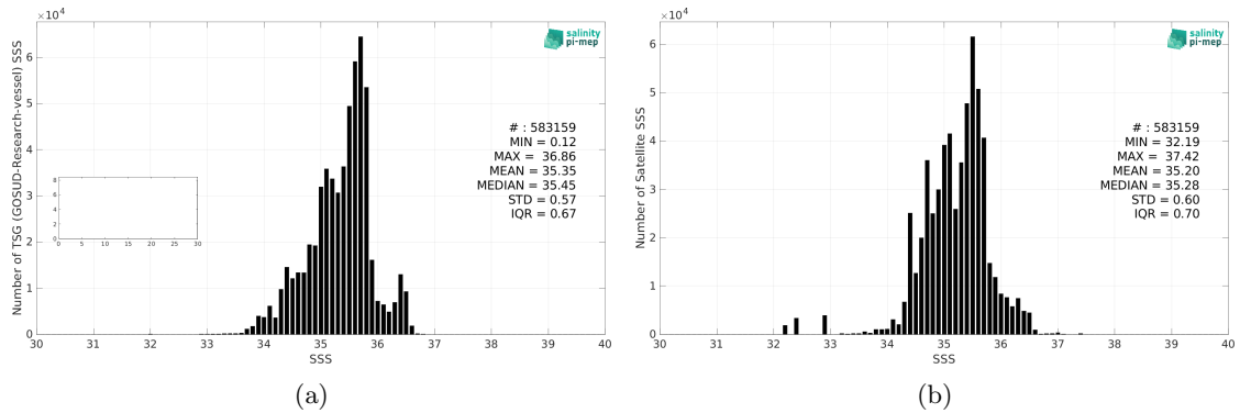
Figure 2: Histograms of SSS from TSG (GOSUD-Research-vessel) (a) and SMAP SSS L3 v5.0 - Monthly (JPL) (b) considering all match-up pairs per bins of 0.1 over the South Pacific Ocean Pi-MEP region and for the full satellite product period.
