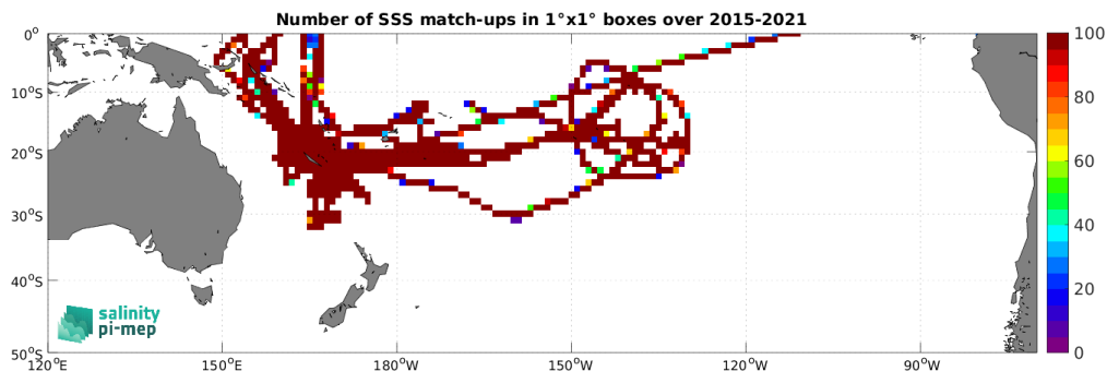
Figure 4: Number of SSS match-ups between TSG (GOSUD-Research-vessel) SSS and the SMAP SSS L3 v5.0 - Monthly (JPL) SSS product for the South Pacific Ocean Pi-MEP region over 1^\circ \times 1^\circ boxes and for the full satellite product period.
