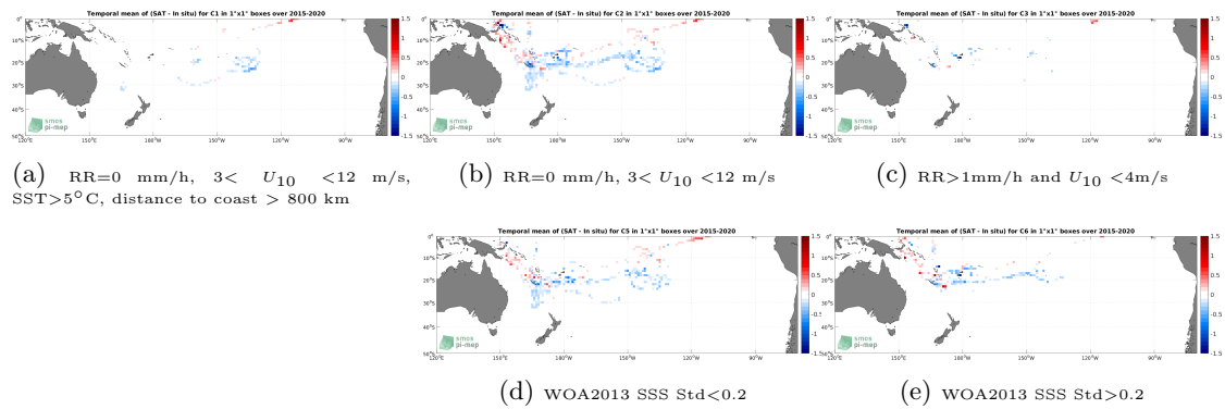
Figure 12: Temporal mean gridded over spatial boxes of size 1^\circ \times 1^\circ of \Delta SSS (SMAP SSS L3 v5.0 - Monthly (JPL) - TSG (GOSUD-Research-vessel)) for 5 different subdatasets corresponding to:RR=0 mm/h, 3 < U_{10} < 12 m/s, SST >5^\circ\text{C} , distance to coast > 800 km (a), RR=0 mm/h, 3 < U_{10} < 12 m/s (b), RR >1 mm/h and U_{10} < 4 m/s (c), WOA2013 SSS Std <0.2 (d), WOA2013 SSS Std >0.2 (e).
