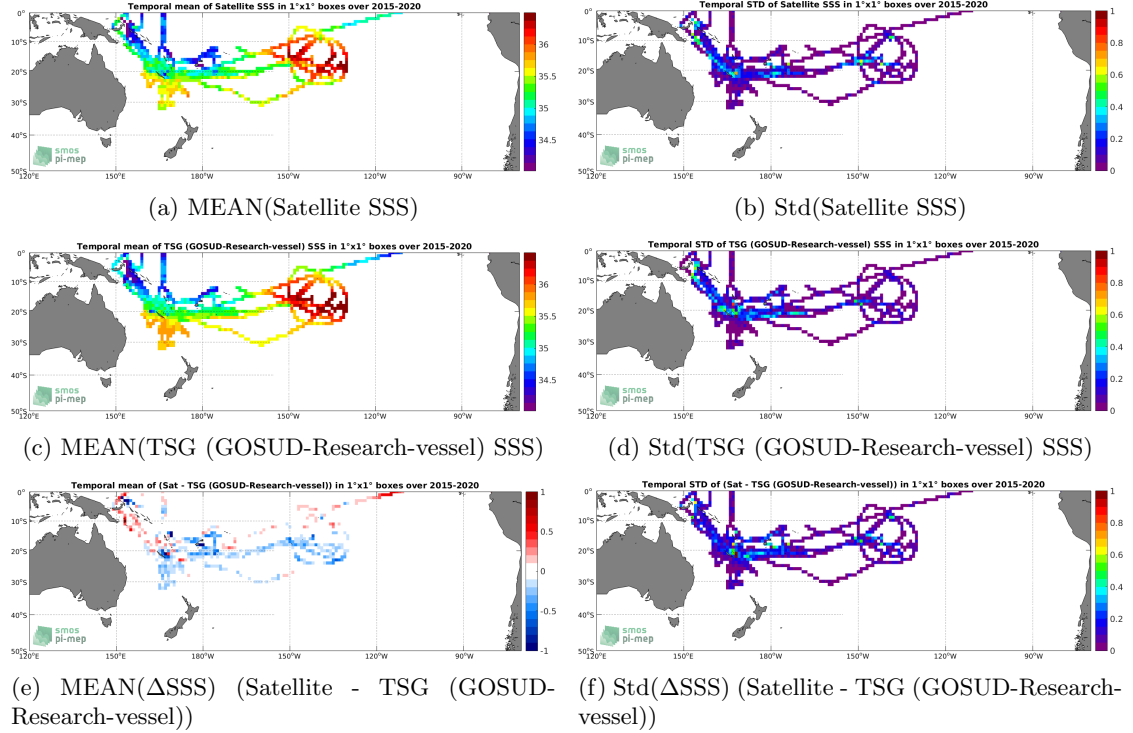
Figure 6: Temporal mean (left) and Std (right) of SSS from SMAP SSS L3 v5.0 - Monthly (JPL) (top), TSG (GOSUD-Research-vessel) (middle), and of \Delta SSS (Satellite - TSG (GOSUD-Research-vessel)). Only match-up pairs are used to generate these maps.
