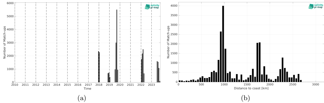
Figure 2: Number of match-ups between Saildrone and SMAP SSS L3 v5.0 - Monthly (JPL) SSS as a function of time (a) and as function of the distance to coast (b) over the South Pacific Ocean Pi-MEP region and for the full satellite product period.
