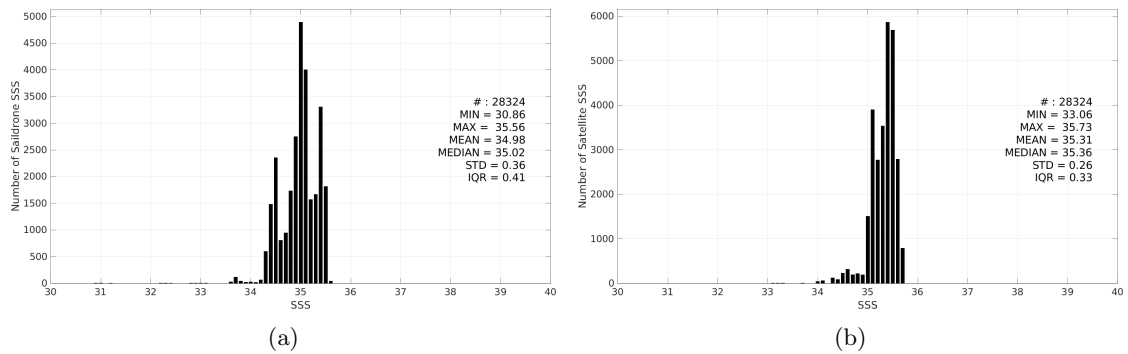
Figure 3: Histograms of SSS from Saildrone (a) and SMAP SSS L3 v5.0 - Monthly (JPL) (b) considering all match-up pairs per bins of 0.1 over the South Pacific Ocean Pi-MEP region and for the full satellite product period.
