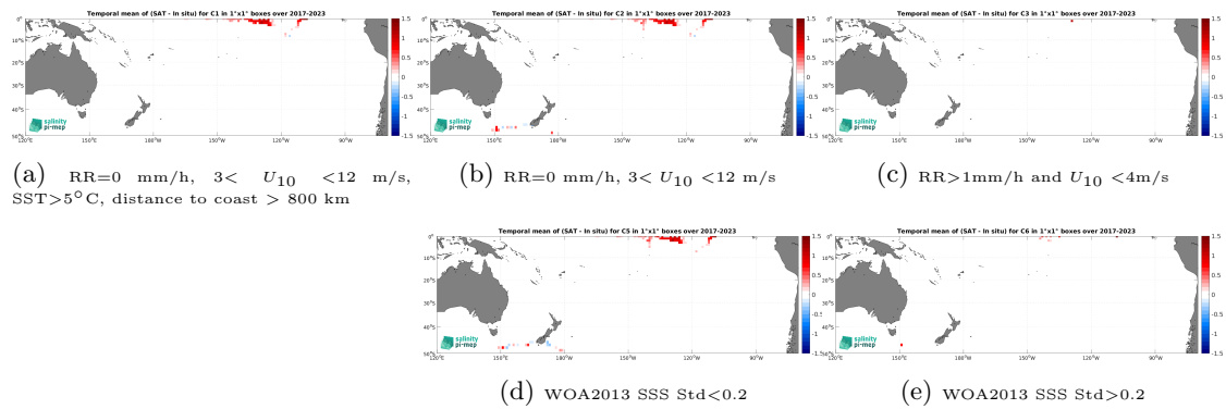
Figure 14: Temporal mean gridded over spatial boxes of size 1^\circ \times 1^\circ of \Delta\text{SSS} (SMAP SSS L3 v5.0 - Monthly (JPL) - Sairdrone) for 5 different subdatasets corresponding to:RR=0 mm/h, 3 < U_{10} < 12 m/s, SST>5°C, distance to coast > 800 km (a), RR=0 mm/h, 3 < U_{10} < 12 m/s (b), RR>1mm/h and U_{10} < 4 m/s (c), WOA2013 SSS Std<0.2 (d), WOA2013 SSS Std>0.2 (e).
