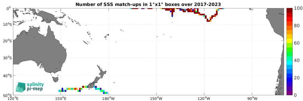
Figure 5: Number of SSS match-ups between Saildrone SSS and the SMAP SSS L3 v5.0 - Monthly (JPL) SSS product for the South Pacific Ocean Pi-MEP region over 1^\circ \times 1^\circ boxes and for the full satellite product period.
