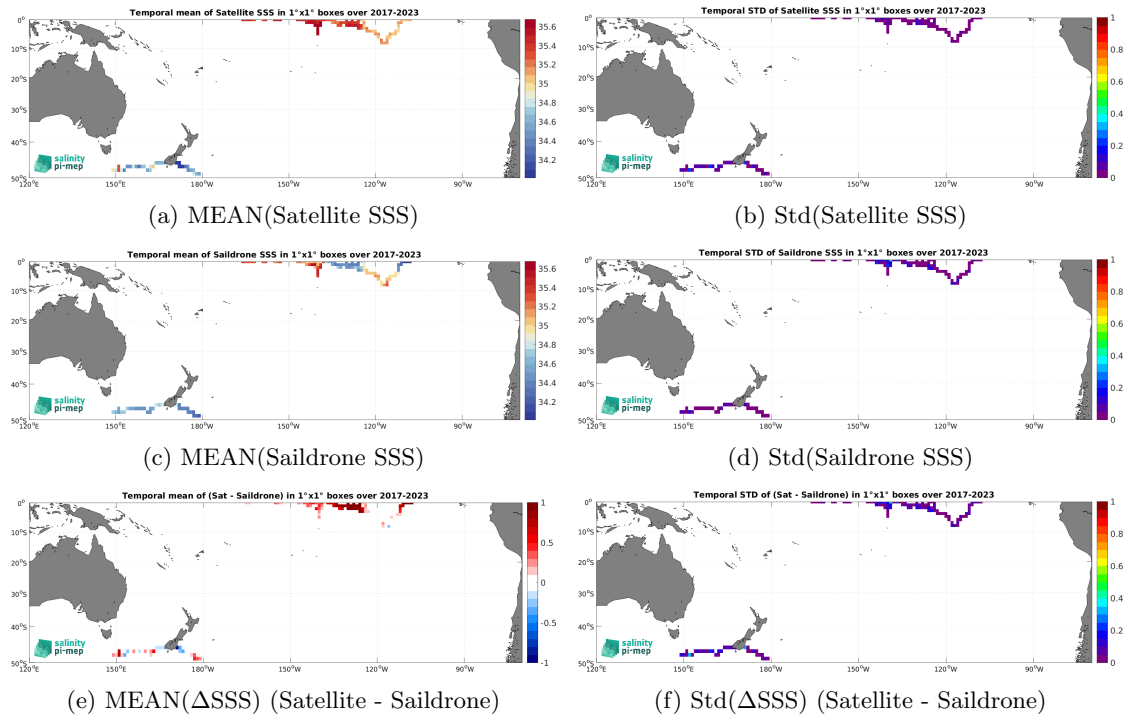
Figure 7: Temporal mean (left) and Std (right) of SSS from SMAP SSS L3 v5.0 - Monthly (JPL) (top), Saildrone (middle), and of \Delta SSS (Satellite - Saildrone). Only match-up pairs are used to generate these maps.
