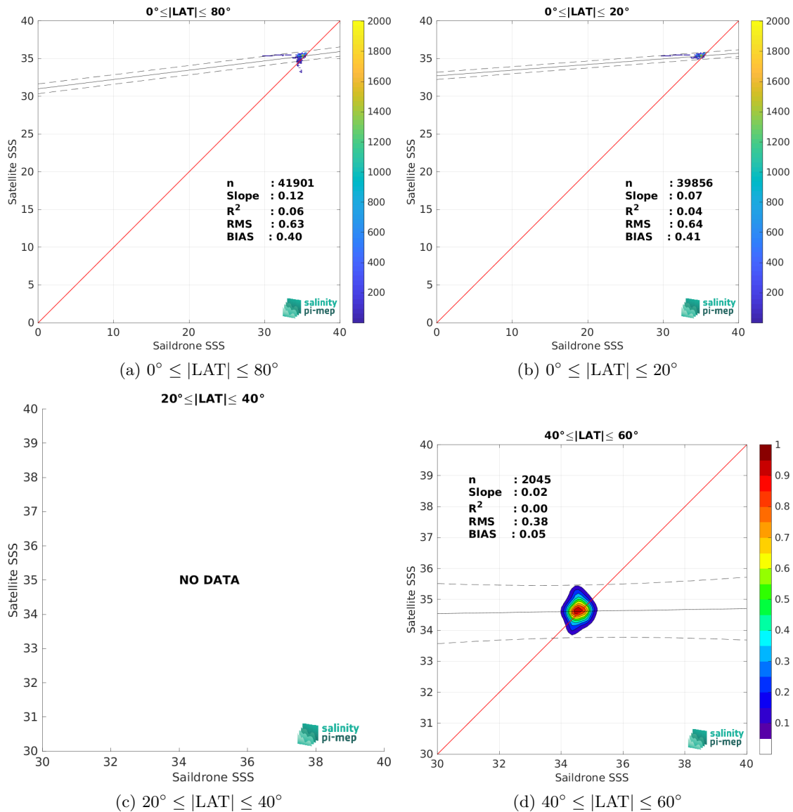
Figure 9: Contour maps of the concentration of SMAP SSS L3 v5.0 - Monthly (JPL) SSS (y-axis) versus Sairdrone SSS (x-axis) at match-up pairs for different latitude bands. For each plot, the red line shows x=y . The black thin and dashed lines indicate a linear fit through the data cloud and the \pm 95\% confidence levels, respectively. The number match-up pairs n , the slope and R^2 coefficient of the linear fit, the root mean square (RMS) and the mean bias between satellite and in situ data are indicated for each latitude band in each plots.
