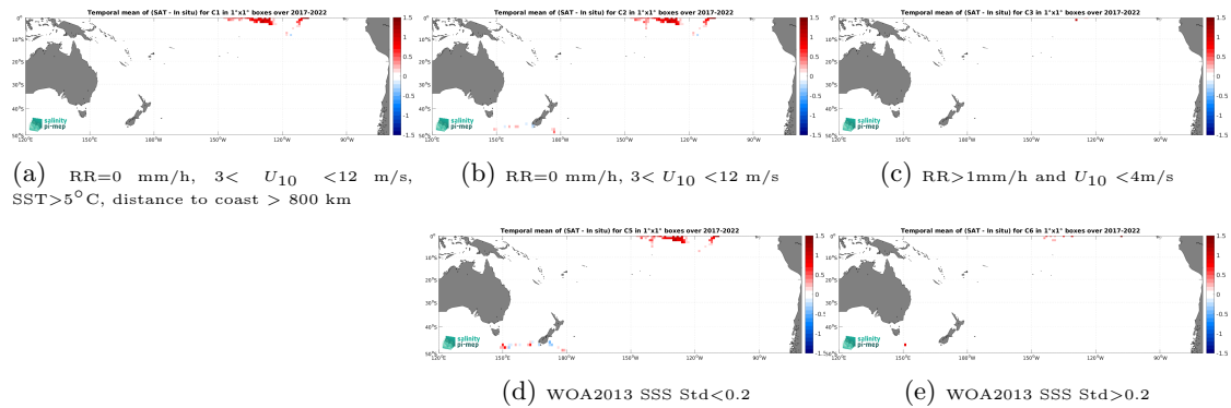
Figure 12: Temporal mean gridded over spatial boxes of size 1^\circ \times 1^\circ of \Delta\text{SSS} (SMAP SSS L3 v5.0 - Monthly (JPL) - Saildrone) for 5 different subdatasets corresponding to:RR=0 mm/h, 3 < U_{10} < 12 m/s, SST >5^\circ\text{C} , distance to coast > 800 km (a), RR=0 mm/h, 3 < U_{10} < 12 m/s (b), RR >1 mm/h and U_{10} < 4 m/s (c), WOA2013 SSS Std <0.2 (d), WOA2013 SSS Std >0.2 (e).
