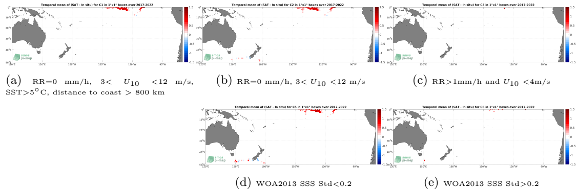
Figure 12: Temporal mean gridded over spatial boxes of size 1^\circ \times 1^\circ of \Delta SSS (SMAP SSS L3 v5.0 - Monthly (JPL) - Saildrone) for 5 different subdatasets corresponding to:RR=0 mm/h, 3 < U_{10} < 12 m/s, SST >5^\circ C, distance to coast > 800 km (a), RR=0 mm/h, 3 < U_{10} < 12 m/s (b), RR >1 mm/h and U_{10} < 4 m/s (c), WOA2013 SSS Std <0.2 (d), WOA2013 SSS Std >0.2 (e).
