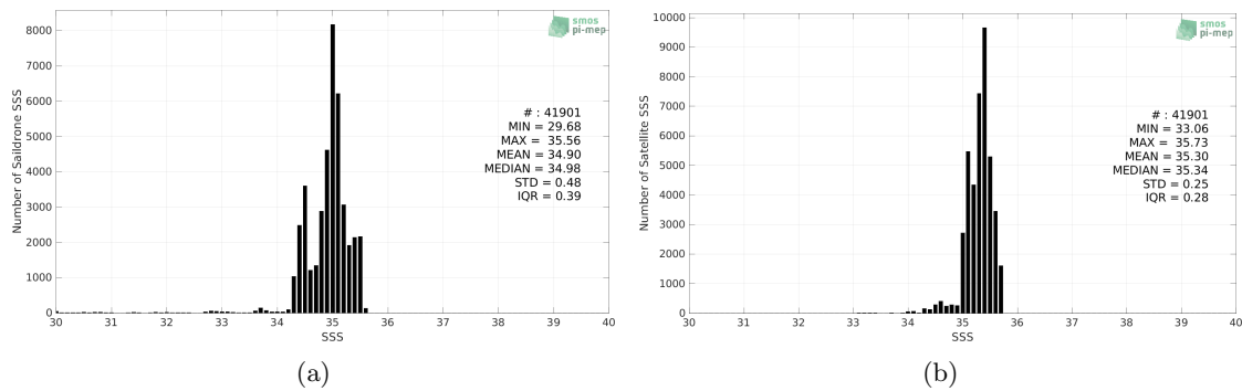
Figure 2: Histograms of SSS from Saildrone (a) and SMAP SSS L3 v5.0 - Monthly (JPL) (b) considering all match-up pairs per bins of 0.1 over the South Pacific Ocean Pi-MEP region and for the full satellite product period.
