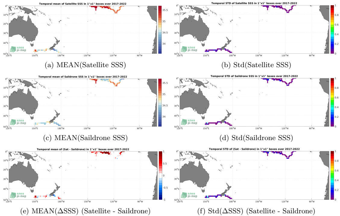
Figure 6: Temporal mean (left) and Std (right) of SSS from SMAP SSS L3 v5.0 - Monthly (JPL) (top), Saildrone (middle), and of \Delta SSS (Satellite - Saildrone). Only match-up pairs are used to generate these maps.
