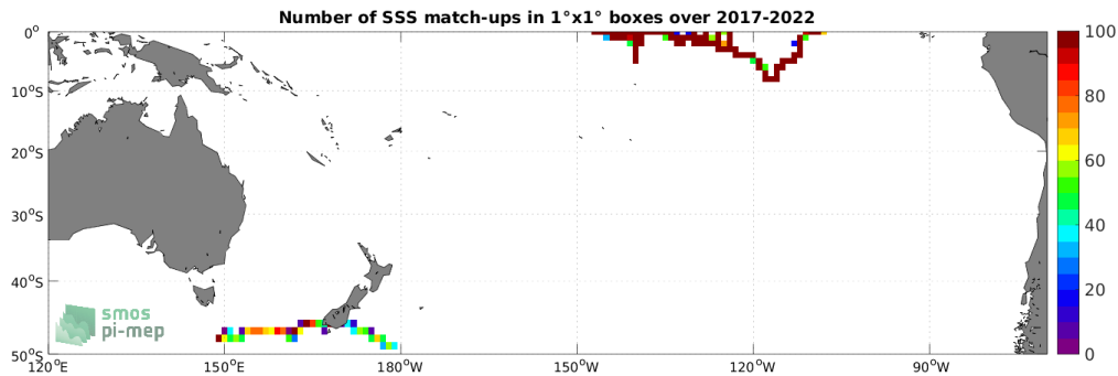
Figure 4: Number of SSS match-ups between Saildrone SSS and the SMAP SSS L3 v5.0 - Monthly (JPL) SSS product for the South Pacific Ocean Pi-MEP region over 1^\circ \times 1^\circ boxes and for the full satellite product period.
