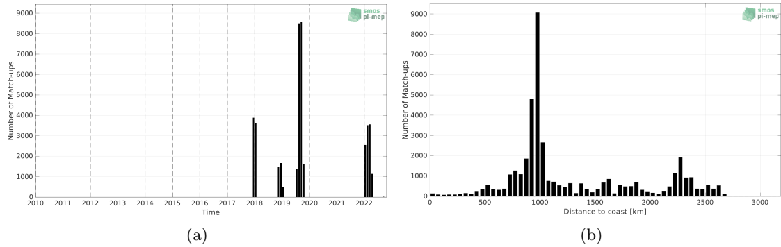
Figure 1: Number of match-ups between Saildrone and SMAP SSS L3 v5.0 - Monthly (JPL) SSS as a function of time (a) and as function of the distance to coast (b) over the South Pacific Ocean Pi-MEP region and for the full satellite product period.
