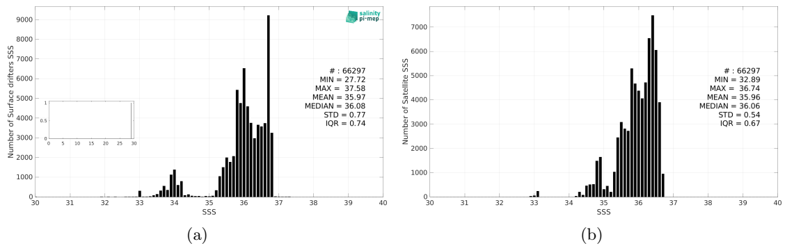
Figure 3: Histograms of SSS from Surface drifters (a) and SMAP SSS L3 v5.0 - Monthly (JPL) (b) considering all match-up pairs per bins of 0.1 over the South Pacific Ocean Pi-MEP region and for the full satellite product period.
