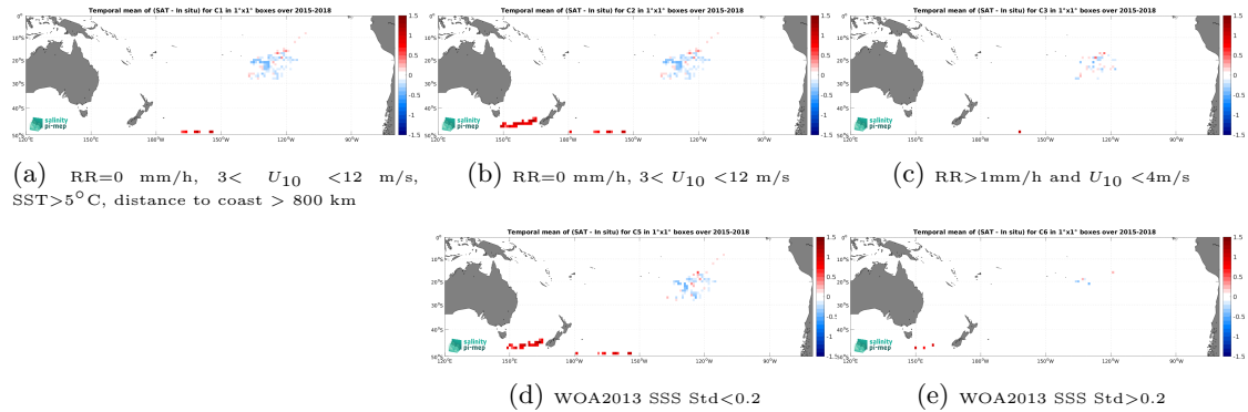
Figure 13: Temporal mean gridded over spatial boxes of size 1^\circ \times 1^\circ of \Delta SSS (SMAP SSS L3 v5.0 - Monthly (JPL) - Surface drifters) for 5 different subdatasets corresponding to:RR=0 mm/h, 3 < U_{10} < 12 m/s, SST >5^\circ C, distance to coast > 800 km (a), RR=0 mm/h, 3 < U_{10} < 12 m/s (b), RR >1 mm/h and U_{10} < 4 m/s (c), WOA2013 SSS Std <0.2 (d), WOA2013 SSS Std >0.2 (e).
