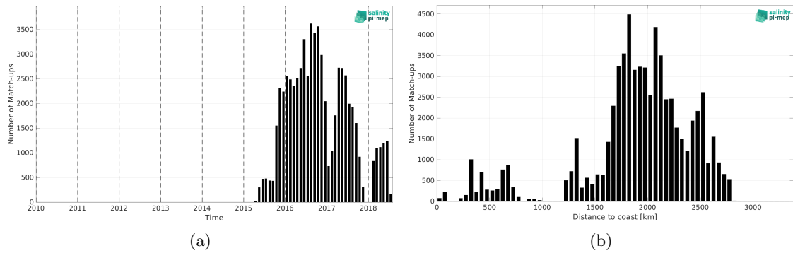
Figure 2: Number of match-ups between Surface drifters and SMAP SSS L3 v5.0 - Monthly (JPL) SSS as a function of time (a) and as function of the distance to coast (b) over the South Pacific Ocean Pi-MEP region and for the full satellite product period.
