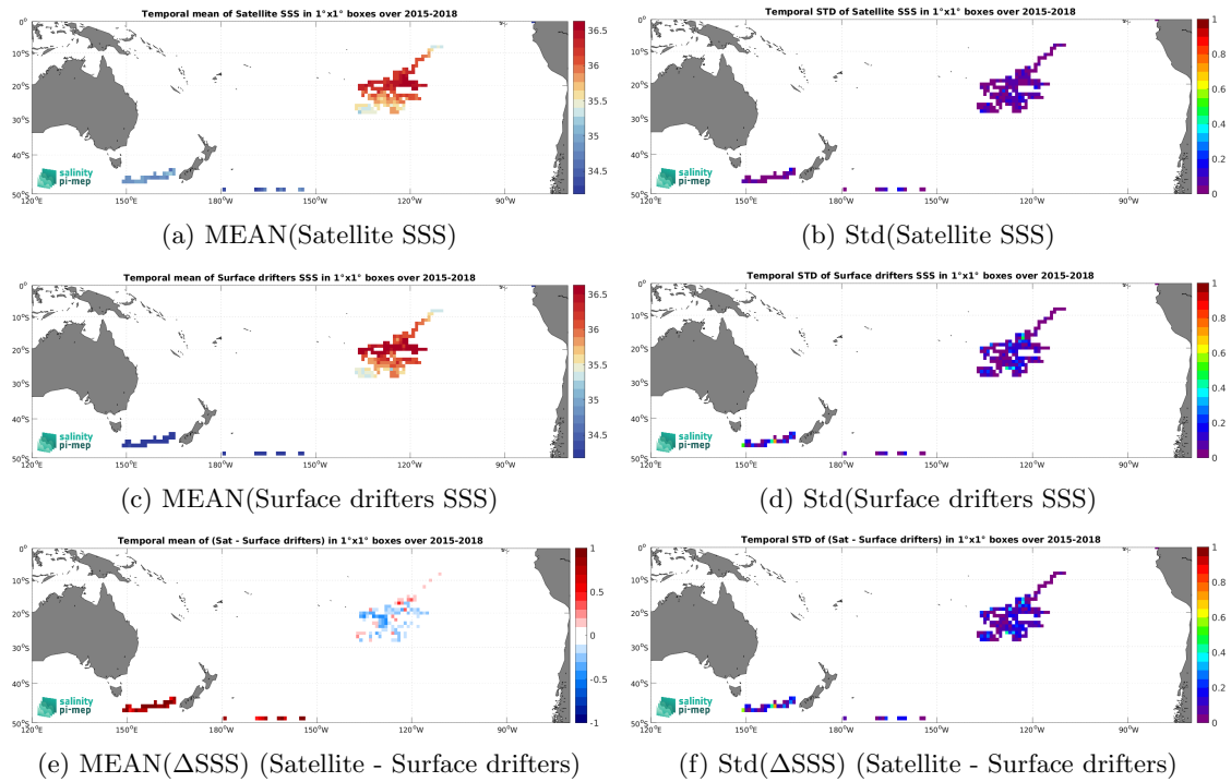
Figure 6: Temporal mean (left) and Std (right) of SSS from SMAP SSS L3 v5.0 - Monthly (JPL) (top), Surface drifters (middle), and of \Delta SSS (Satellite - Surface drifters). Only match-up pairs are used to generate these maps.
