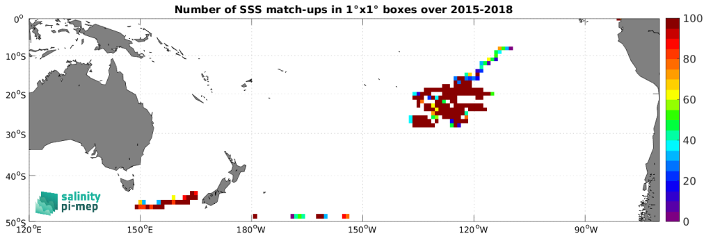
Figure 4: Number of SSS match-ups between Surface drifters SSS and the SMAP SSS L3 v5.0 - Monthly (JPL) SSS product for the South Pacific Ocean Pi-MEP region over 1^\circ \times 1^\circ boxes and for the full satellite product period.
