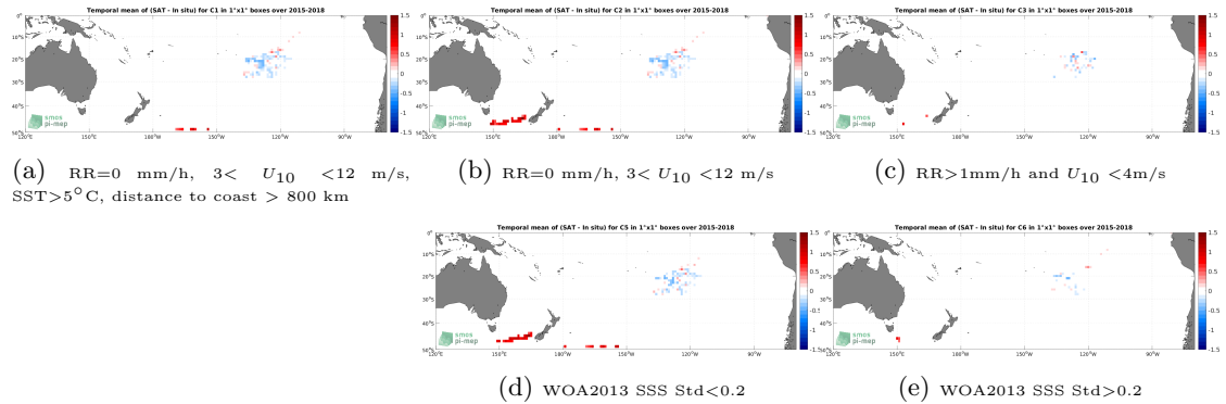
Figure 11: Temporal mean gridded over spatial boxes of size 1^\circ \times 1^\circ of \Delta SSS (SMAP SSS L3 v5.0 - Monthly (JPL) - Surface drifters) for 5 different subdatasets corresponding to:RR=0 mm/h, 3 < U_{10} < 12 m/s, SST >5^\circ C, distance to coast > 800 km (a), RR=0 mm/h, 3 < U_{10} < 12 m/s (b), RR >1 mm/h and U_{10} < 4 m/s (c), WOA2013 SSS Std <0.2 (d), WOA2013 SSS Std >0.2 (e).
