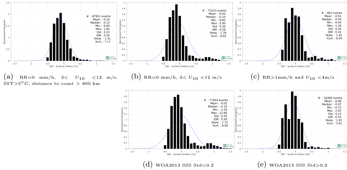
Figure 12: Normalized histogram of \Delta\text{SSS} (SMAP SSS L3 v5.0 - Monthly (JPL) - Surface drifters) for 5 different subdatasets corresponding to: RR=0 mm/h, 3 < U_{10} < 12 m/s, SST > 5^\circ\text{C} , distance to coast > 800 km (a), RR=0 mm/h, 3 < U_{10} < 12 m/s (b), RR > 1 mm/h and U_{10} < 4 m/s (c), WOA2013 SSS Std < 0.2 (d), WOA2013 SSS Std > 0.2 (e).
