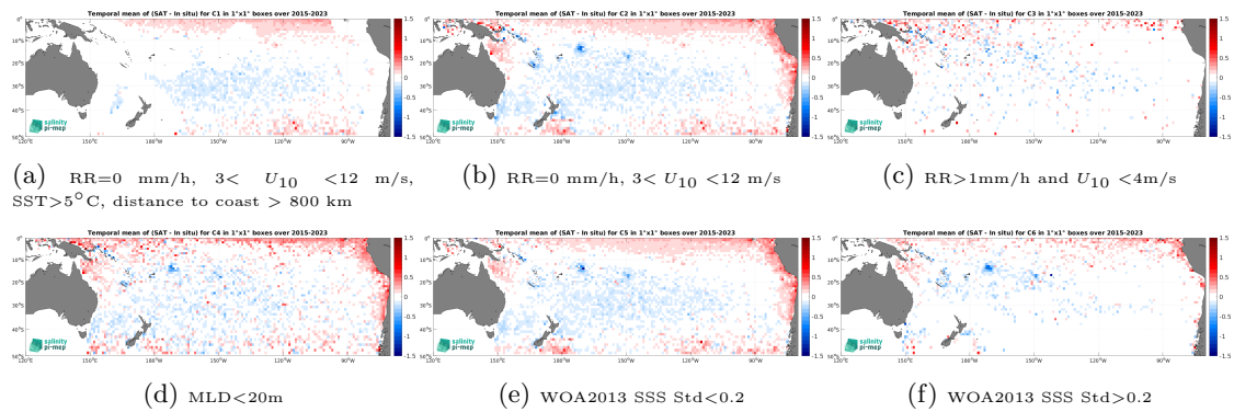
Figure 12: Temporal mean gridded over spatial boxes of size 1^\circ \times 1^\circ of \Delta SSS (SMAP SSS L3 v5.0 - Monthly (JPL) - Argo) for 6 different subdatasets corresponding to:RR=0 mm/h, 3 < U_{10} < 12 m/s, SST >5^\circ\text{C} , distance to coast > 800 km (a), RR=0 mm/h, 3 < U_{10} < 12 m/s (b), RR >1 mm/h and U_{10} < 4 m/s (c),MLD <20 m (d),WOA2013 SSS Std <0.2 (e),WOA2013 SSS Std >0.2 (f).
