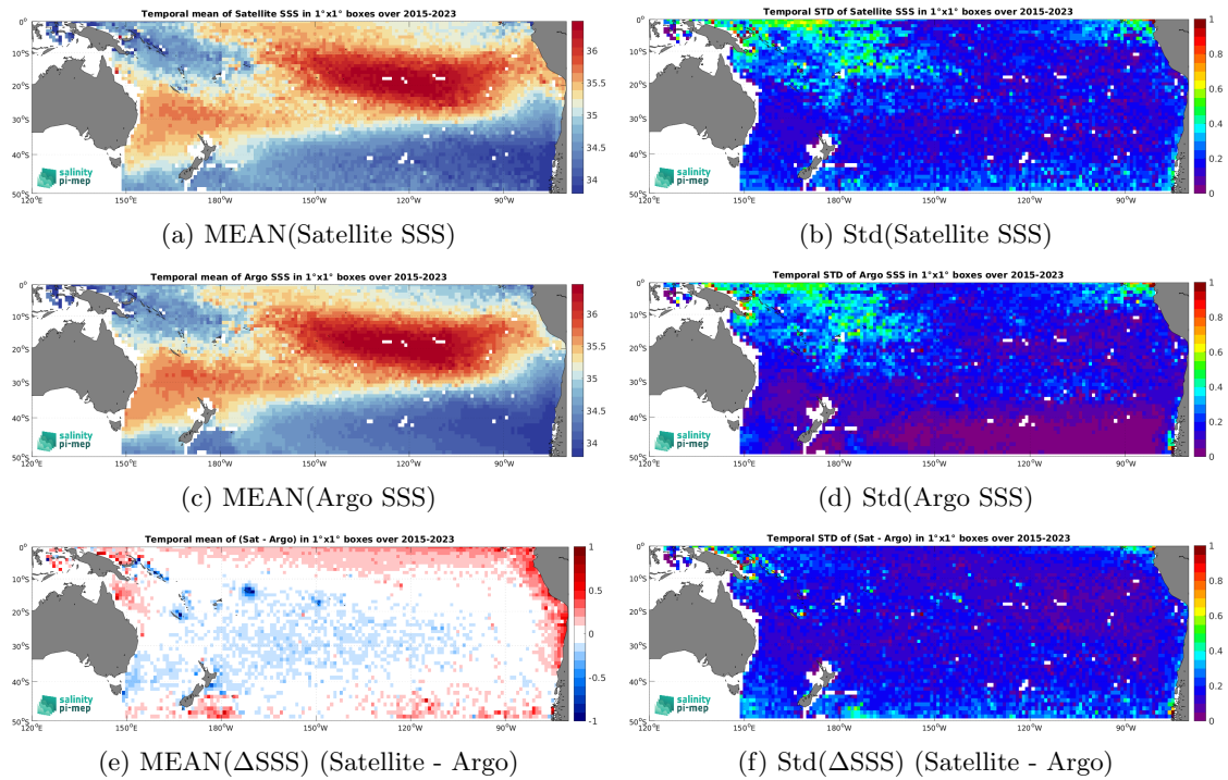
Figure 6: Temporal mean (left) and Std (right) of SSS from SMAP SSS L3 v5.0 - Monthly (JPL) (top), Argo (middle), and of \Delta SSS (Satellite - Argo). Only match-up pairs are used to generate these maps.
