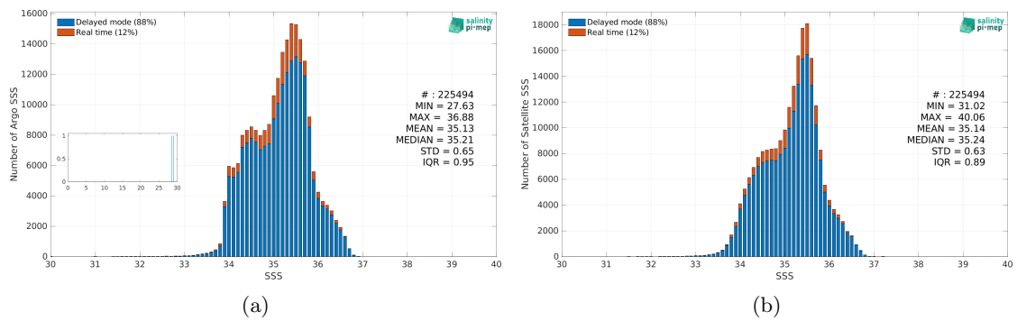
Figure 2: Histograms of SSS from Argo (a) and SMAP SSS L3 v5.0 - Monthly (JPL) (b) considering all match-up pairs per bins of 0.1 over the South Pacific Ocean Pi-MEP region and for the full satellite product period.
