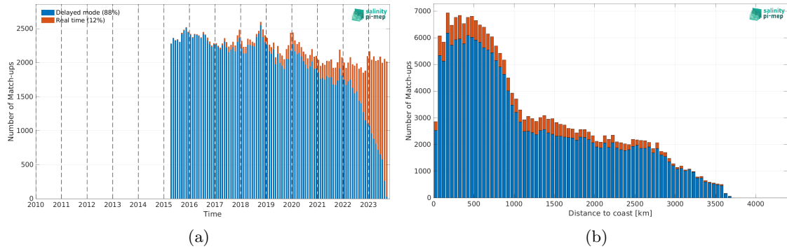
Figure 1: Number of match-ups between Argo and SMAP SSS L3 v5.0 - Monthly (JPL) SSS as a function of time (a) and as function of the distance to coast (b) over the South Pacific Ocean Pi-MEP region and for the full satellite product period.
