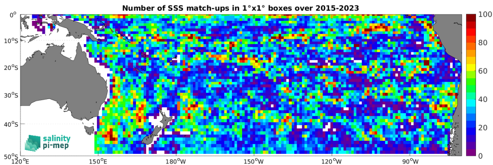
Figure 4: Number of SSS match-ups between Argo SSS and the SMAP SSS L3 v5.0 - Monthly (JPL) SSS product for the South Pacific Ocean Pi-MEP region over 1^\circ \times 1^\circ boxes and for the full satellite product period.
