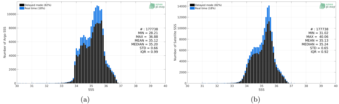
Figure 2: Histograms of SSS from Argo (a) and SMAP SSS L3 v5.0 - Monthly (JPL) (b) considering all match-up pairs per bins of 0.1 over the South Pacific Ocean Pi-MEP region and for the full satellite product period.
