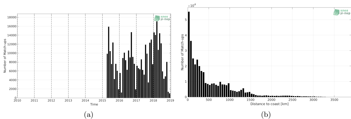
Figure 1: Number of match-ups between TSG-LEGOS-DM and SMAP-L3-JPL-V4.3-MONTHLY-60KM SSS as a function of time (a) and as function of the distance to coast (b) over the South Pacific Ocean Pi-MEP region and for the full satellite product period.
