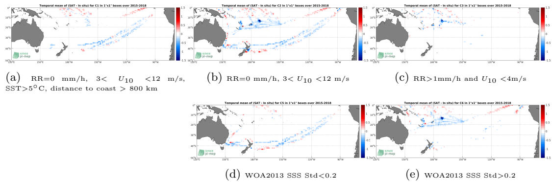
Figure 12: Temporal mean gridded over spatial boxes of size 1^\circ \times 1^\circ of \Delta SSS (SMAP-L3-JPL-V4.3-MONTHLY-60KM - TSG-LEGOS-DM) for 5 different subdatasets corresponding to:RR=0 mm/h, 3 < U_{10} < 12 m/s, SST >5^\circ C, distance to coast > 800 km (a), RR=0 mm/h, 3 < U_{10} < 12 m/s (b), RR >1 mm/h and U_{10} < 4 m/s (c), WOA2013 SSS Std <0.2 (d), WOA2013 SSS Std >0.2 (e).
