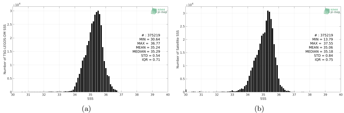
Figure 2: Histograms of SSS from TSG-LEGOS-DM (a) and SMAP-L3-JPL-V4.3-MONTHLY-60KM (b) considering all match-up pairs per bins of 0.1 over the South Pacific Ocean Pi-MEP region and for the full satellite product period.
