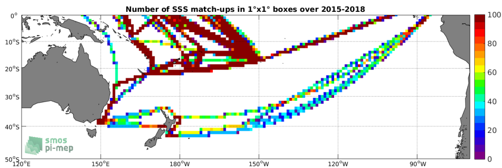
Figure 4: Number of SSS match-ups between TSG-LEGOS-DM SSS and the SMAP-L3-JPL-V4.3-MONTHLY-60KM SSS product for the South Pacific Ocean Pi-MEP region over 1°x1° boxes and for the full satellite product period.
