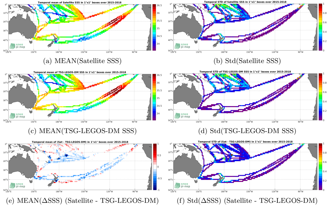
Figure 6: Temporal mean (left) and Std (right) of SSS from SMAP-L3-JPL-V4.3-MONTHLY-60KM (top), TSG-LEGOS-DM (middle), and of \Delta SSS (Satellite - TSG-LEGOS-DM). Only match-up pairs are used to generate these maps.
