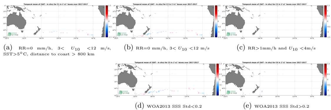
Figure 12: Temporal mean gridded over spatial boxes of size 1^\circ \times 1^\circ of \Delta SSS (SMAP-L3-JPL-V4.3-MONTHLY-60KM - TSG-GOSUD-Sailing-ship) for 5 different subdatasets corresponding to:RR=0 mm/h, 3 < U_{10} < 12 m/s, SST >5^\circ\text{C} , distance to coast > 800 km (a), RR=0 mm/h, 3 < U_{10} < 12 m/s (b), RR >1 mm/h and U_{10} < 4 m/s (c), WOA2013 SSS Std <0.2 (d), WOA2013 SSS Std >0.2 (e).
