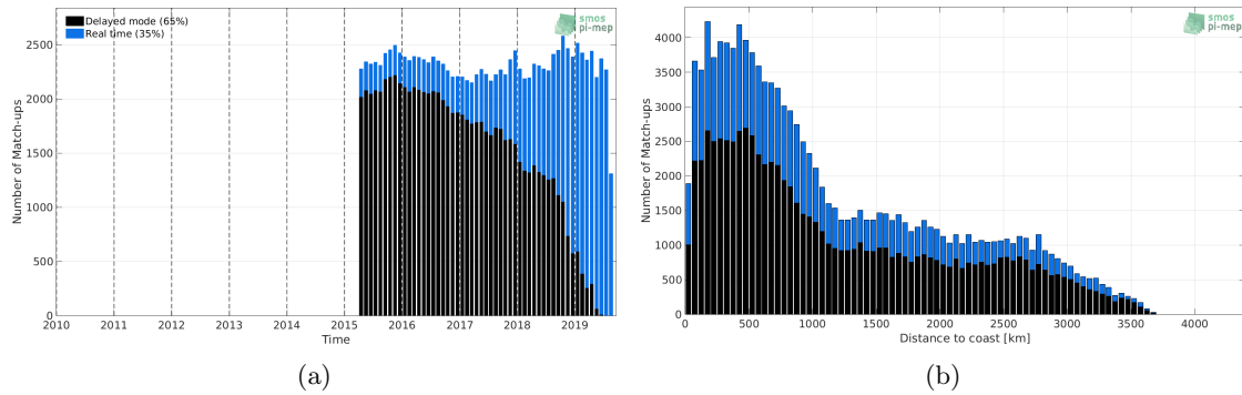
Figure 1: Number of match-ups between Argo and SMAP-L3-JPL-V4.3-MONTHLY-60KM SSS as a function of time (a) and as function of the distance to coast (b) over the South Pacific Ocean Pi-MEP region and for the full satellite product period.
