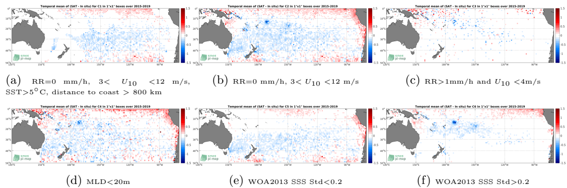
Figure 12: Temporal mean gridded over spatial boxes of size 1^\circ \times 1^\circ of \Delta SSS (SMAP-L3-JPL-V4.3-MONTHLY-60KM - Argo) for 6 different subdatasets corresponding to:RR=0 mm/h, 3 < U_{10} < 12 m/s, SST >5^\circ C, distance to coast > 800 km (a), RR=0 mm/h, 3 < U_{10} < 12 m/s (b), RR >1 mm/h and U_{10} < 4 m/s (c),MLD <20 m (d),WOA2013 SSS Std <0.2 (e),WOA2013 SSS Std >0.2 (f).
