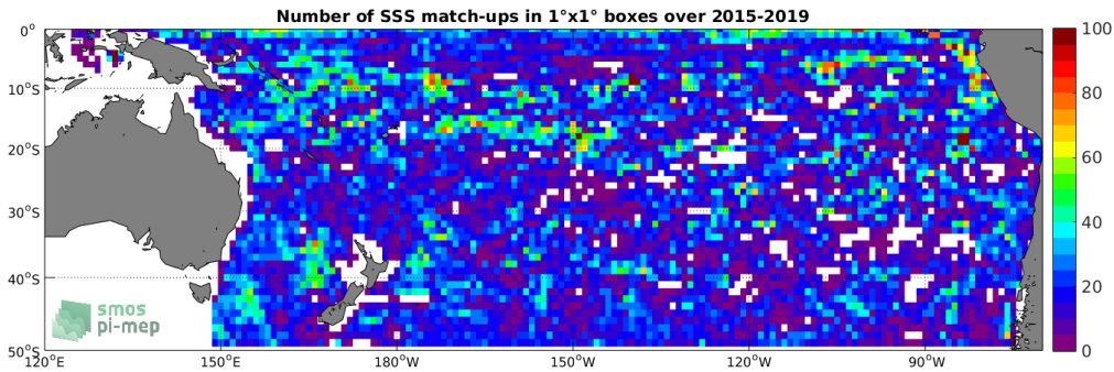
Figure 4: Number of SSS match-ups between Argo SSS and the SMAP-L3-JPL-V4.3-MONTHLY-60KM SSS product for the South Pacific Ocean Pi-MEP region over 1^\circ \times 1^\circ boxes and for the full satellite product period.
