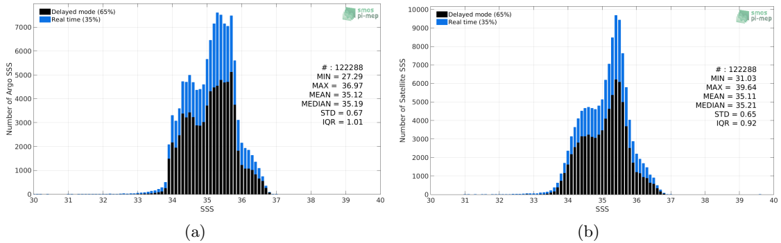
Figure 2: Histograms of SSS from Argo (a) and SMAP-L3-JPL-V4.3-MONTHLY-60KM (b) considering all match-up pairs per bins of 0.1 over the South Pacific Ocean Pi-MEP region and for the full satellite product period.
