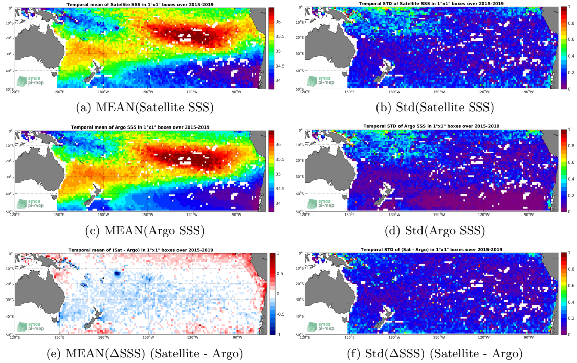
Figure 6: Temporal mean (left) and Std (right) of SSS from SMAP-L3-JPL-V4.3-MONTHLY-60KM (top), Argo (middle), and of \Delta SSS (Satellite - Argo). Only match-up pairs are used to generate these maps.
