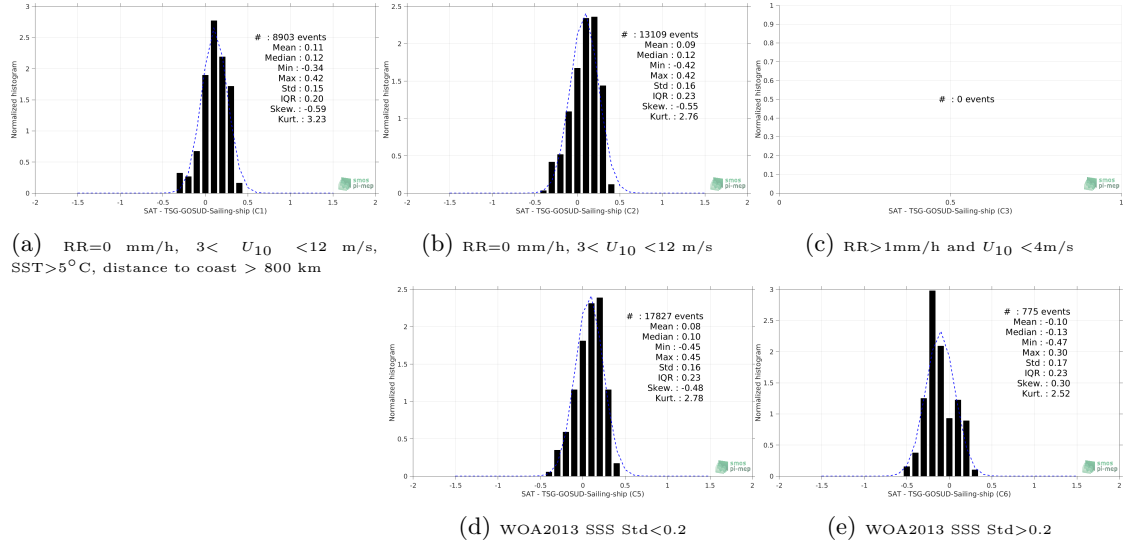
Figure 13: Normalized histogram of \Delta\text{SSS} (SMAP-L3-JPL-V4.2-MONTHLY-60KM - TSG-GOSUD-Sailing-ship) for 5 different subdatasets corresponding to: RR=0 mm/h, 3 < U_{10} < 12 m/s, SST > 5^{\circ}\text{C} , distance to coast > 800 km (a), RR=0 mm/h, 3 < U_{10} < 12 m/s (b), RR > 1 mm/h and U_{10} < 4 m/s (c), WOA2013 SSS Std < 0.2 (d), WOA2013 SSS Std > 0.2 (e).
