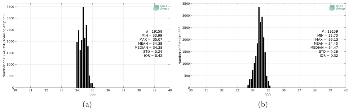
Figure 2: Histograms of SSS from TSG-GOSUD-Sailing-ship (a) and SMAP-L3-JPL-V4.2-MONTHLY-60KM (b) considering all match-up pairs per bins of 0.1 over the South Pacific Ocean Pi-MEP region and for the full satellite product period.
