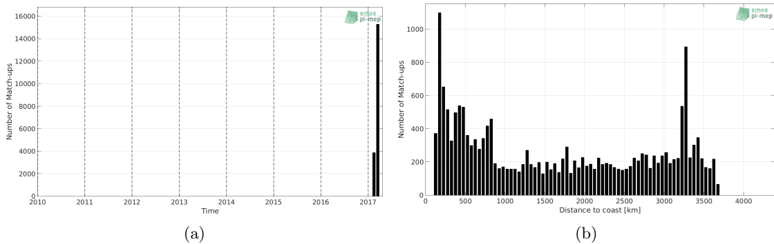
Figure 1: Number of match-ups between TSG-GOSUD-Sailing-ship and SMAP-L3-JPL-V4.2-MONTHLY-60KM SSS as a function of time (a) and as function of the distance to coast (b) over the South Pacific Ocean Pi-MEP region and for the full satellite product period.
