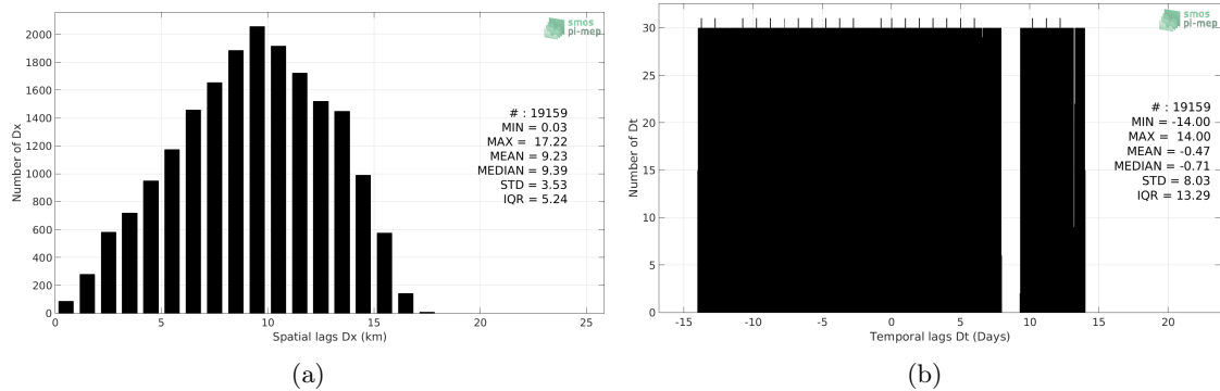
Figure 5: Histograms of the spatial (a) and temporal (b) lags between the time of the TSG-GOSUD-Sailing-ship measurements and the date of the corresponding SMAP-L3-JPL-V4.2-MONTHLY-60KM SSS product.
