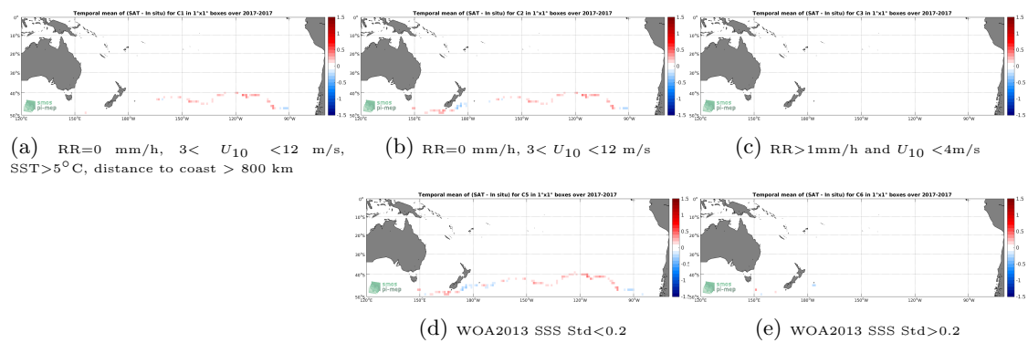
Figure 12: Temporal mean gridded over spatial boxes of size 1^\circ \times 1^\circ of \Delta SSS (SMAP-L3-JPL-V4.2-MONTHLY-60KM - TSG-GOSUD-Sailing-ship) for 5 different subdatasets corresponding to:RR=0 mm/h, 3 < U_{10} < 12 m/s, SST >5^\circ C, distance to coast > 800 km (a), RR=0 mm/h, 3 < U_{10} < 12 m/s (b), RR >1 mm/h and U_{10} < 4 m/s (c), WOA2013 SSS Std <0.2 (d), WOA2013 SSS Std >0.2 (e).
