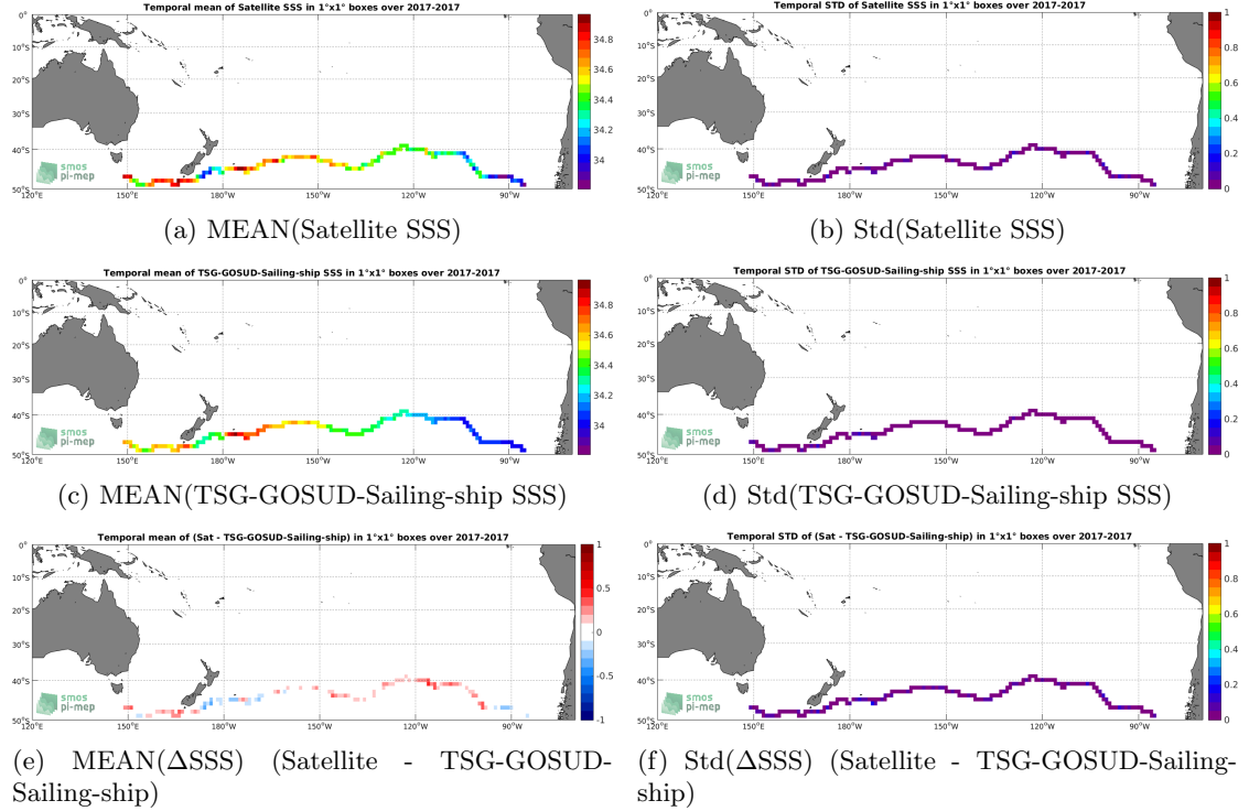
Figure 6: Temporal mean (left) and Std (right) of SSS from SMAP-L3-JPL-V4.2-MONTHLY-60KM (top), TSG-GOSUD-Sailing-ship (middle), and of \Delta SSS (Satellite - TSG-GOSUD-Sailing-ship). Only match-up pairs are used to generate these maps.
