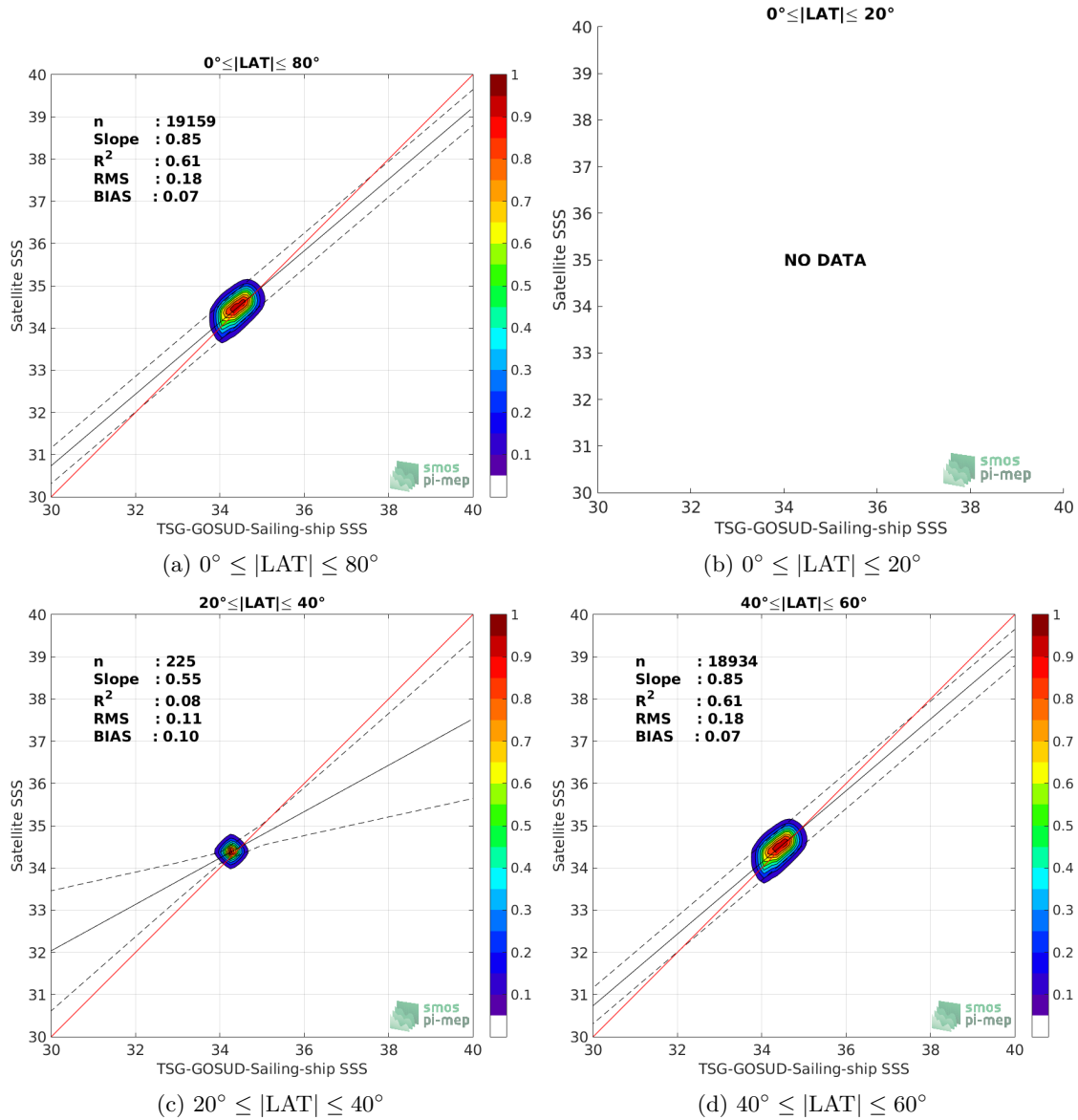
Figure 9: Contour maps of the concentration of SMAP-L3-JPL-V4.2-MONTHLY-60KM SSS (y-axis) versus TSG-GOSUD-Sailing-ship SSS (x-axis) at match-up pairs for different latitude bands. For each plot, the red line shows x=y . The black thin and dashed lines indicate a linear fit through the data cloud and the \pm 95\% confidence levels, respectively. The number match-up pairs n , the slope and R^2 coefficient of the linear fit, the root mean square (RMS) and the mean bias between satellite and in situ data are indicated for each latitude band in each plots.
