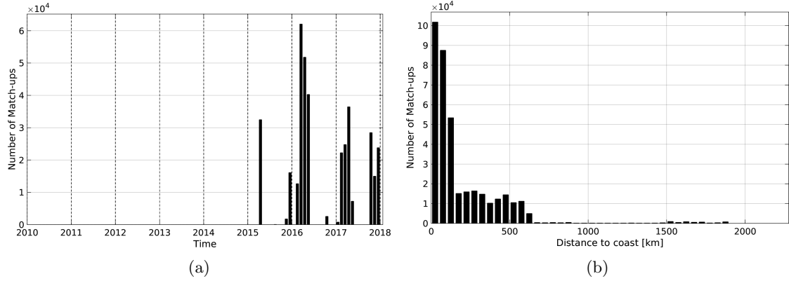
Figure 1: Number of match-ups between TSG-SAMOS and SMAP-L3-JPL-V4-8DAY-RUNNING-60KM SSS as a function of time (a) and as function of the distance to coast (b) over the South Pacific Ocean Pi-MEP region and for the full satellite product period.
