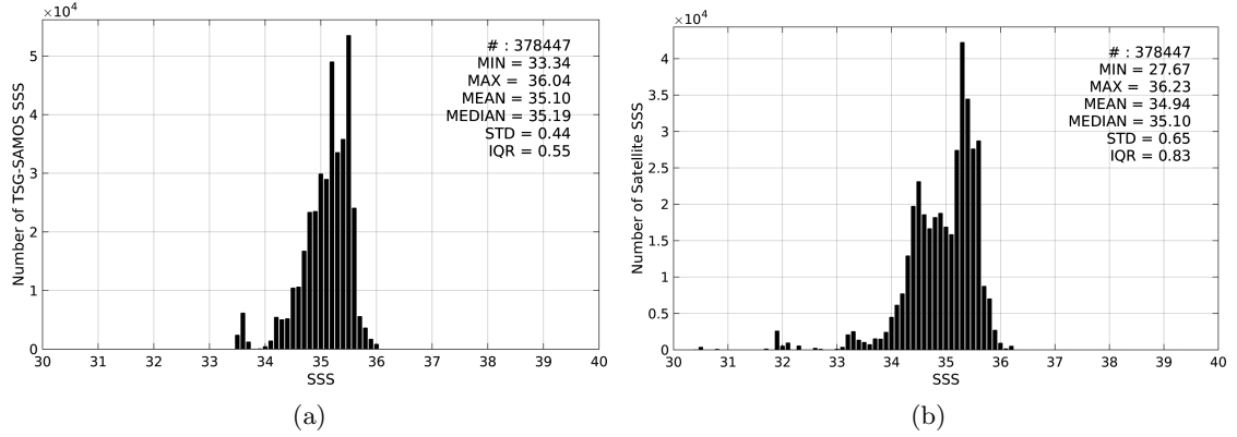
Figure 2: Histograms of SSS from TSG-SAMOS (a) and SMAP-L3-JPL-V4-8DAY-RUNNING-60KM (b) considering all match-up pairs per bins of 0.1 over the South Pacific Ocean Pi-MEP region and for the full satellite product period.
