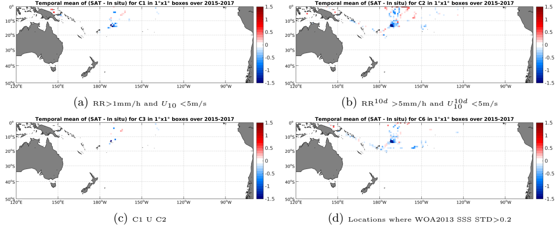
Figure 12: Temporal mean gridded over spatial boxes of size 1^\circ \times 1^\circ of \Delta SSS (SMAP-L3-JPL-V4-8DAY-RUNNING-60KM - TSG-SAMOS) for 4 different subdatasets corresponding to: RR > 1 mm/h and U_{10} < 5 m/s (a), RR^{10d} > 5 mm/h and U_{10}^{10d} < 5 m/s (b), C1 U C2 (c), Locations where WOA2013 SSS STD > 0.2 (d).
