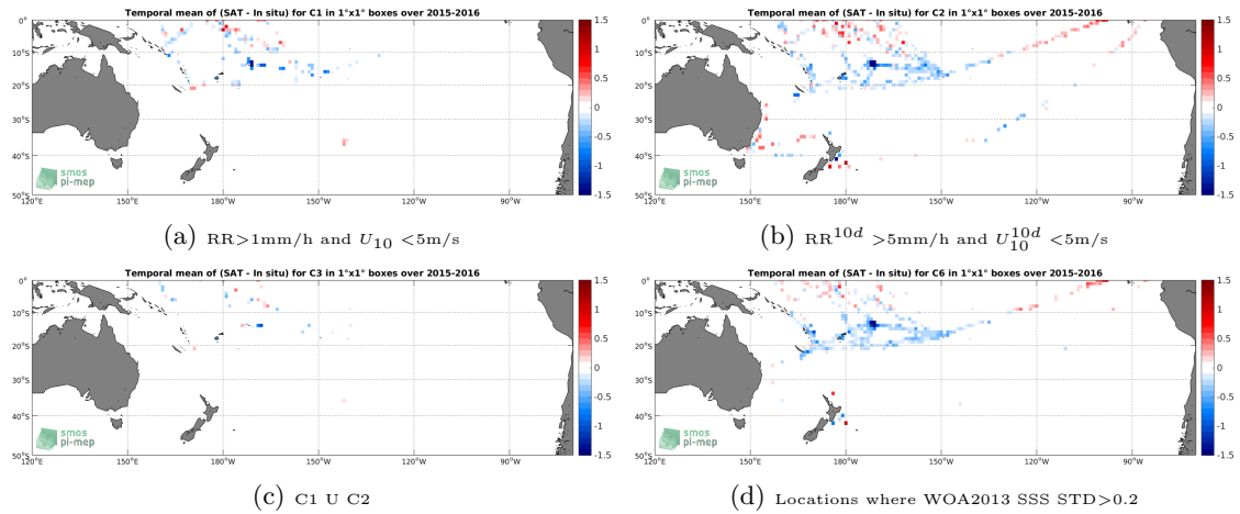
Figure 12: Temporal mean gridded over spatial boxes of size 1^\circ \times 1^\circ of \Delta SSS (SMAP-L3-JPL-V4-8DAY-RUNNING-60KM - TSG-LEGOS-DM) for 4 different subdatasets corresponding to: RR > 1\text{mm/h} and U_{10} < 5\text{m/s} (a), RR^{10d} > 5\text{mm/h} and U_{10}^{10d} < 5\text{m/s} (b), C1 U C2 (c), Locations where WOA2013 SSS STD > 0.2 (d).
