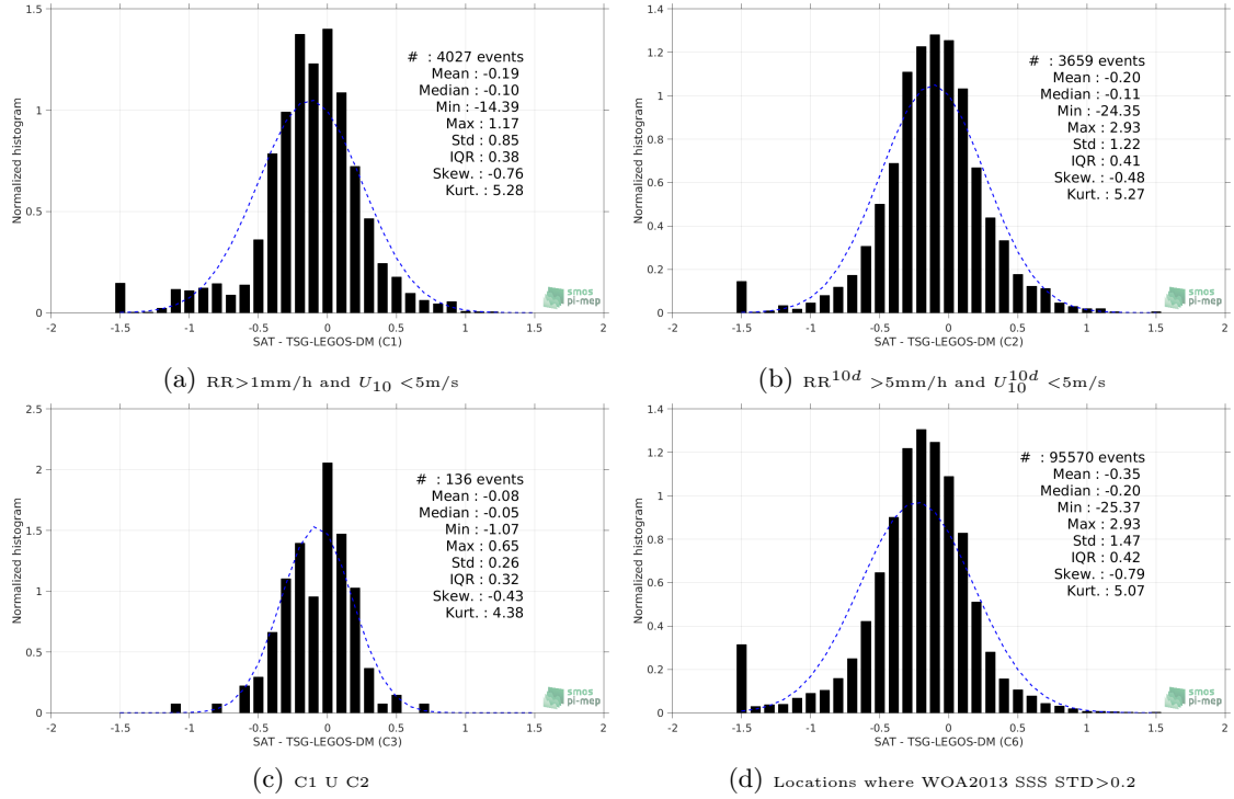
Figure 13: Normalized histogram of \Delta SSS (SMAP-L3-JPL-V4-8DAY-RUNNING-60KM - TSG-LEGOS-DM) for 6 different subdatasets corresponding to: RR > 1mm/h and U_{10} < 5 m/s (a), RR^{10d} > 5 mm/h and U_{10}^{10d} < 5 m/s (b), C1 U C2 (c), Locations where WOA2013 SSS STD > 0.2 (d).
