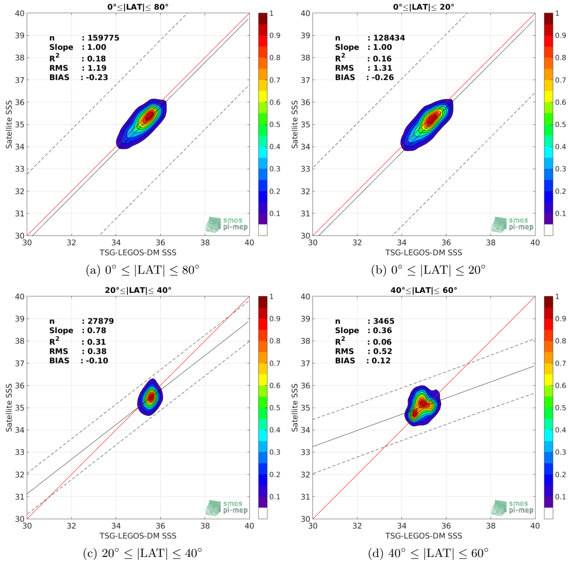
Figure 9: Contour maps of the concentration of SMAP-L3-JPL-V4-8DAY-RUNNING-60KM SSS (y-axis) versus TSG-LEGOS-DM SSS (x-axis) at match-up pairs for different latitude bands. For each plot, the red line shows x=y . The black thin and dashed lines indicate a linear fit through the data cloud and the \pm 95\% confidence levels, respectively. The number match-up pairs n , the slope and R^2 coefficient of the linear fit, the root mean square (RMS) and the mean bias between satellite and in situ data are indicated for each latitude band in each plots.
