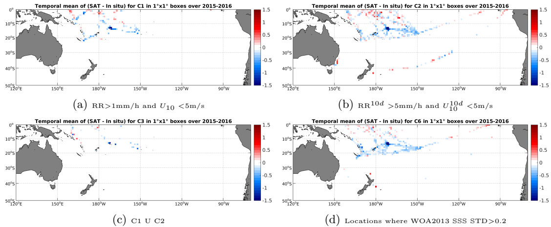
Figure 12: Temporal mean gridded over spatial boxes of size 1^\circ \times 1^\circ of \Delta SSS (SMAP-L3-JPL-V4-8DAY-RUNNING-60KM - TSG-LEGOS-DM) for 4 different subdatasets corresponding to:RR > 1 mm/h and U_{10} < 5 m/s (a), RR 10d > 5 mm/h and U_{10}^{10d} < 5 m/s (b), C1 U C2 (c),Locations where WOA2013 SSS STD > 0.2 (d).
