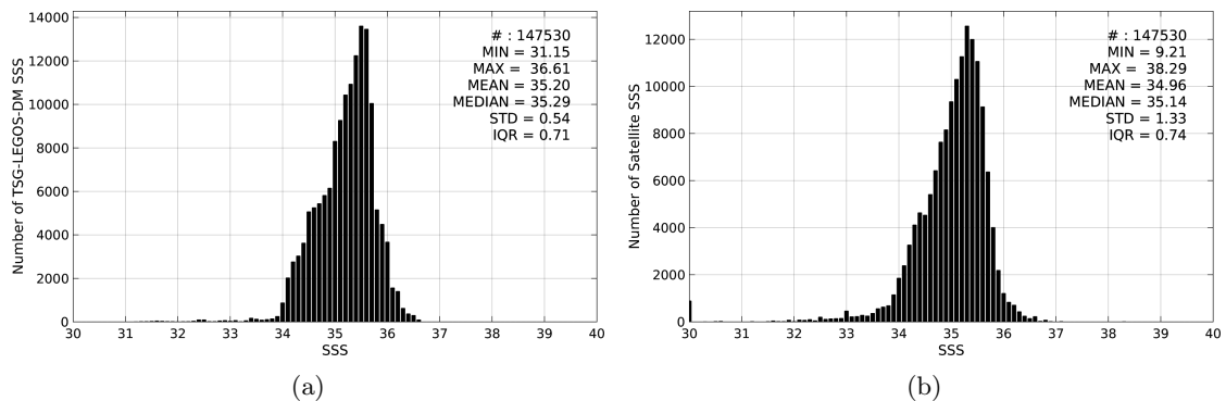
Figure 2: Histograms of SSS from TSG-LEGOS-DM (a) and SMAP-L3-JPL-V4-8DAY-RUNNING-60KM (b) considering all match-up pairs per bins of 0.1 over the South Pacific Ocean Pi-MEP region and for the full satellite product period.
