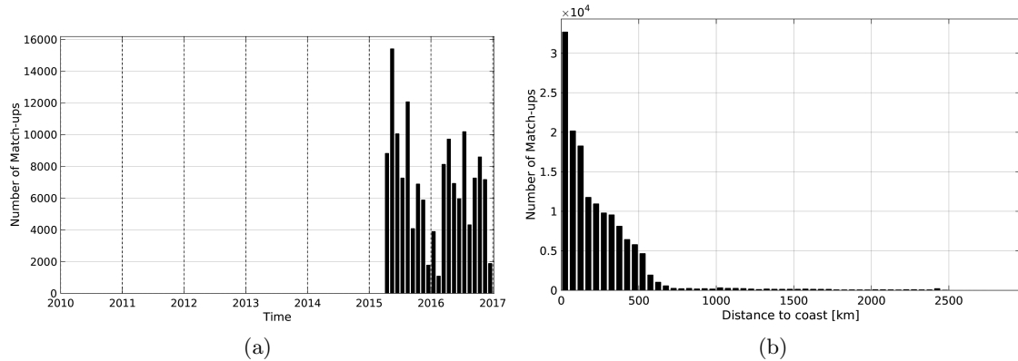
Figure 1: Number of match-ups between TSG-LEGOS-DM and SMAP-L3-JPL-V4-8DAY-RUNNING-60KM SSS as a function of time (a) and as function of the distance to coast (b) over the South Pacific Ocean Pi-MEP region and for the full satellite product period.
