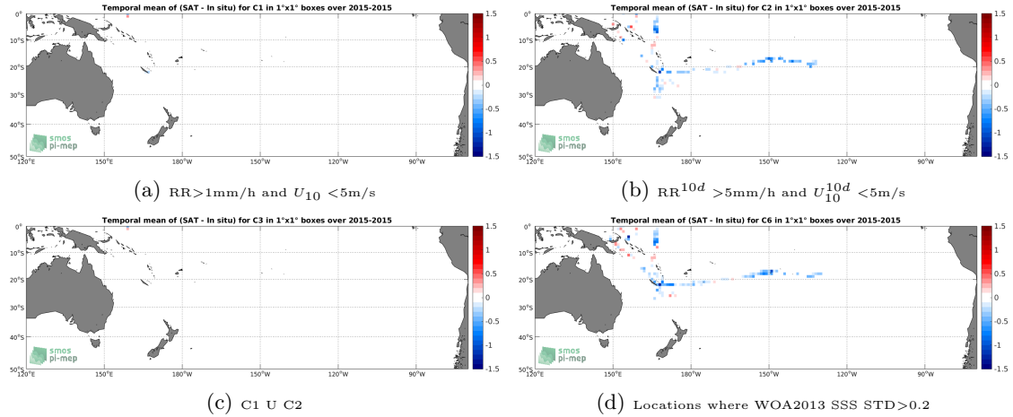
Figure 12: Temporal mean gridded over spatial boxes of size 1^\circ \times 1^\circ of \Delta SSS (SMAP-L3-JPL-V4-8DAY-RUNNING-60KM - TSG-GOSUD-Research-vessel) for 4 different subdatasets corresponding to: RR > 1\text{mm/h} and U_{10} < 5\text{m/s} (a), RR^{10d} > 5\text{mm/h} and U_{10}^{10d} < 5\text{m/s} (b), C1 U C2 (c), Locations where WOA2013 SSS STD > 0.2 (d).
