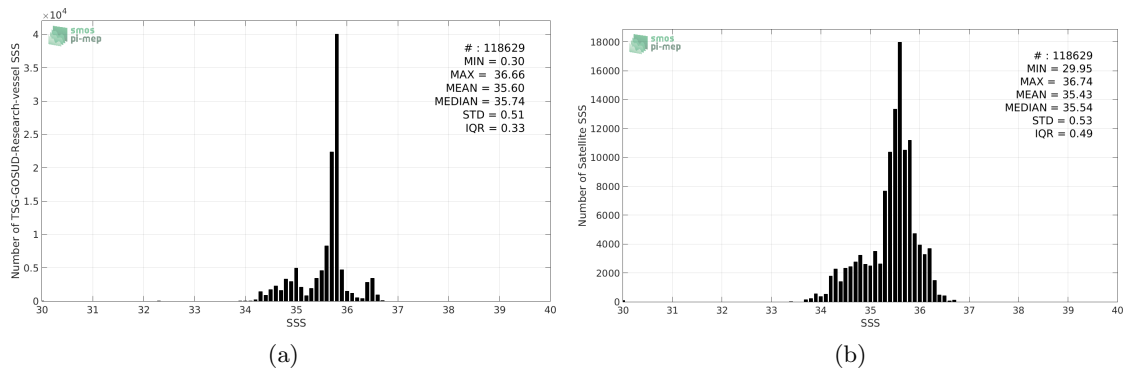
Figure 2: Histograms of SSS from TSG-GOSUD-Research-vessel (a) and SMAP-L3-JPL-V4-8DAY-RUNNING-60KM (b) considering all match-up pairs per bins of 0.1 over the South Pacific Ocean Pi-MEP region and for the full satellite product period.
