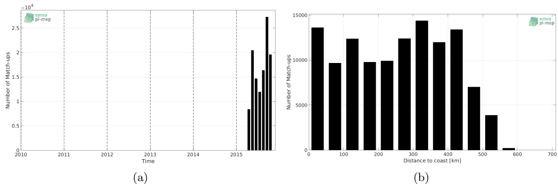
Figure 1: Number of match-ups between TSG-GOSUD-Research-vessel and SMAP-L3-JPL-V4-8DAY-RUNNING-60KM SSS as a function of time (a) and as function of the distance to coast (b) over the South Pacific Ocean Pi-MEP region and for the full satellite product period.
