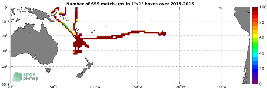
Figure 4: Number of SSS match-ups between TSG-GOSUD-Research-vessel SSS and the SMAP-L3-JPL-V4-8DAY-RUNNING-60KM SSS product for the South Pacific Ocean Pi-MEP region over 1^\circ \times 1^\circ boxes and for the full satellite product period.
