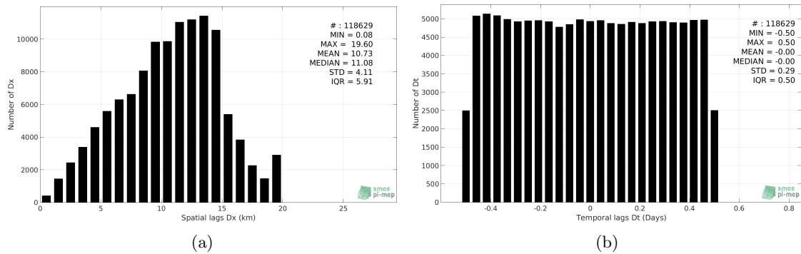
Figure 5: Histograms of the spatial (a) and temporal (b) lags between the time of the TSG-GOSUD-Research-vessel measurements and the date of the corresponding SMAP-L3-JPL-V4-8DAY-RUNNING-60KM SSS product.
