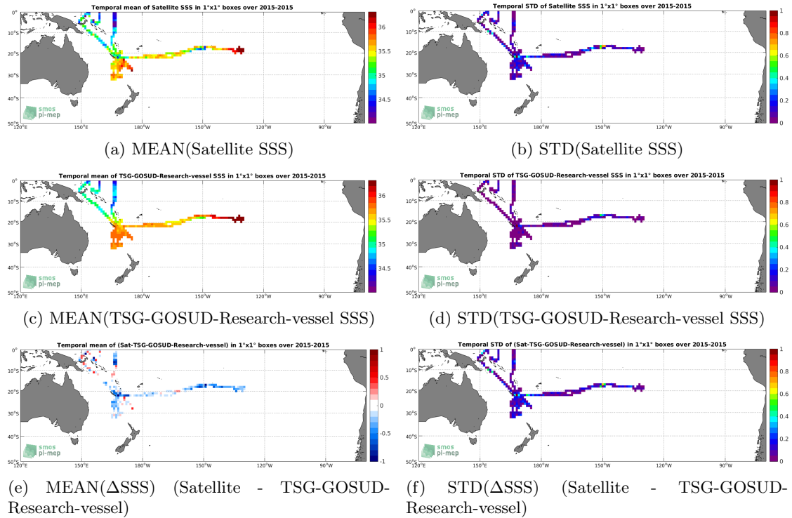
Figure 6: Temporal mean (left) and STD (right) of SSS from SMAP-L3-JPL-V4-8DAY-RUNNING-60KM (top), TSG-GOSUD-Research-vessel (middle), and of \Delta SSS (Satellite - TSG-GOSUD-Research-vessel). Only match-up pairs are used to generate these maps.
