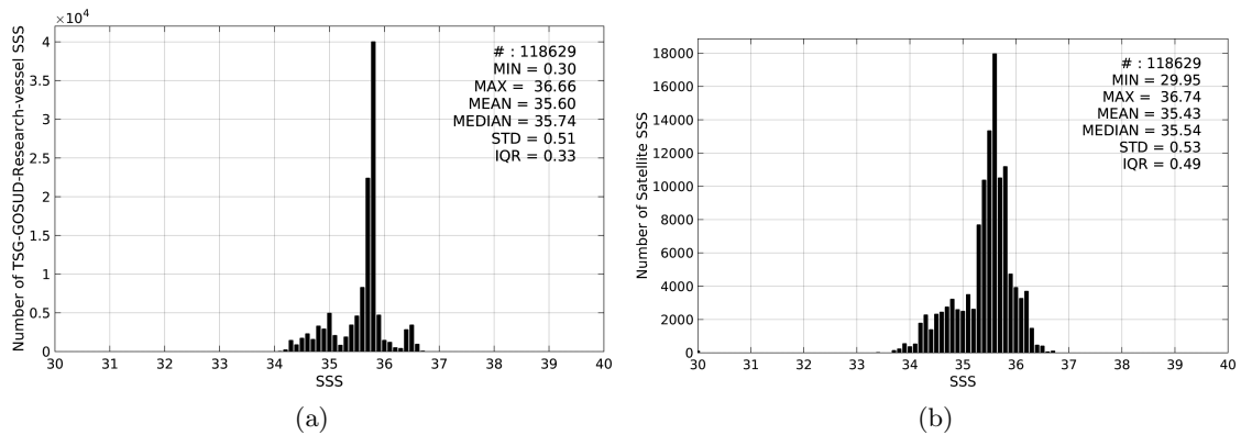
Figure 2: Histograms of SSS from TSG-GOSUD-Research-vessel (a) and SMAP-L3-JPL-V4-8DAY-RUNNING-60KM (b) considering all match-up pairs per bins of 0.1 over the South Pacific Ocean Pi-MEP region and for the full satellite product period.
