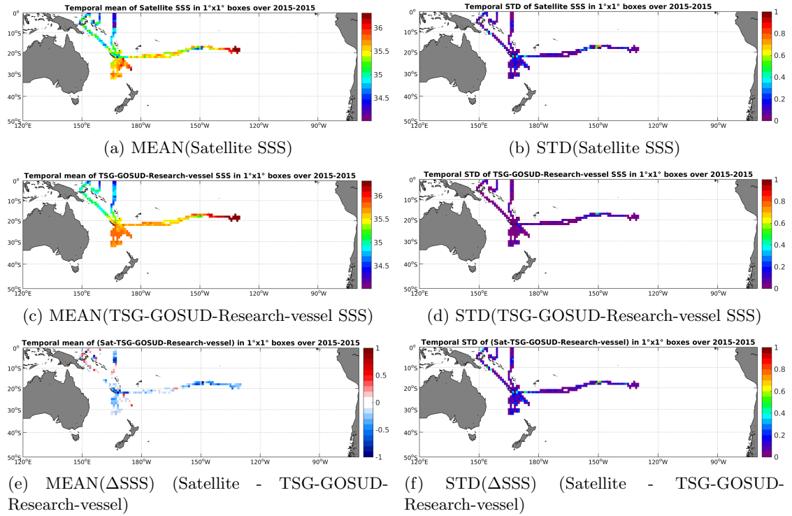
Figure 6: Temporal mean (left) and STD (right) of SSS from SMAP-L3-JPL-V4-8DAY-RUNNING-60KM (top), TSG-GOSUD-Research-vessel (middle), and of \Delta SSS (Satellite - TSG-GOSUD-Research-vessel). Only match-up pairs are used to generate these maps.
