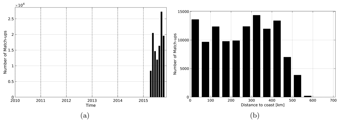
Figure 1: Number of match-ups between TSG-GOSUD-Research-vessel and SMAP-L3-JPL-V4-8DAY-RUNNING-60KM SSS as a function of time (a) and as function of the distance to coast (b) over the South Pacific Ocean Pi-MEP region and for the full satellite product period.
