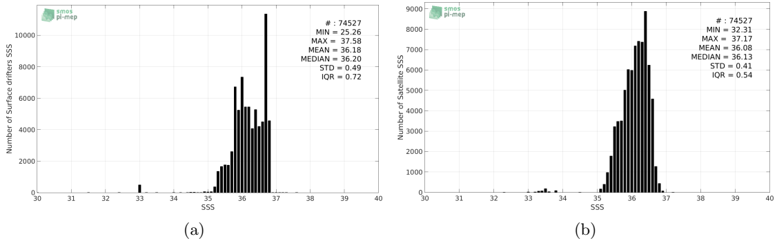
Figure 2: Histograms of SSS from Surface drifters (a) and SMAP-L3-JPL-V4-8DAY-RUNNING-60KM (b) considering all match-up pairs per bins of 0.1 over the South Pacific Ocean Pi-MEP region and for the full satellite product period.
