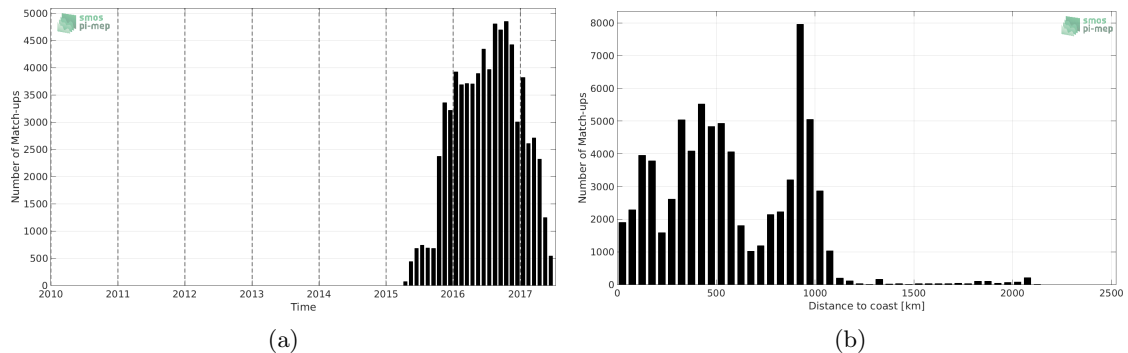
Figure 1: Number of match-ups between Surface drifters and SMAP-L3-JPL-V4-8DAY-RUNNING-60KM SSS as a function of time (a) and as function of the distance to coast (b) over the South Pacific Ocean Pi-MEP region and for the full satellite product period.
