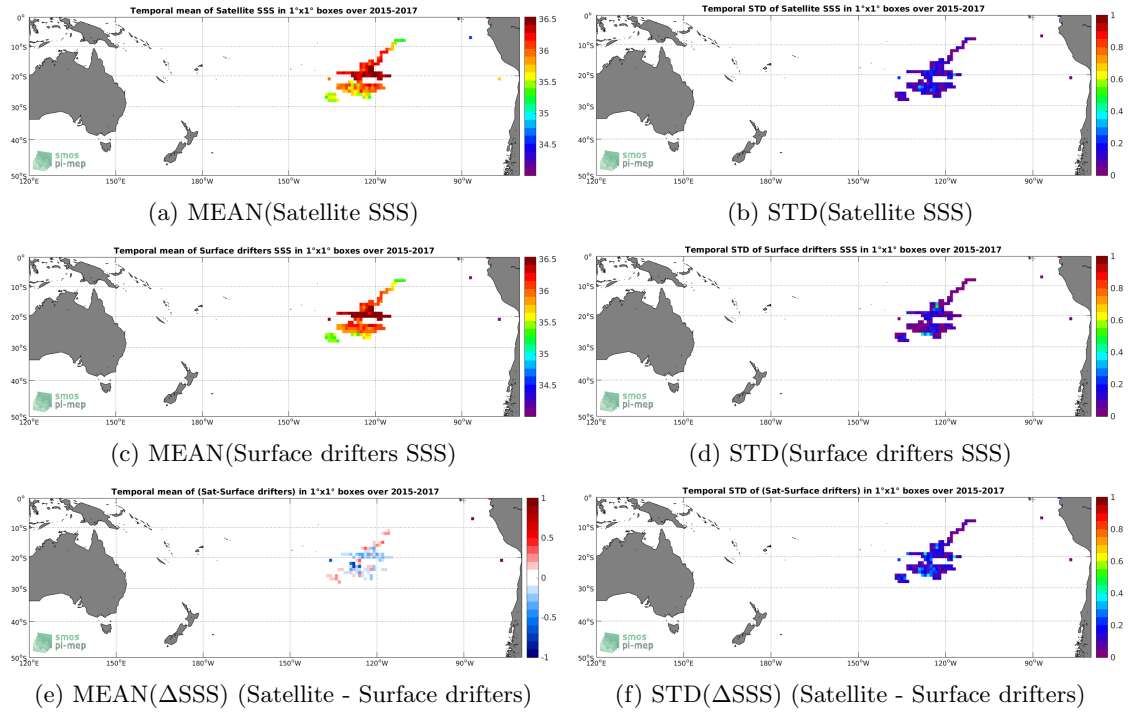
Figure 5: Temporal mean (left) and STD (right) of SSS from SMAP-L3-JPL-V4-8DAY-RUNNING-60KM (top), Surface drifters (middle), and of \Delta SSS (Satellite - Surface drifters). Only match-up pairs are used to generate these maps.
