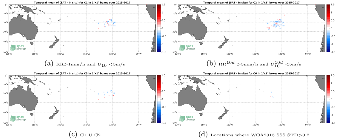
Figure 11: Temporal mean gridded over spatial boxes of size 1^\circ \times 1^\circ of \Delta SSS (SMAP-L3-JPL-V4-8DAY-RUNNING-60KM - Surface drifters) for 4 different subdatasets corresponding to: RR > 1\text{mm/h} and U_{10} < 5\text{m/s} (a), RR^{10d} > 5\text{mm/h} and U_{10}^{10d} < 5\text{m/s} (b), C1 U C2 (c), Locations where WOA2013 SSS STD > 0.2 (d).
