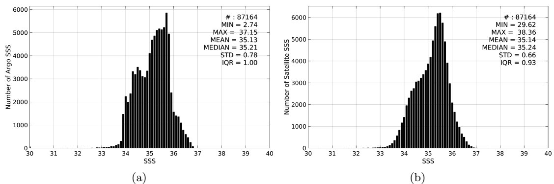
Figure 2: Histograms of SSS from Argo (a) and SMAP-L3-JPL-V4-8DAY-RUNNING-60KM (b) considering all match-up pairs per bins of 0.1 over the South Pacific Ocean Pi-MEP region and for the full satellite product period.
