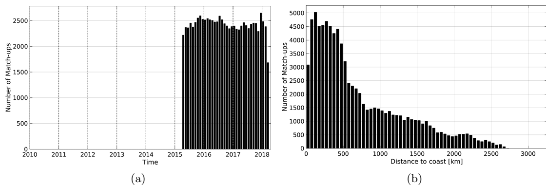
Figure 1: Number of match-ups between Argo and SMAP-L3-JPL-V4-8DAY-RUNNING-60KM SSS as a function of time (a) and as function of the distance to coast (b) over the South Pacific Ocean Pi-MEP region and for the full satellite product period.
