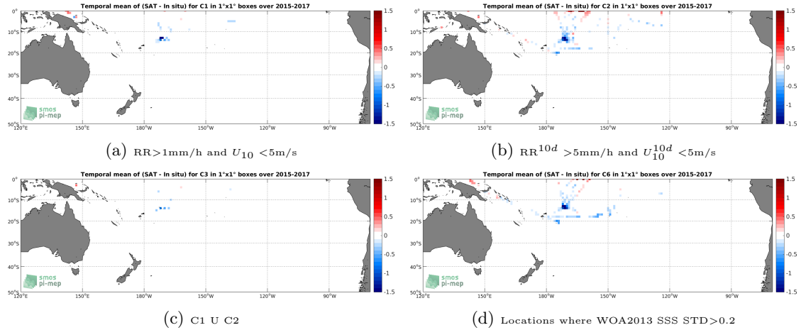
Figure 12: Temporal mean gridded over spatial boxes of size 1^\circ \times 1^\circ of \Delta SSS (SMAP-L3-JPL-V4-MONTHLY-60KM - TSG-SAMOS) for 4 different subdatasets corresponding to: RR > 1mm/h and U_{10} < 5\text{m/s} (a), RR^{10d} > 5\text{mm/h} and U_{10}^{10d} < 5\text{m/s} (b), C1 U C2 (c), Locations where WOA2013 SSS STD > 0.2 (d).
