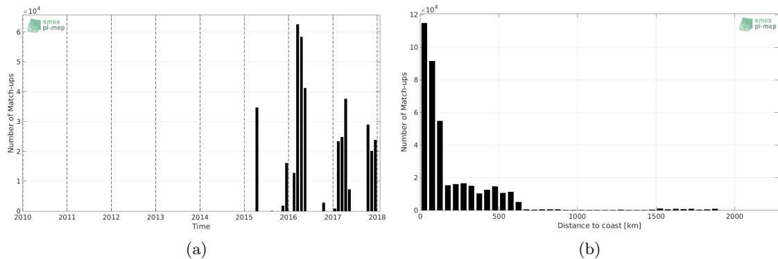
Figure 1: Number of match-ups between TSG-SAMOS and SMAP-L3-JPL-V4-MONTHLY-60KM SSS as a function of time (a) and as function of the distance to coast (b) over the South Pacific Ocean Pi-MEP region and for the full satellite product period.
