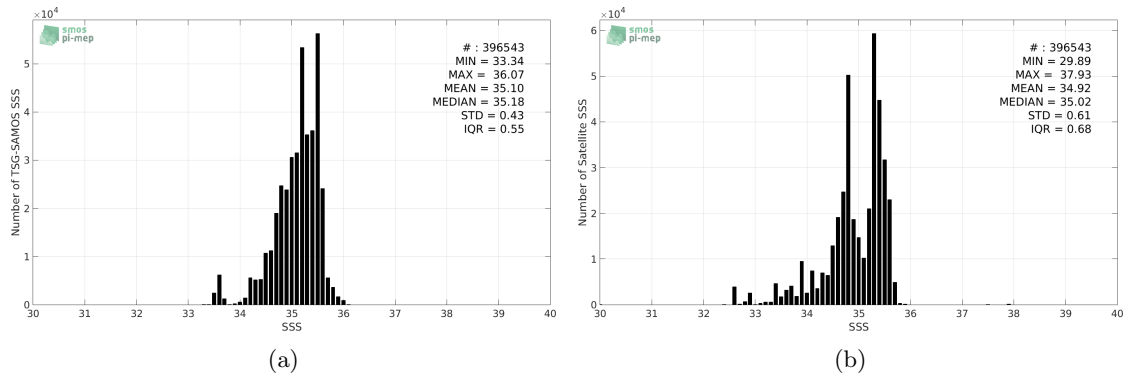
Figure 2: Histograms of SSS from TSG-SAMOS (a) and SMAP-L3-JPL-V4-MONTHLY-60KM (b) considering all match-up pairs per bins of 0.1 over the South Pacific Ocean Pi-MEP region and for the full satellite product period.
