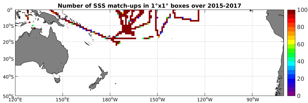
Figure 4: Number of SSS match-ups between TSG-SAMOS SSS and the SMAP-L3-JPL-V4-MONTHLY-60KM SSS product for the South Pacific Ocean Pi-MEP region over 1^\circ \times 1^\circ boxes and for the full satellite product period.
