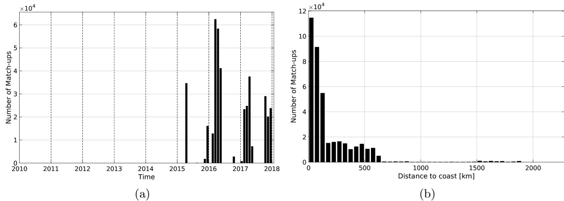
Figure 1: Number of match-ups between TSG-SAMOS and SMAP-L3-JPL-V4-MONTHLY-60KM SSS as a function of time (a) and as function of the distance to coast (b) over the South Pacific Ocean Pi-MEP region and for the full satellite product period.
