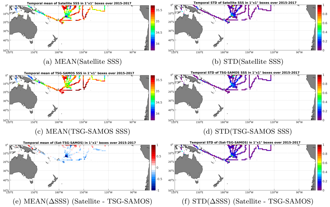
Figure 6: Temporal mean (left) and STD (right) of SSS from SMAP-L3-JPL-V4-MONTHLY-60KM (top), TSG-SAMOS (middle), and of \Delta SSS (Satellite - TSG-SAMOS). Only match-up pairs are used to generate these maps.
