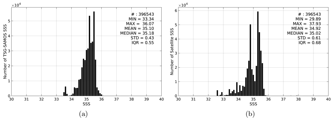
Figure 2: Histograms of SSS from TSG-SAMOS (a) and SMAP-L3-JPL-V4-MONTHLY-60KM (b) considering all match-up pairs per bins of 0.1 over the South Pacific Ocean Pi-MEP region and for the full satellite product period.
