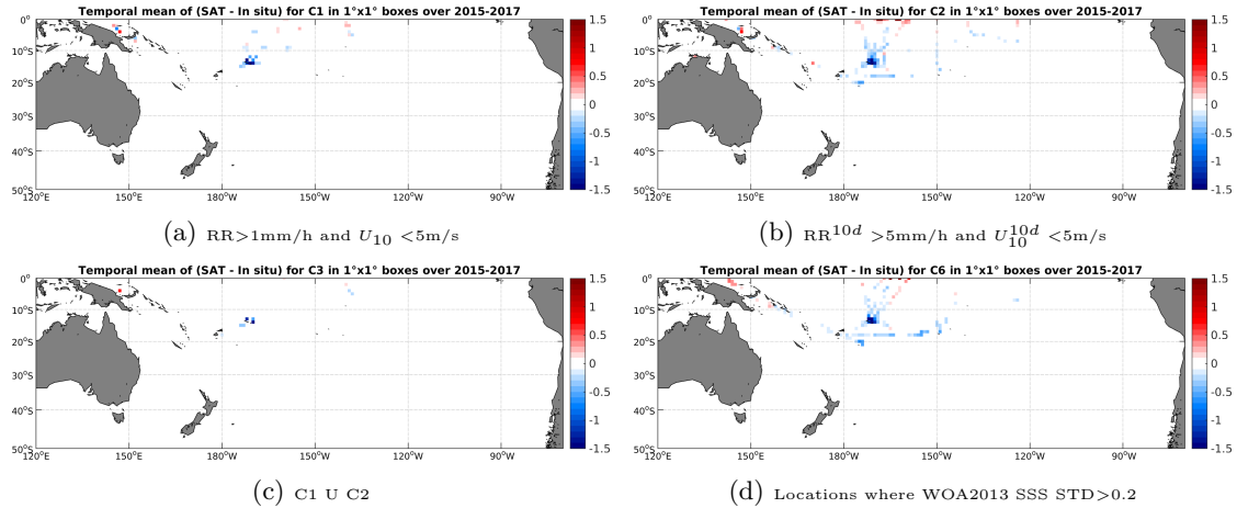
Figure 12: Temporal mean gridded over spatial boxes of size 1^\circ \times 1^\circ of \Delta SSS (SMAP-L3-JPL-V4-MONTHLY-60KM - TSG-SAMOS) for 4 different subdatasets corresponding to: RR > 1\text{mm/h} and U_{10} < 5\text{m/s} (a), RR^{10d} > 5\text{mm/h} and U_{10}^{10d} < 5\text{m/s} (b), C1 U C2 (c), Locations where WOA2013 SSS STD > 0.2 (d).
