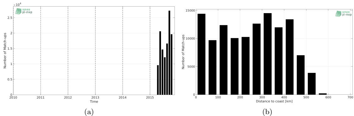
Figure 1: Number of match-ups between TSG-GOSUD-Research-vessel and SMAP-L3-JPL-V4-MONTHLY-60KM SSS as a function of time (a) and as function of the distance to coast (b) over the South Pacific Ocean Pi-MEP region and for the full satellite product period.
