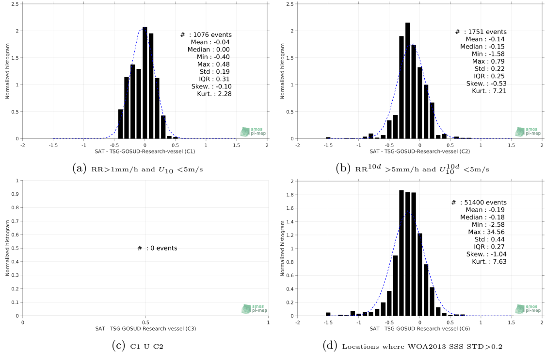
Figure 13: Normalized histogram of \Delta\text{SSS} (SMAP-L3-JPL-V4-MONTHLY-60KM - TSG-GOSUD-Research-vessel) for 6 different subdatasets corresponding to: RR > 1mm/h and U_{10} < 5\text{m/s} (a), RR^{10d} > 5\text{mm/h} and U_{10}^{10d} < 5\text{m/s} (b), C1 U C2 (c), Locations where WOA2013 SSS STD > 0.2 (d).
