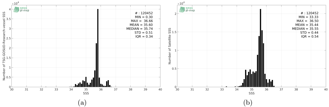
Figure 2: Histograms of SSS from TSG-GOSUD-Research-vessel (a) and SMAP-L3-JPL-V4-MONTHLY-60KM (b) considering all match-up pairs per bins of 0.1 over the South Pacific Ocean Pi-MEP region and for the full satellite product period.
