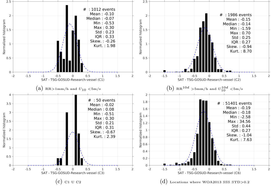
Figure 13: Normalized histogram of \Delta SSS (SMAP-L3-JPL-V4-MONTHLY-60KM - TSG-GOSUD-Research-vessel) for 6 different subdatasets corresponding to: RR > 1\text{mm/h} and U_{10} < 5\text{m/s} (a), RR^{10d} > 5\text{mm/h} and U_{10}^{10d} < 5\text{m/s} (b), C1 U C2 (c), Locations where WOA2013 SSS STD > 0.2 (d).
