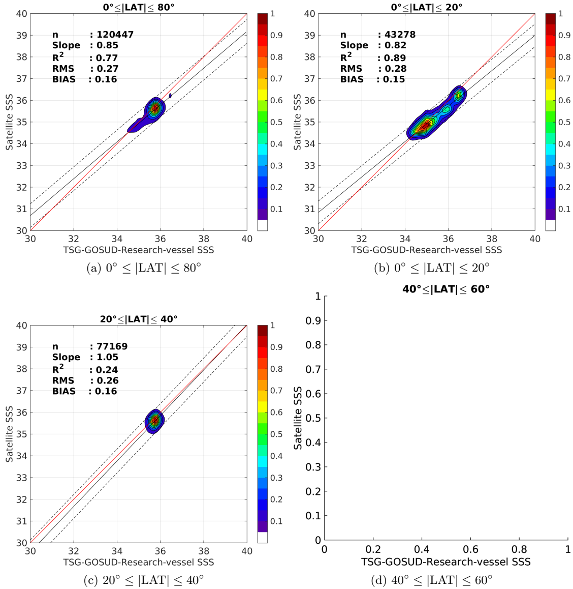
Figure 9: Contour maps of the concentration of SMAP-L3-JPL-V4-MONTHLY-60KM SSS (y-axis) versus TSG-GOSUD-Research-vessel SSS (x-axis) at match-up pairs for different latitude bands. For each plot, the red line shows x=y . The black thin and dashed lines indicate a linear fit through the data cloud and the \pm 95\% confidence levels, respectively. The number match-up pairs n , the slope and R^2 coefficient of the linear fit, the root mean square (RMS) and the mean bias between satellite and in situ data are indicated for each latitude band in each plots.
