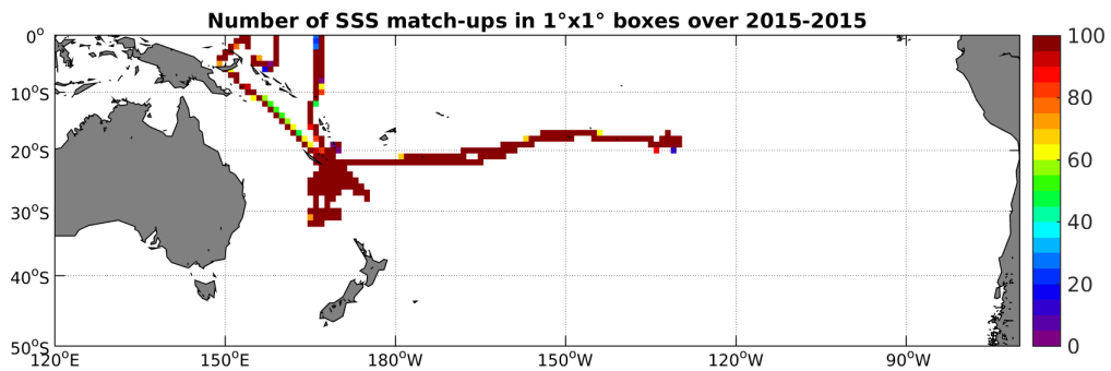
Figure 4: Number of SSS match-ups between TSG-GOSUD-Research-vessel SSS and the SMAP-L3-JPL-V4-MONTHLY-60KM SSS product for the South Pacific Ocean Pi-MEP region over 1^\circ \times 1^\circ boxes and for the full satellite product period.
