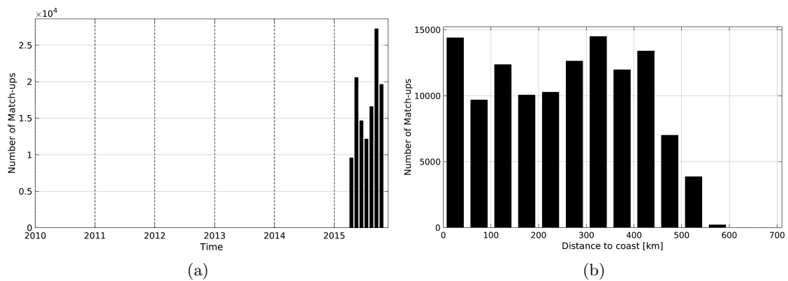
Figure 1: Number of match-ups between TSG-GOSUD-Research-vessel and SMAP-L3-JPL-V4-MONTHLY-60KM SSS as a function of time (a) and as function of the distance to coast (b) over the South Pacific Ocean Pi-MEP region and for the full satellite product period.
