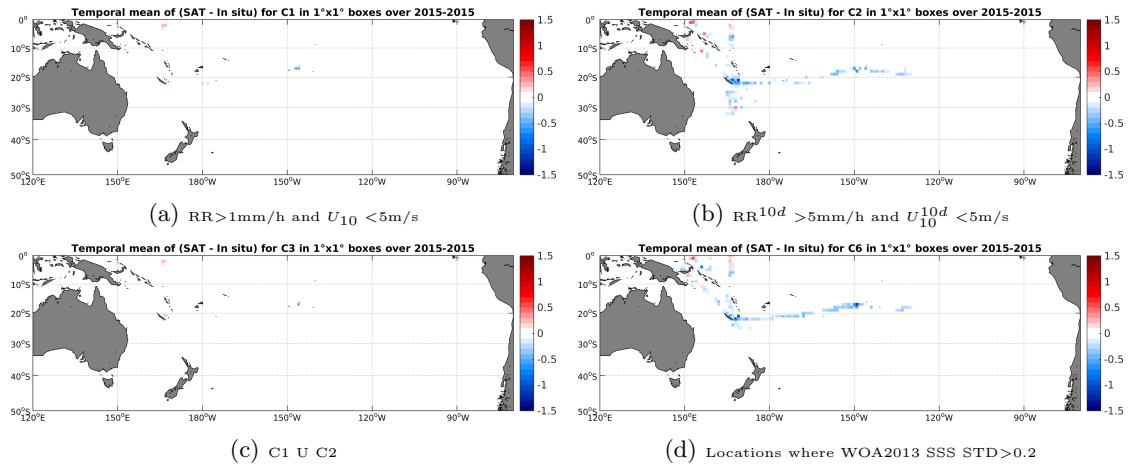
Figure 12: Temporal mean gridded over spatial boxes of size 1^\circ \times 1^\circ of \Delta SSS (SMAP-L3-JPL-V4-MONTHLY-60KM - TSG-GOSUD-Research-vessel) for 4 different subdatasets corresponding to: RR > 1mm/h and U_{10} < 5\text{m/s} (a), RR^{10d} > 5\text{mm/h} and U_{10}^{10d} < 5\text{m/s} (b), C1 U C2 (c), Locations where WOA2013 SSS STD > 0.2 (d).
