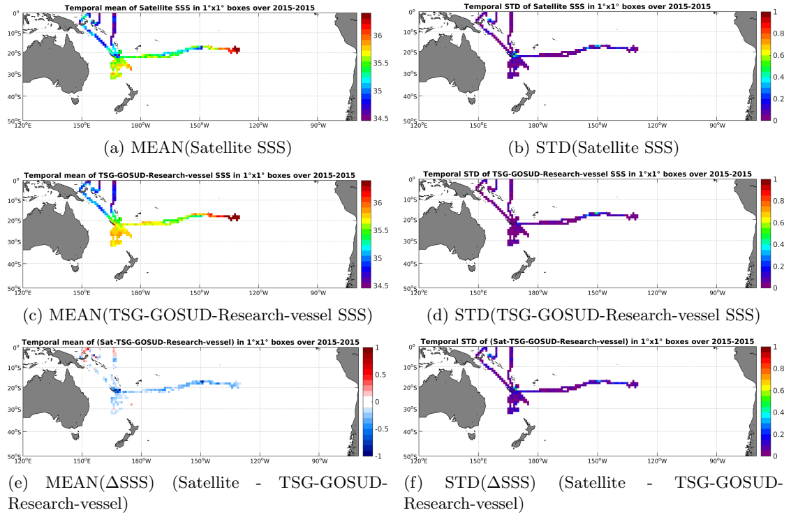
Figure 6: Temporal mean (left) and STD (right) of SSS from SMAP-L3-JPL-V4-MONTHLY-60KM (top), TSG-GOSUD-Research-vessel (middle), and of \Delta SSS (Satellite - TSG-GOSUD-Research-vessel). Only match-up pairs are used to generate these maps.
