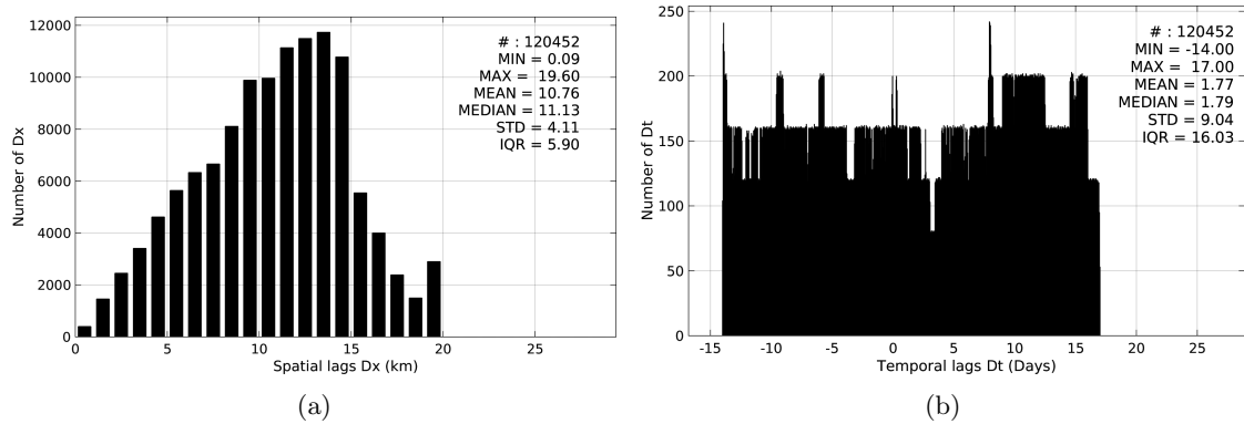
Figure 5: Histograms of the spatial (a) and temporal (b) lags between the time of the TSG-GOSUD-Research-vessel measurements and the date of the corresponding SMAP-L3-JPL-V4-MONTHLY-60KM SSS product.
