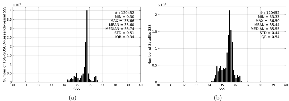
Figure 2: Histograms of SSS from TSG-GOSUD-Research-vessel (a) and SMAP-L3-JPL-V4-MONTHLY-60KM (b) considering all match-up pairs per bins of 0.1 over the South Pacific Ocean Pi-MEP region and for the full satellite product period.
