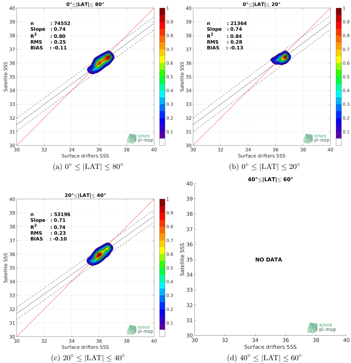
Figure 8: Contour maps of the concentration of SMAP-L3-JPL-V4-MONTHLY-60KM SSS (y-axis) versus Surface drifters SSS (x-axis) at match-up pairs for different latitude bands. For each plot, the red line shows x=y . The black thin and dashed lines indicate a linear fit through the data cloud and the \pm 95\% confidence levels, respectively. The number match-up pairs n , the slope and R^2 coefficient of the linear fit, the root mean square (RMS) and the mean bias between satellite and in situ data are indicated for each latitude band in each plots.
