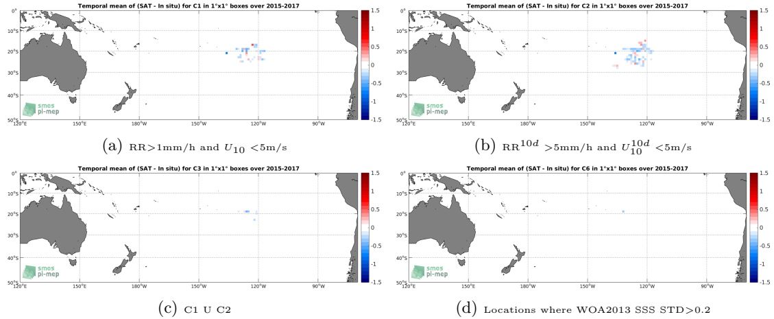
Figure 11: Temporal mean gridded over spatial boxes of size 1^\circ \times 1^\circ of \Delta SSS (SMAP-L3-JPL-V4-MONTHLY-60KM - Surface drifters) for 4 different subdatasets corresponding to: RR > 1 mm/h and U_{10} < 5 m/s (a), RR 10d > 5 mm/h and U_{10}^{10d} < 5 m/s (b), C1 U C2 (c), Locations where WOA2013 SSS STD > 0.2 (d).
