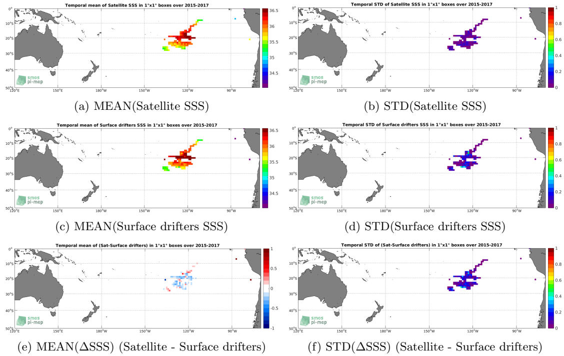
Figure 5: Temporal mean (left) and STD (right) of SSS from SMAP-L3-JPL-V4-MONTHLY-60KM (top), Surface drifters (middle), and of \Delta SSS (Satellite - Surface drifters). Only match-up pairs are used to generate these maps.
