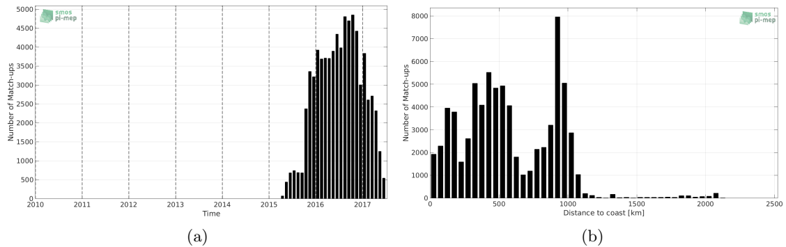
Figure 1: Number of match-ups between Surface drifters and SMAP-L3-JPL-V4-MONTHLY-60KM SSS as a function of time (a) and as function of the distance to coast (b) over the South Pacific Ocean Pi-MEP region and for the full satellite product period.
