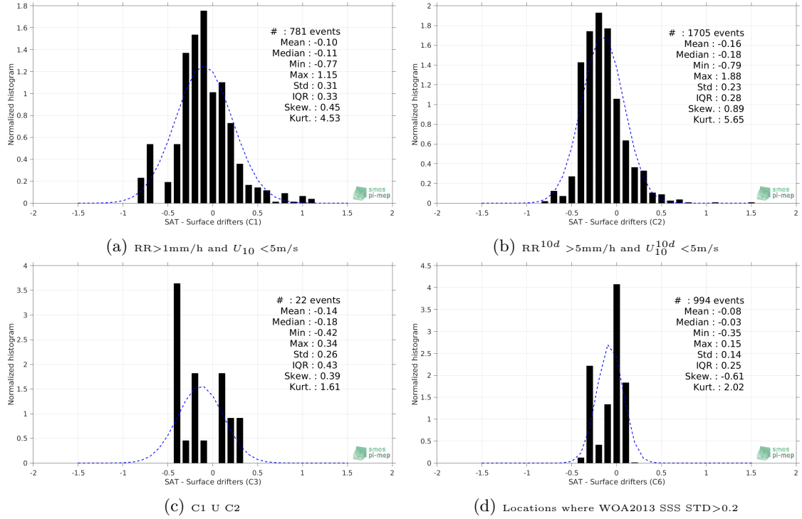
Figure 12: Normalized histogram of \Delta SSS (SMAP-L3-JPL-V4-MONTHLY-60KM - Surface drifters) for 6 different subdatasets corresponding to: RR > 1\text{mm/h} and U_{10} < 5\text{m/s} (a), RR^{10d} > 5\text{mm/h} and U_{10}^{10d} < 5\text{m/s} (b), C1 U C2 (c), Locations where WOA2013 SSS STD > 0.2 (d).
