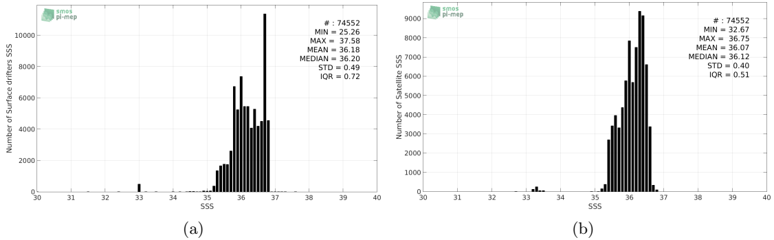
Figure 2: Histograms of SSS from Surface drifters (a) and SMAP-L3-JPL-V4-MONTHLY-60KM (b) considering all match-up pairs per bins of 0.1 over the South Pacific Ocean Pi-MEP region and for the full satellite product period.
