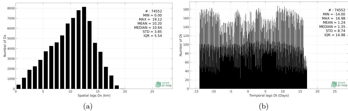
Figure 4: Histograms of the spatial (a) and temporal (b) lags between the time of the Surface drifters measurements and the date of the corresponding SMAP-L3-JPL-V4-MONTHLY-60KM SSS product.
