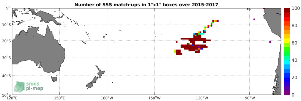
Figure 3: Number of SSS match-ups between Surface drifters SSS and the SMAP-L3-JPL-V4-MONTHLY-60KM SSS product for the South Pacific Ocean Pi-MEP region over 1°x1° boxes and for the full satellite product period.
