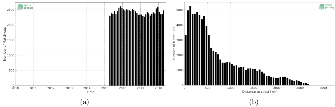
Figure 1: Number of match-ups between Argo and SMAP-L3-JPL-V4-MONTHLY-60KM SSS as a function of time (a) and as function of the distance to coast (b) over the South Pacific Ocean Pi-MEP region and for the full satellite product period.
