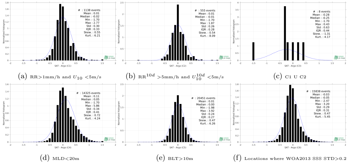
Figure 13: Normalized histogram of \Delta\text{SSS} (SMAP-L3-JPL-V4-MONTHLY-60KM - Argo) for 6 different subdatasets corresponding to: RR > 1\text{mm/h} and U_{10} < 5\text{m/s} (a), RR^{10d} > 5\text{mm/h} and U_{10}^{10d} < 5\text{m/s} (b), C1 U C2 (c), MLD < 20\text{m} (d), BLT > 10\text{m} (e), Locations where WOA2013 SSS STD > 0.2 (f).
