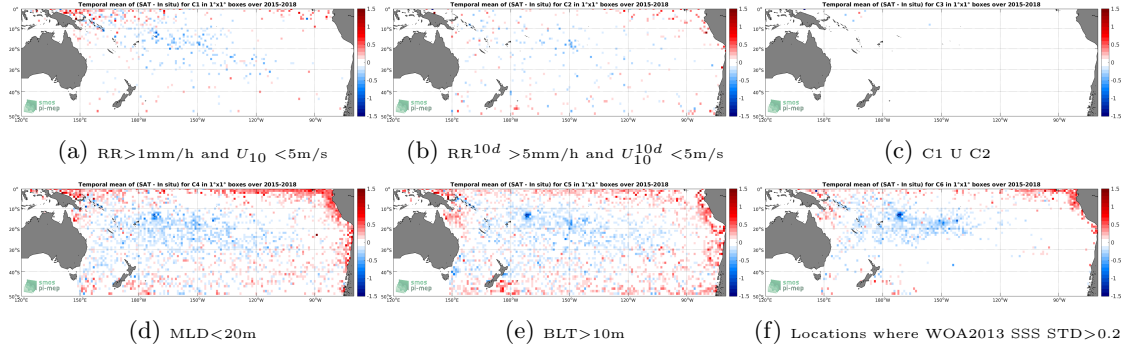
Figure 12: Temporal mean gridded over spatial boxes of size 1^\circ \times 1^\circ of \Delta\text{SSS} (SMAP-L3-JPL-V4-MONTHLY-60KM - Argo) for 6 different subdatasets corresponding to: RR > 1\text{mm/h} and U_{10} < 5\text{m/s} (a), RR^{10d} > 5\text{mm/h} and U_{10}^{10d} < 5\text{m/s} (b), C1 U C2 (c), MLD < 20\text{m} (d), BLT > 10\text{m} (e), Locations where WOA2013 SSS STD > 0.2 (f).
