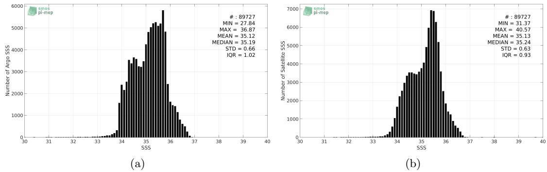
Figure 2: Histograms of SSS from Argo (a) and SMAP-L3-JPL-V4-MONTHLY-60KM (b) considering all match-up pairs per bins of 0.1 over the South Pacific Ocean Pi-MEP region and for the full satellite product period.
