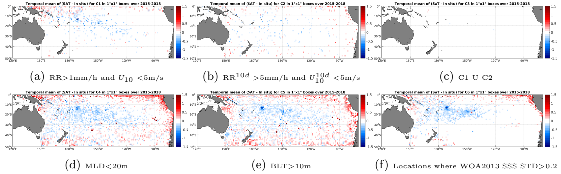
Figure 12: Temporal mean gridded over spatial boxes of size 1^\circ \times 1^\circ of \Delta SSS (SMAP-L3-JPL-V4-MONTHLY-60KM - Argo) for 6 different subdatasets corresponding to: RR > 1\text{mm/h} and U_{10} < 5\text{m/s} (a), RR^{10d} > 5\text{mm/h} and U_{10}^{10d} < 5\text{m/s} (b), C1 U C2 (c), MLD < 20\text{m} (d), BLT > 10\text{m} (e), Locations where WOA2013 SSS STD > 0.2 (f).
