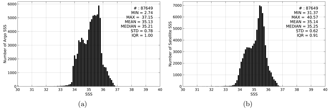
Figure 2: Histograms of SSS from Argo (a) and SMAP-L3-JPL-V4-MONTHLY-60KM (b) considering all match-up pairs per bins of 0.1 over the South Pacific Ocean Pi-MEP region and for the full satellite product period.
