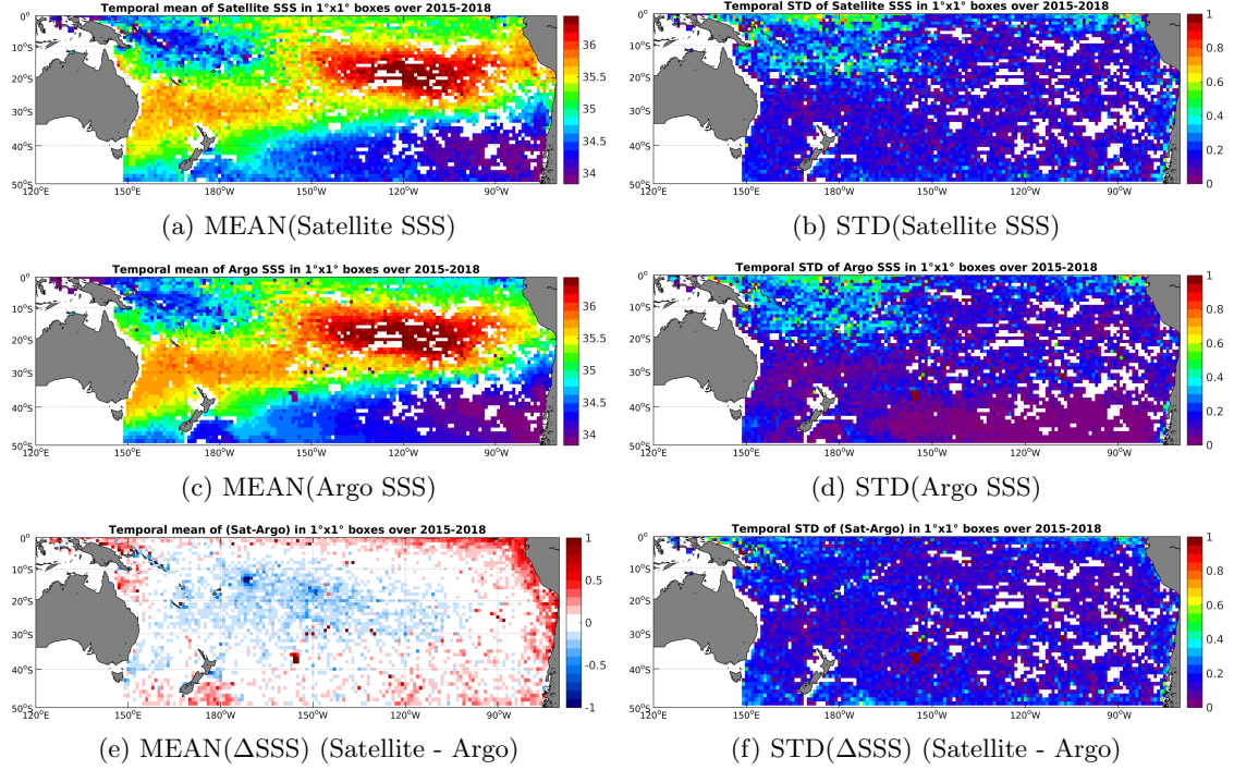
Figure 6: Temporal mean (left) and STD (right) of SSS from SMAP-L3-JPL-V4-MONTHLY-60KM (top), Argo (middle), and of \Delta SSS (Satellite - Argo). Only match-up pairs are used to generate these maps.
