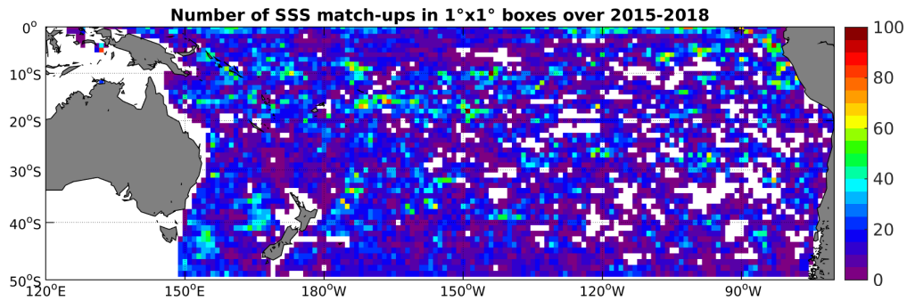
Figure 4: Number of SSS match-ups between Argo SSS and the SMAP-L3-JPL-V4-MONTHLY-60KM SSS product for the South Pacific Ocean Pi-MEP region over 1^\circ \times 1^\circ boxes and for the full satellite product period.
