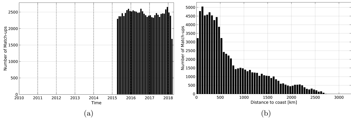
Figure 1: Number of match-ups between Argo and SMAP-L3-JPL-V4-MONTHLY-60KM SSS as a function of time (a) and as function of the distance to coast (b) over the South Pacific Ocean Pi-MEP region and for the full satellite product period.
