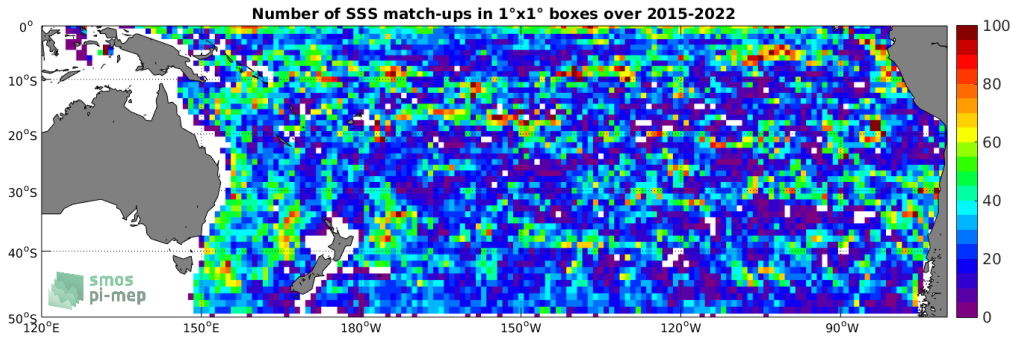
Figure 4: Number of SSS match-ups between Argo SSS and the SMAP SSS L2-AVERAGED v5.0 (JPL) SSS product for the South Pacific Ocean Pi-MEP region over 1^\circ \times 1^\circ boxes and for the full satellite product period.
