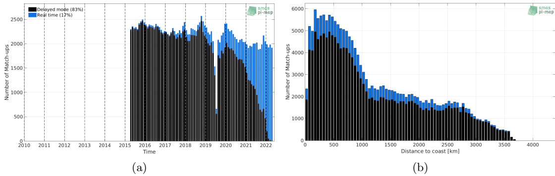
Figure 1: Number of match-ups between Argo and SMAP SSS L2-AVERAGED v5.0 (JPL) SSS as a function of time (a) and as function of the distance to coast (b) over the South Pacific Ocean Pi-MEP region and for the full satellite product period.
