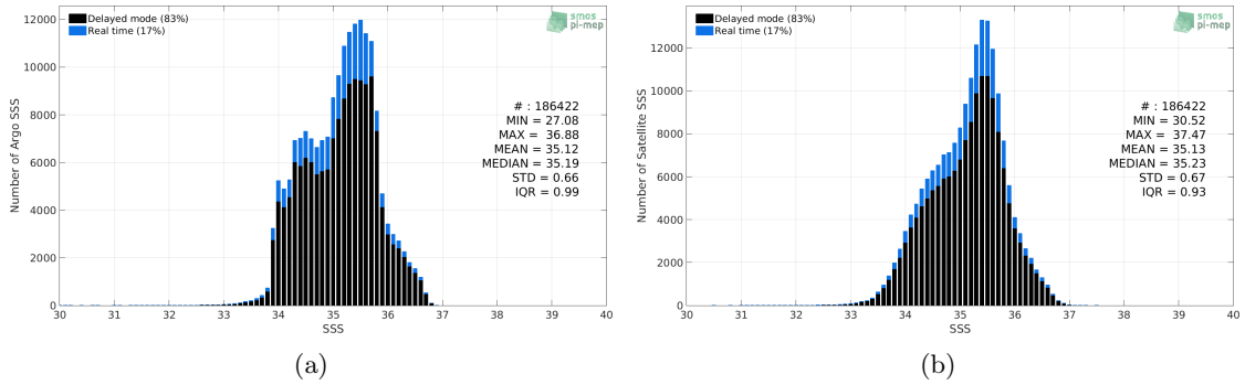
Figure 2: Histograms of SSS from Argo (a) and SMAP SSS L2-AVERAGED v5.0 (JPL) (b) considering all match-up pairs per bins of 0.1 over the South Pacific Ocean Pi-MEP region and for the full satellite product period.
