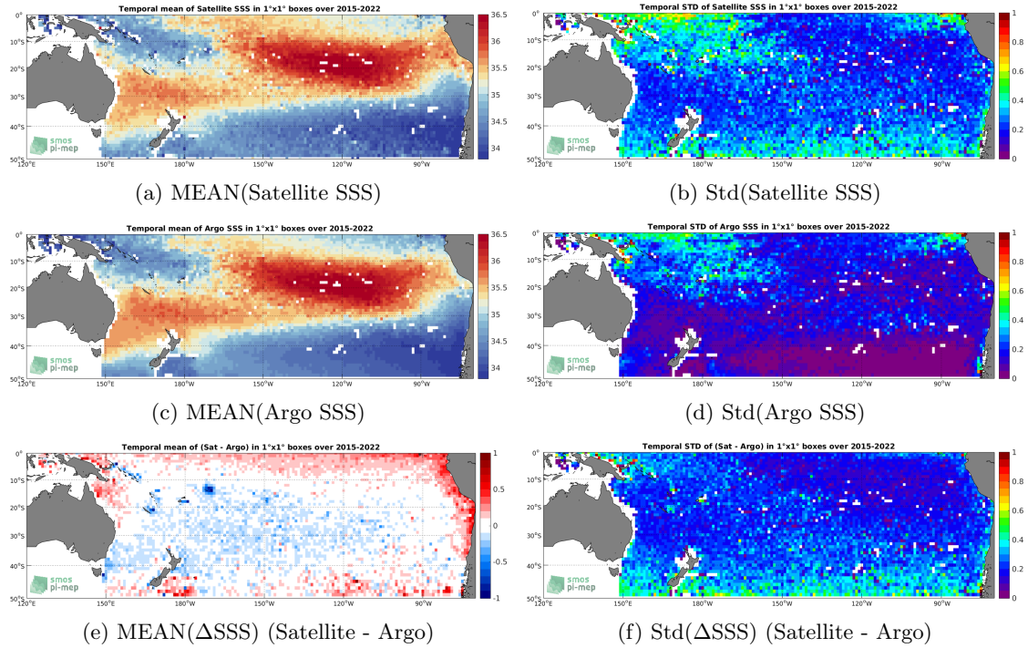
Figure 6: Temporal mean (left) and Std (right) of SSS from SMAP SSS L2-AVERAGED v5.0 (JPL) (top), Argo (middle), and of \Delta SSS (Satellite - Argo). Only match-up pairs are used to generate these maps.
