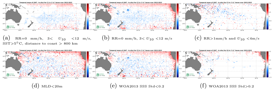
Figure 12: Temporal mean gridded over spatial boxes of size 1^\circ \times 1^\circ of \Delta SSS (SMAP SSS L2-AVERAGED v5.0 (JPL) - Argo) for 6 different subdatasets corresponding to:RR=0 mm/h, 3 < U_{10} < 12 m/s, SST >5^\circ C, distance to coast > 800 km (a), RR=0 mm/h, 3 < U_{10} < 12 m/s (b), RR >1 mm/h and U_{10} < 4 m/s (c),MLD <20 m (d),WOA2013 SSS Std <0.2 (e),WOA2013 SSS Std >0.2 (f).
