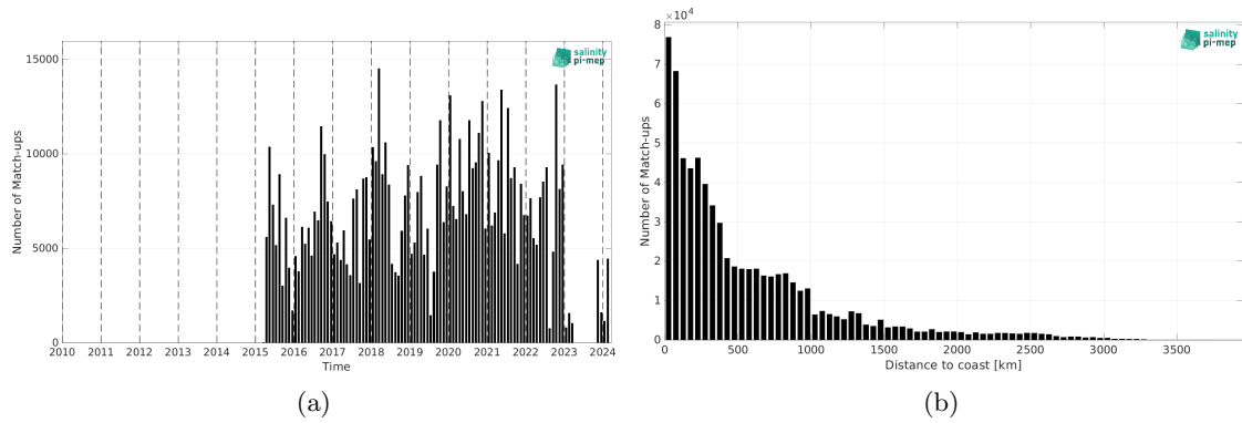
Figure 2: Number of match-ups between TSG (LEGOS-DM) and SMAP SSS L2 v6 (RSS) SSS as a function of time (a) and as function of the distance to coast (b) over the South Pacific Ocean Pi-MEP region and for the full satellite product period.
