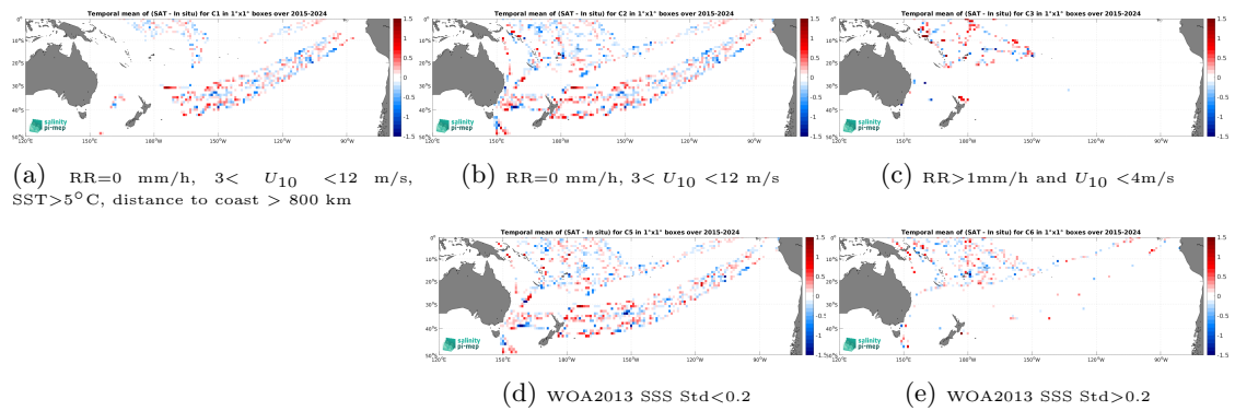
Figure 14: Temporal mean gridded over spatial boxes of size 1^\circ \times 1^\circ of \Delta SSS (SMAP SSS L2 v6 (RSS) - TSG (LEGOS-DM)) for 5 different subdatasets corresponding to:RR=0 mm/h, 3 < U_{10} < 12 m/s, SST>5°C, distance to coast > 800 km (a), RR=0 mm/h, 3 < U_{10} < 12 m/s (b), RR>1mm/h and U_{10} < 4 m/s (c), WOA2013 SSS Std<0.2 (d), WOA2013 SSS Std>0.2 (e).
