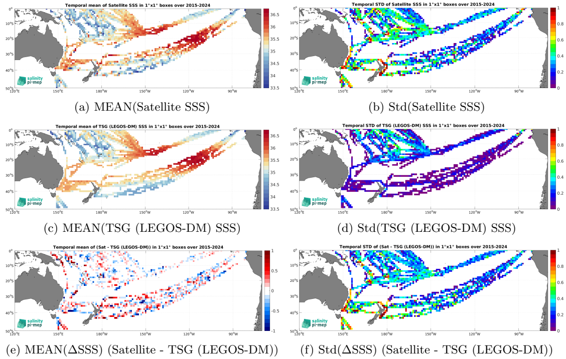
Figure 7: Temporal mean (left) and Std (right) of SSS from SMAP SSS L2 v6 (RSS) (top), TSG (LEGOS-DM) (middle), and of \Delta SSS (Satellite - TSG (LEGOS-DM)). Only match-up pairs are used to generate these maps.
