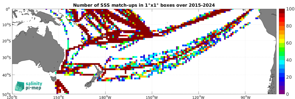
Figure 5: Number of SSS match-ups between TSG (LEGOS-DM) SSS and the SMAP SSS L2 v6 (RSS) SSS product for the South Pacific Ocean Pi-MEP region over 1^\circ \times 1^\circ boxes and for the full satellite product period.
