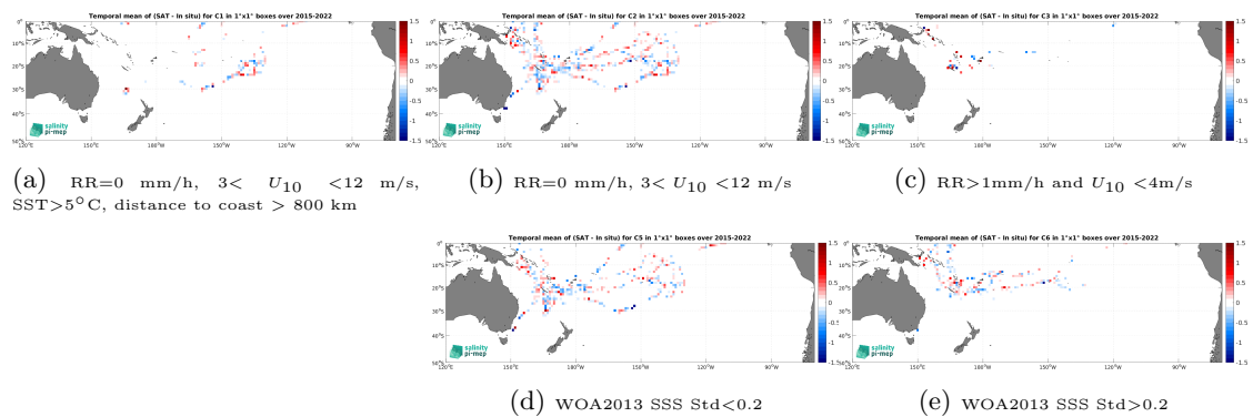
Figure 14: Temporal mean gridded over spatial boxes of size 1^\circ \times 1^\circ of \Delta SSS (SMAP SSS L2 v6 (RSS) - TSG (GOSUD-Research-vessel)) for 5 different subdatasets corresponding to:RR=0 mm/h, 3 < U_{10} < 12 m/s, SST >5^\circ\text{C} , distance to coast > 800 km (a), RR=0 mm/h, 3 < U_{10} < 12 m/s (b), RR >1 mm/h and U_{10} < 4 m/s (c), WOA2013 SSS Std <0.2 (d), WOA2013 SSS Std >0.2 (e).
