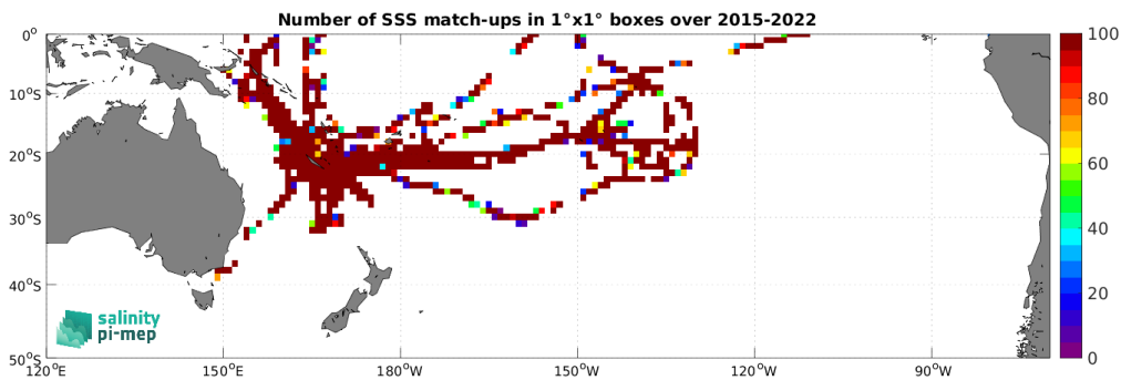
Figure 5: Number of SSS match-ups between TSG (GOSUD-Research-vessel) SSS and the SMAP SSS L2 v6 (RSS) SSS product for the South Pacific Ocean Pi-MEP region over 1^\circ \times 1^\circ boxes and for the full satellite product period.
