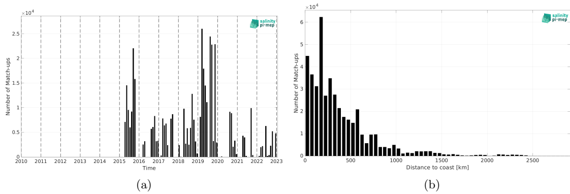
Figure 2: Number of match-ups between TSG (GOSUD-Research-vessel) and SMAP SSS L2 v6 (RSS) SSS as a function of time (a) and as function of the distance to coast (b) over the South Pacific Ocean Pi-MEP region and for the full satellite product period.
