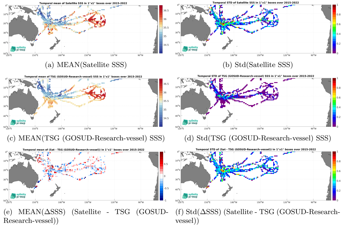
Figure 7: Temporal mean (left) and Std (right) of SSS from SMAP SSS L2 v6 (RSS) (top), TSG (GOSUD-Research-vessel) (middle), and of \Delta SSS (Satellite - TSG (GOSUD-Research-vessel)). Only match-up pairs are used to generate these maps.
