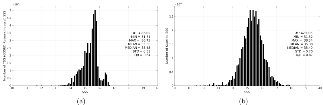
Figure 3: Histograms of SSS from TSG (GOSUD-Research-vessel) (a) and SMAP SSS L2 v6 (RSS) (b) considering all match-up pairs per bins of 0.1 over the South Pacific Ocean Pi-MEP region and for the full satellite product period.
