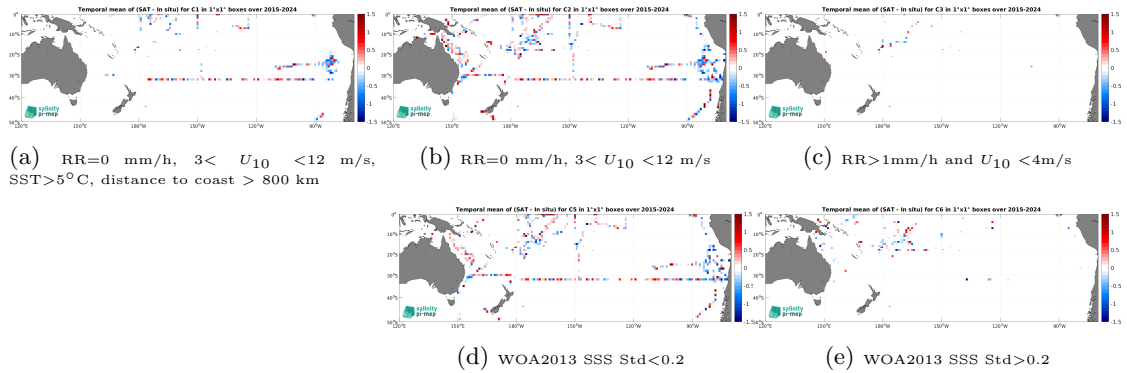
Figure 14: Temporal mean gridded over spatial boxes of size 1^\circ \times 1^\circ of \Delta SSS (SMAP SSS L2 v6 - 40 km (RSS) - TSG (SAMOS)) for 5 different subdatasets corresponding to:RR=0 mm/h, 3 < U_{10} < 12 m/s, SST>5°C, distance to coast > 800 km (a), RR=0 mm/h, 3 < U_{10} < 12 m/s (b), RR>1mm/h and U_{10} < 4 m/s (c), WOA2013 SSS Std<0.2 (d), WOA2013 SSS Std>0.2 (e).
