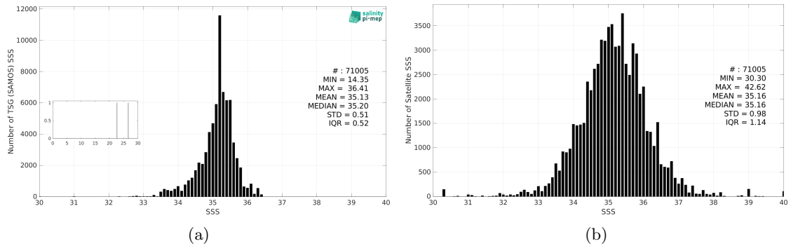
Figure 3: Histograms of SSS from TSG (SAMOS) (a) and SMAP SSS L2 v6 - 40 km (RSS) (b) considering all match-up pairs per bins of 0.1 over the South Pacific Ocean Pi-MEP region and for the full satellite product period.
