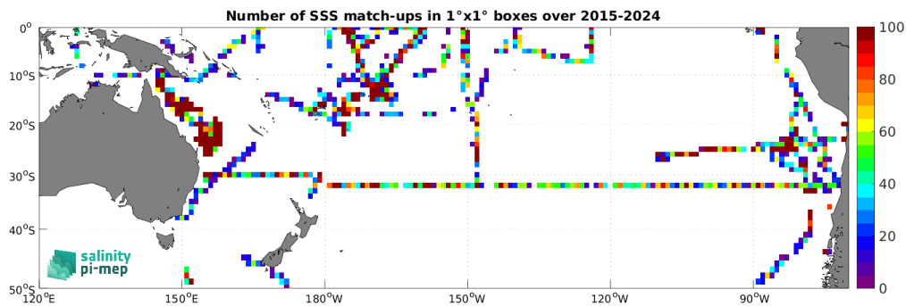
Figure 5: Number of SSS match-ups between TSG (SAMOS) SSS and the SMAP SSS L2 v6 - 40 km (RSS) SSS product for the South Pacific Ocean Pi-MEP region over 1^\circ \times 1^\circ boxes and for the full satellite product period.
