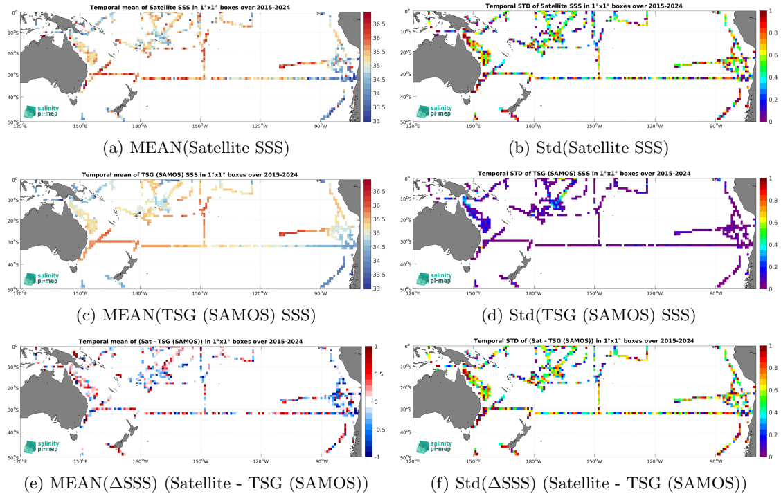
Figure 7: Temporal mean (left) and Std (right) of SSS from SMAP SSS L2 v6 - 40 km (RSS) (top), TSG (SAMOS) (middle), and of \Delta SSS (Satellite - TSG (SAMOS)). Only match-up pairs are used to generate these maps.
