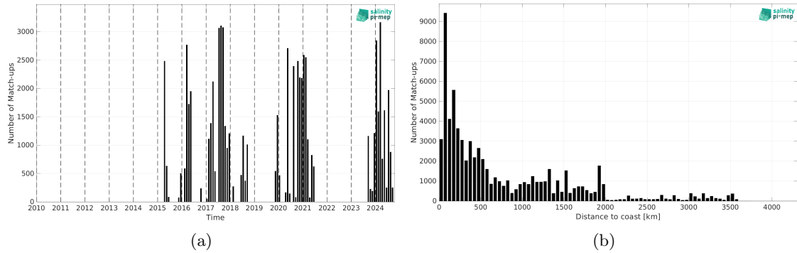
Figure 2: Number of match-ups between TSG (SAMOS) and SMAP SSS L2 v6 - 40 km (RSS) SSS as a function of time (a) and as function of the distance to coast (b) over the South Pacific Ocean Pi-MEP region and for the full satellite product period.
