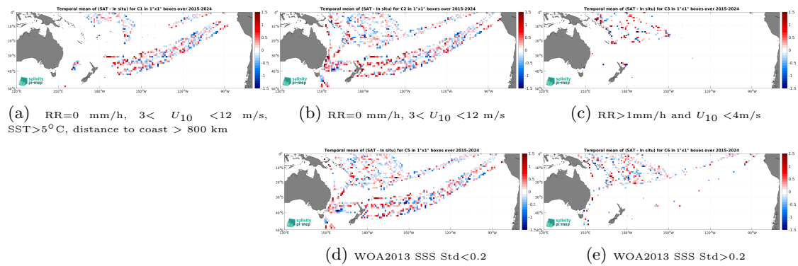
Figure 14: Temporal mean gridded over spatial boxes of size 1^\circ \times 1^\circ of \Delta\text{SSS} (SMAP SSS L2 v6 - 40 km (RSS) - TSG (LEGOS-DM)) for 5 different subdatasets corresponding to:RR=0 mm/h, 3 < U_{10} < 12 m/s, SST>5°C, distance to coast > 800 km (a), RR=0 mm/h, 3 < U_{10} < 12 m/s (b), RR>1mm/h and U_{10} < 4 m/s (c), WOA2013 SSS Std<0.2 (d), WOA2013 SSS Std>0.2 (e).
