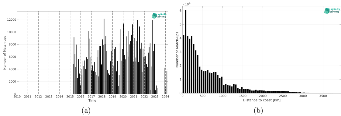
Figure 2: Number of match-ups between TSG (LEGOS-DM) and SMAP SSS L2 v6 - 40 km (RSS) SSS as a function of time (a) and as function of the distance to coast (b) over the South Pacific Ocean Pi-MEP region and for the full satellite product period.
