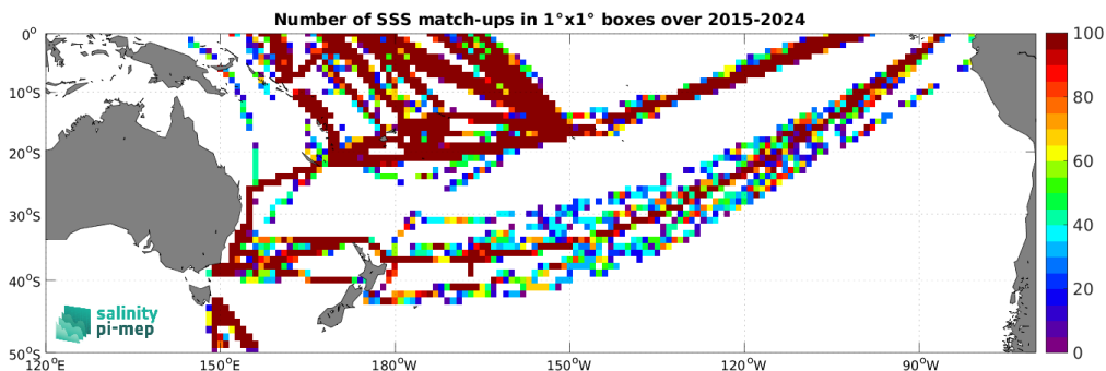
Figure 5: Number of SSS match-ups between TSG (LEGOS-DM) SSS and the SMAP SSS L2 v6 - 40 km (RSS) SSS product for the South Pacific Ocean Pi-MEP region over 1^\circ \times 1^\circ boxes and for the full satellite product period.
