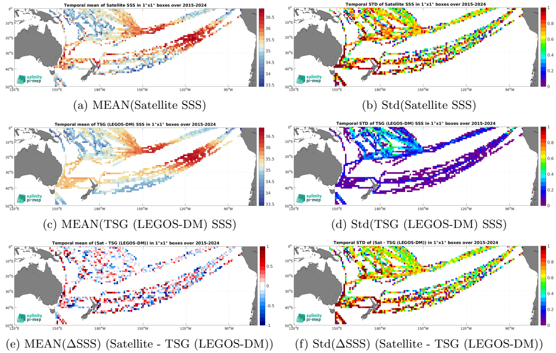
Figure 7: Temporal mean (left) and Std (right) of SSS from SMAP SSS L2 v6 - 40 km (RSS) (top), TSG (LEGOS-DM) (middle), and of \Delta SSS (Satellite - TSG (LEGOS-DM)). Only match-up pairs are used to generate these maps.
