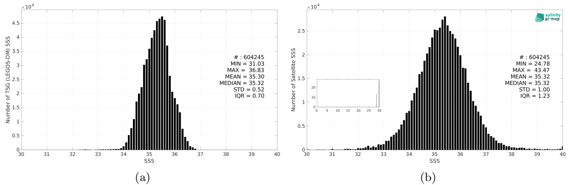
Figure 3: Histograms of SSS from TSG (LEGOS-DM) (a) and SMAP SSS L2 v6 - 40 km (RSS) (b) considering all match-up pairs per bins of 0.1 over the South Pacific Ocean Pi-MEP region and for the full satellite product period.
