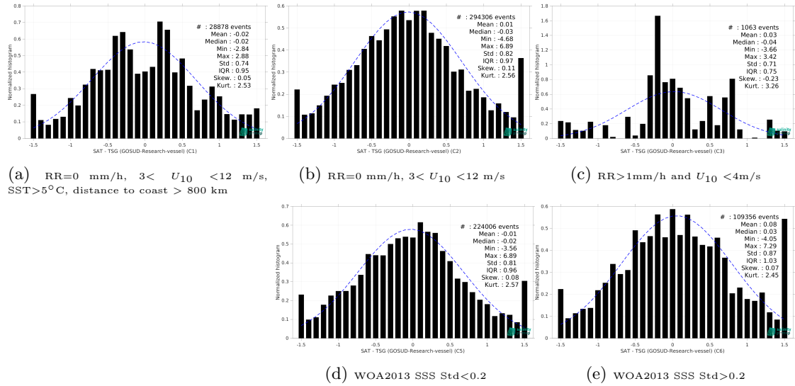
Figure 15: Normalized histogram of \Delta SSS (SMAP SSS L2 v6 - 40 km (RSS) - TSG (GOSUD-Research-vessel)) for 5 different subdatasets corresponding to: RR=0 mm/h, 3 < U_{10} < 12 m/s, SST>5°C, distance to coast > 800 km (a), RR=0 mm/h, 3 < U_{10} < 12 m/s (b), RR>1mm/h and U_{10} < 4 m/s (c), WOA2013 SSS Std<0.2 (d), WOA2013 SSS Std>0.2 (e).
