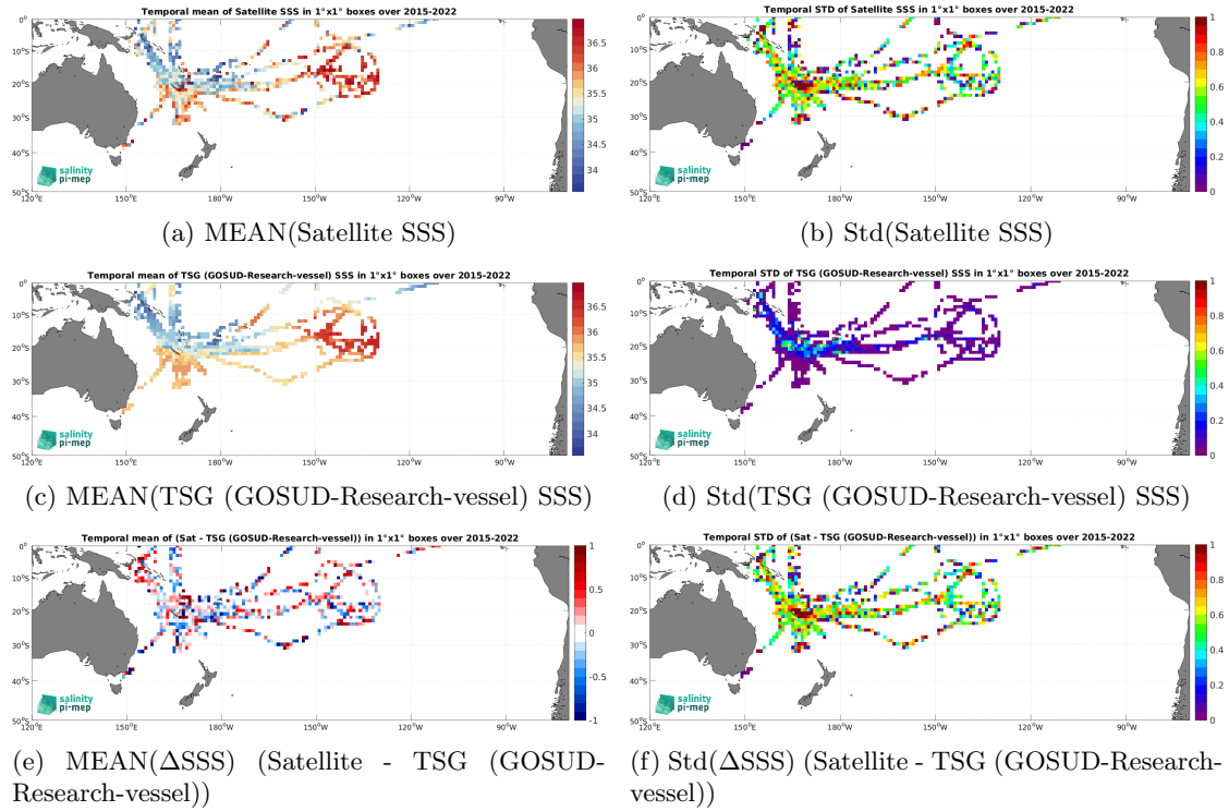
Figure 7: Temporal mean (left) and Std (right) of SSS from SMAP SSS L2 v6 - 40 km (RSS) (top), TSG (GOSUD-Research-vessel) (middle), and of \Delta SSS (Satellite - TSG (GOSUD-Research-vessel)). Only match-up pairs are used to generate these maps.
