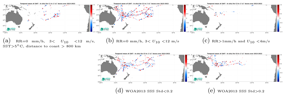
Figure 14: Temporal mean gridded over spatial boxes of size 1^\circ \times 1^\circ of \Delta SSS (SMAP SSS L2 v6 - 40 km (RSS) - TSG (GOSUD-Research-vessel)) for 5 different subdatasets corresponding to:RR=0 mm/h, 3 < U_{10} < 12 m/s, SST >5^\circ\text{C} , distance to coast > 800 km (a), RR=0 mm/h, 3 < U_{10} < 12 m/s (b), RR >1 mm/h and U_{10} < 4 m/s (c), WOA2013 SSS Std <0.2 (d), WOA2013 SSS Std >0.2 (e).
