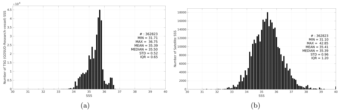
Figure 3: Histograms of SSS from TSG (GOSUD-Research-vessel) (a) and SMAP SSS L2 v6 - 40 km (RSS) (b) considering all match-up pairs per bins of 0.1 over the South Pacific Ocean Pi-MEP region and for the full satellite product period.
