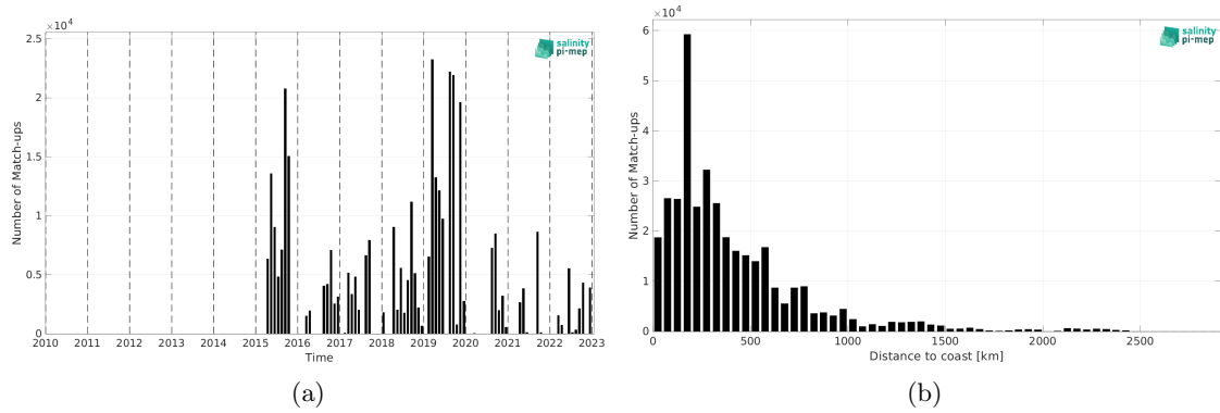
Figure 2: Number of match-ups between TSG (GOSUD-Research-vessel) and SMAP SSS L2 v6 - 40 km (RSS) SSS as a function of time (a) and as function of the distance to coast (b) over the South Pacific Ocean Pi-MEP region and for the full satellite product period.
