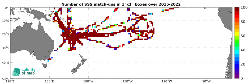
Figure 5: Number of SSS match-ups between TSG (GOSUD-Research-vessel) SSS and the SMAP SSS L2 v6 - 40 km (RSS) SSS product for the South Pacific Ocean Pi-MEP region over 1^\circ \times 1^\circ boxes and for the full satellite product period.
